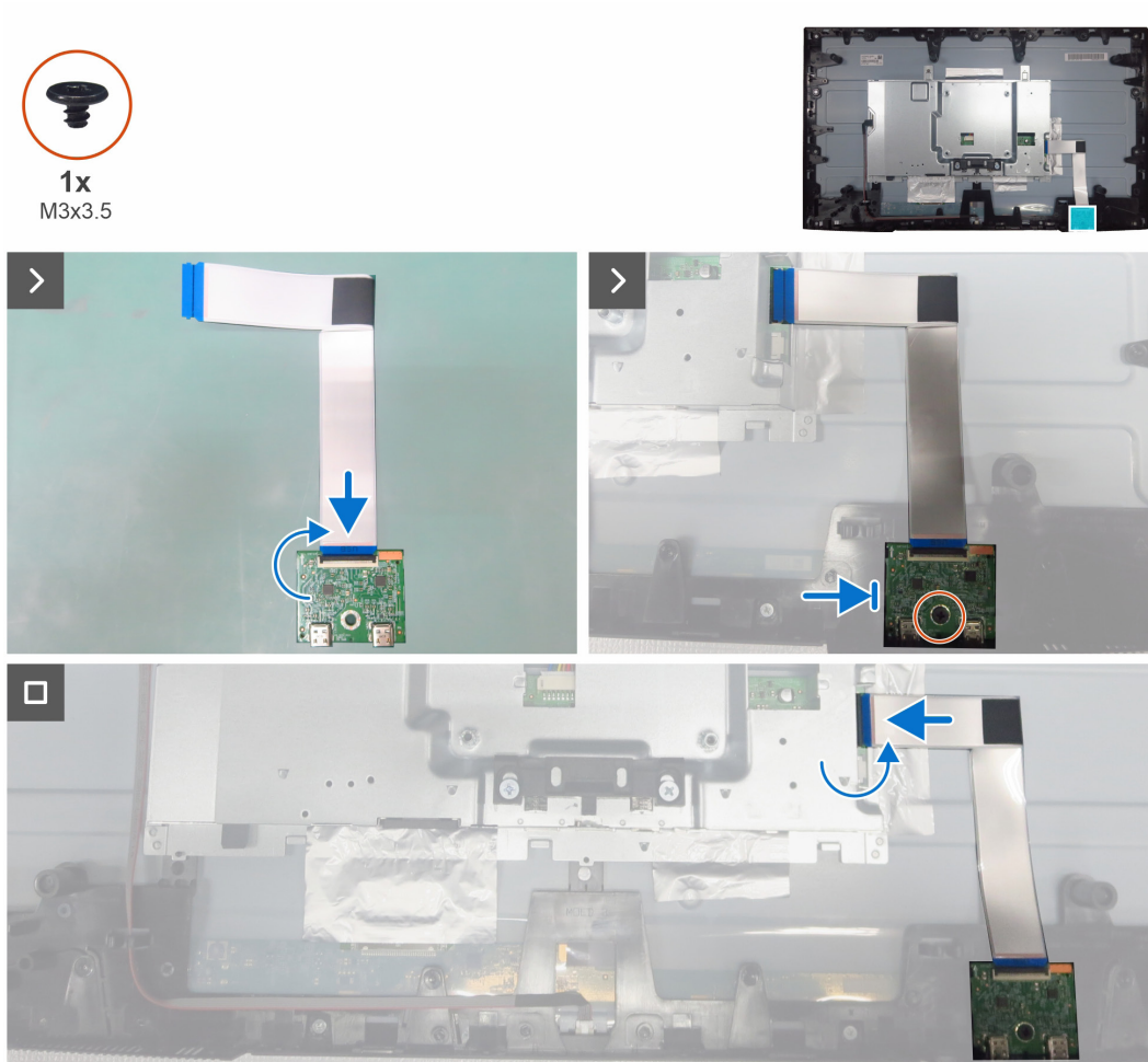
Figure 10. Installing the USB board
