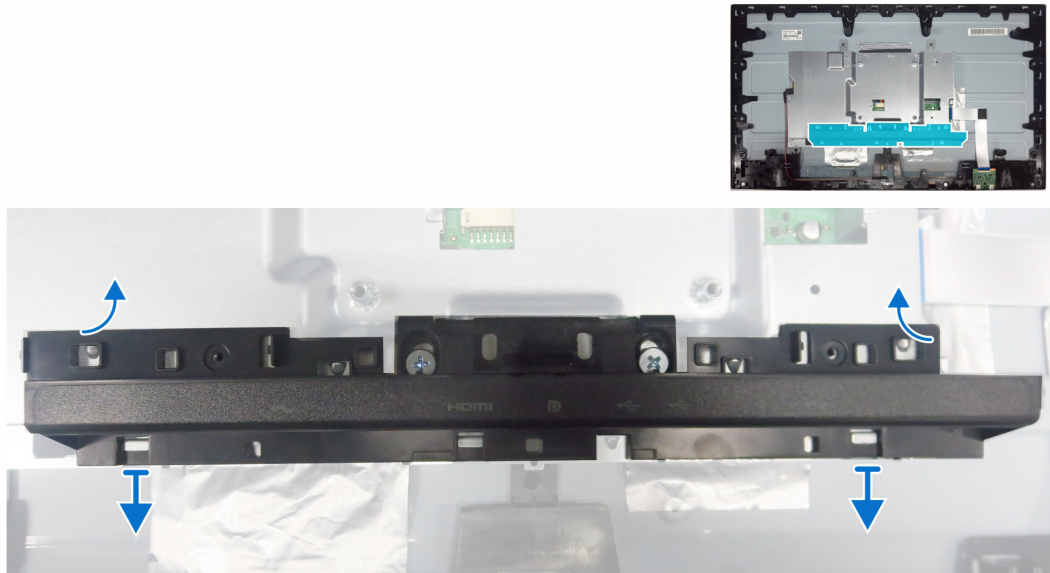
Figure 7. Removing the I/O cover
