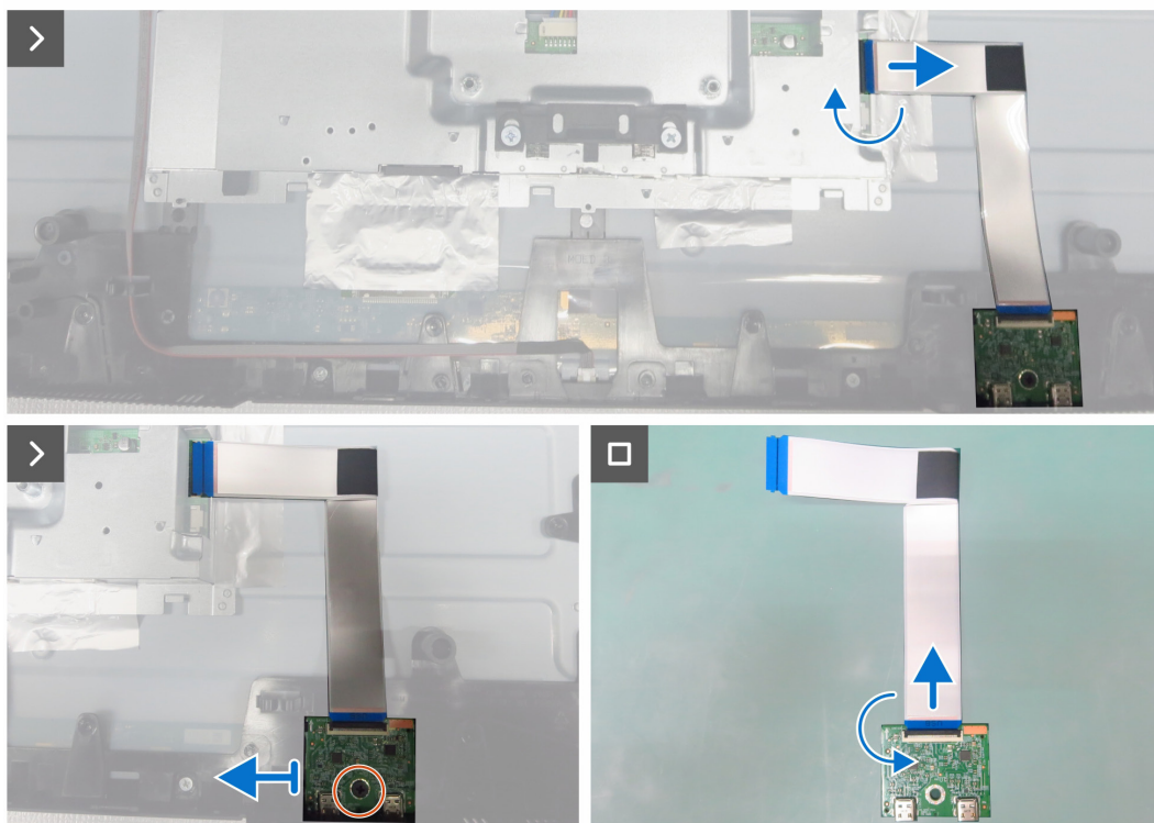
Figure 9. Removing the USB board
