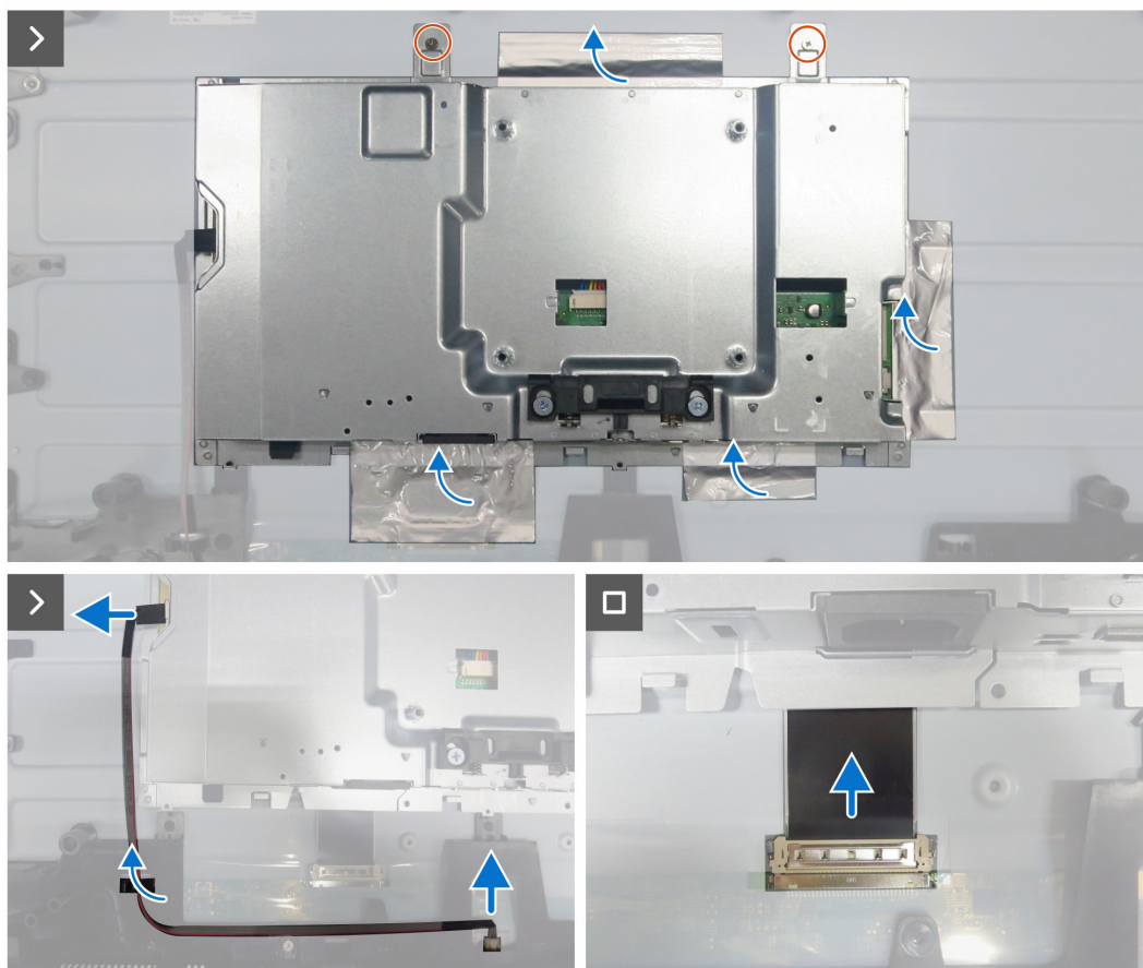
Figure 11. Removing the main chassis
