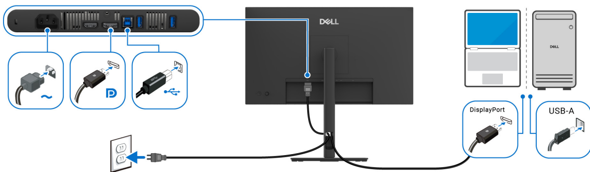
Figure 30. DisplayPort connection
