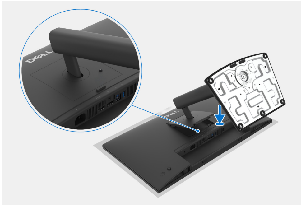
Figure 12. Installer le pied
