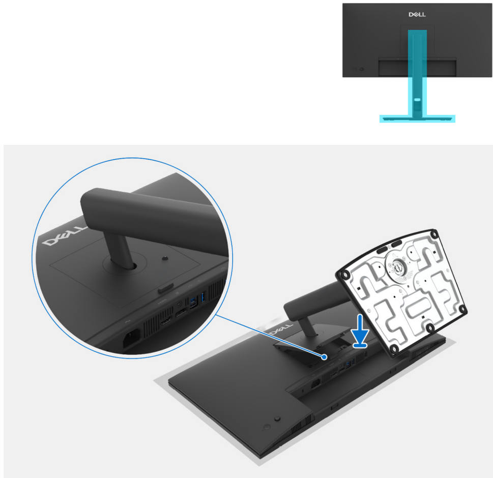
Figure 2. Installer le pied
