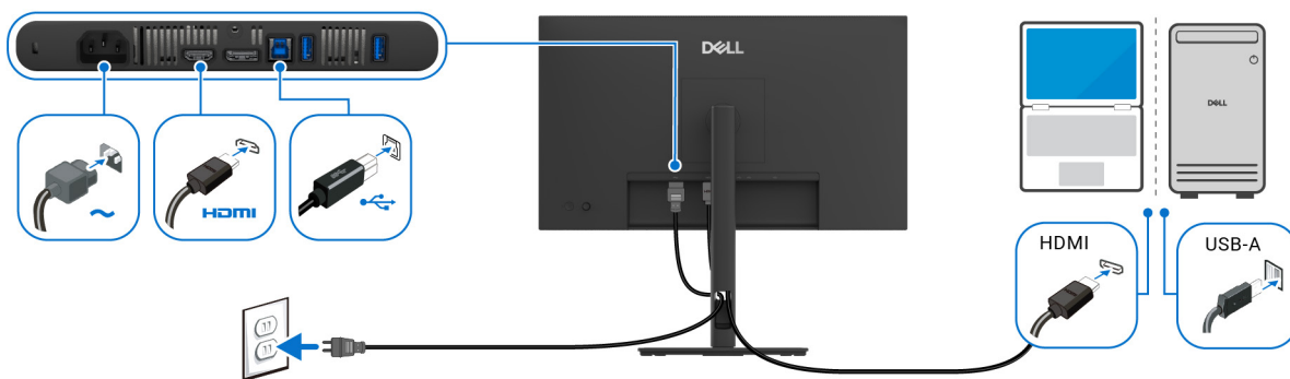
Figure 10. Connexion HDMI
