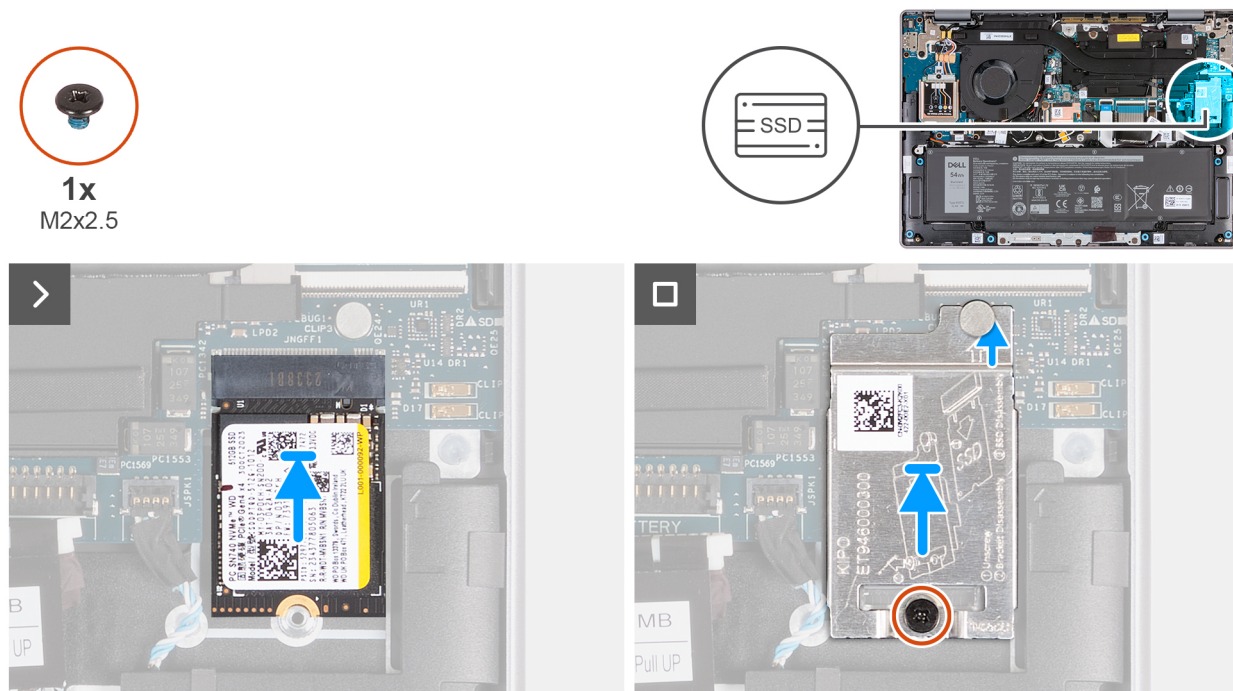
Figure 24. Installation du SSD
