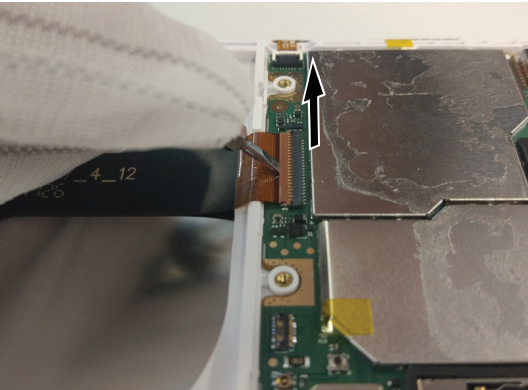
Figure 4. Removal steps of main FPC (continued)
