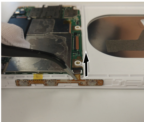
Figure 6. Removal steps of sidekey (continued)
