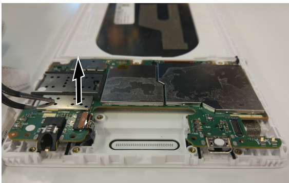
Figure 8. Removal steps of main board (continued)
