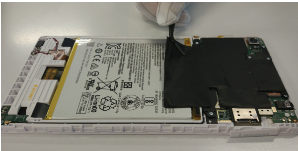
Figure 2. Removal steps of battery
