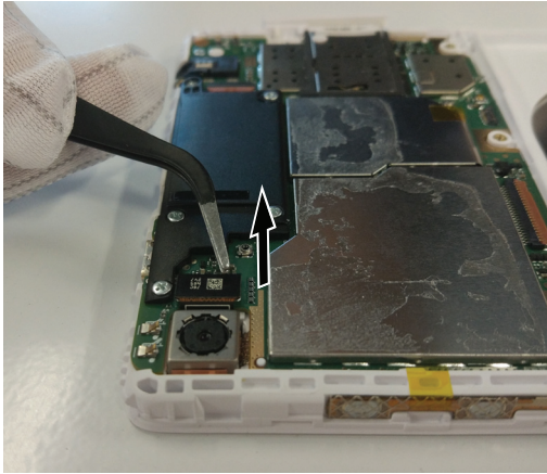
Figure 5. Removal steps of rear camera
