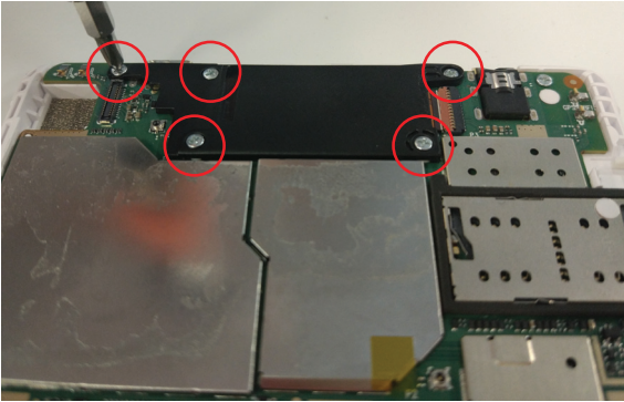
Figure 7. Removal steps of speaker box
