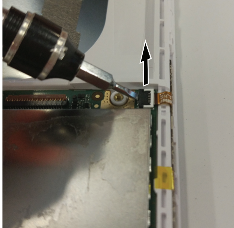
Figure 6. Removal steps of sidekey
