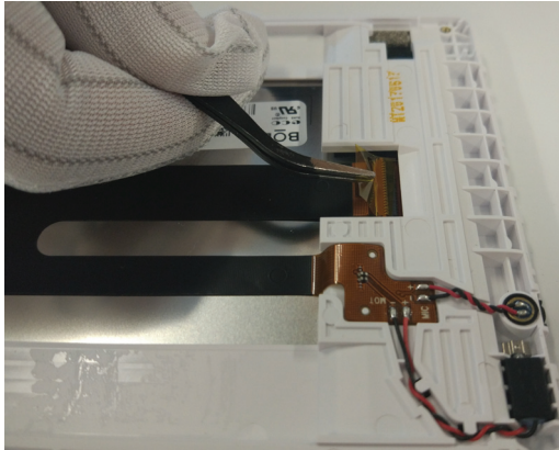
Figure 4. Removal steps of main FPC
