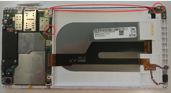
Figure 3. Removal steps of sub board Disconnect the ends of the RF cable and remove the RF cable from the routing groove.
