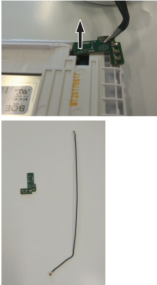
Figure 3. Removal steps of sub board (continued)
