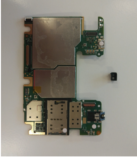
Figure 8. Removal steps of main board (continued)
