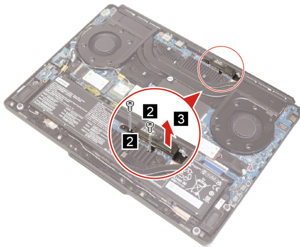
Figure 18. Remove two screws and the DC-in bracket
