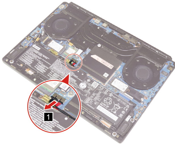
Figure 17. Disconnect the battery pack cable
