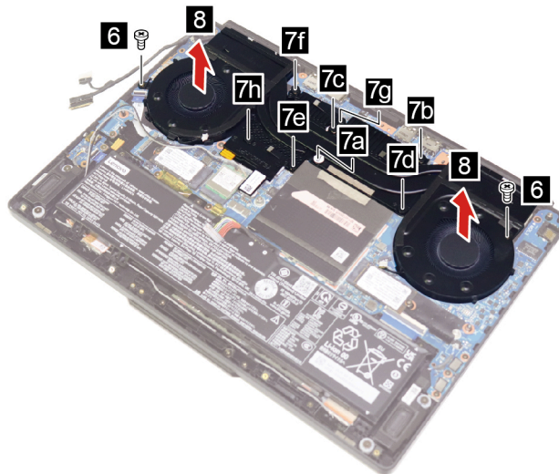
Figure 21. Remove two screws, loosen eight screws, and remove the thermal module
