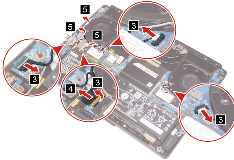
Figure 20. Disconnect the fan cables and EDP cable, and remove the antennas
