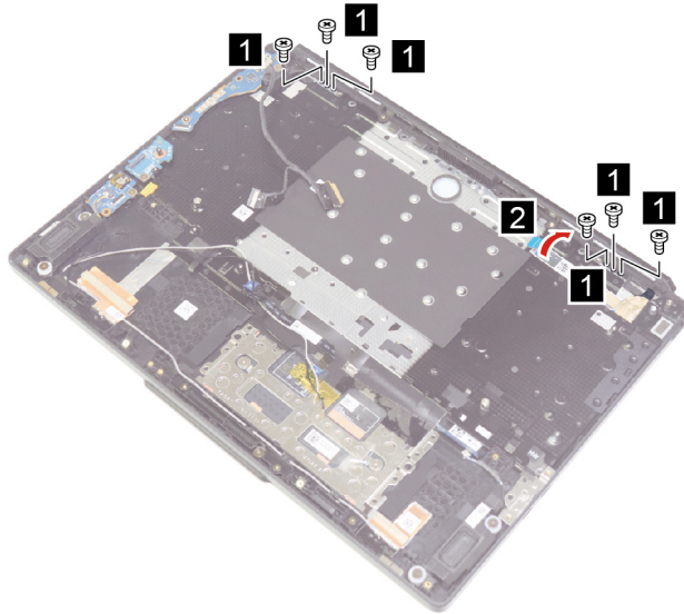
Figure 33. Remove six screws and lift the camera cable
