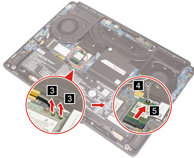
Figure 8. Disconnect the antennas and remove one screw and the Wi-Fi card
