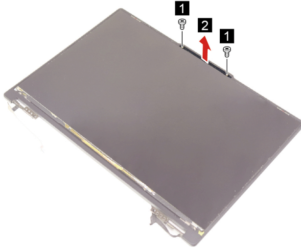
Figure 36. Remove two screws and the camera bracket
