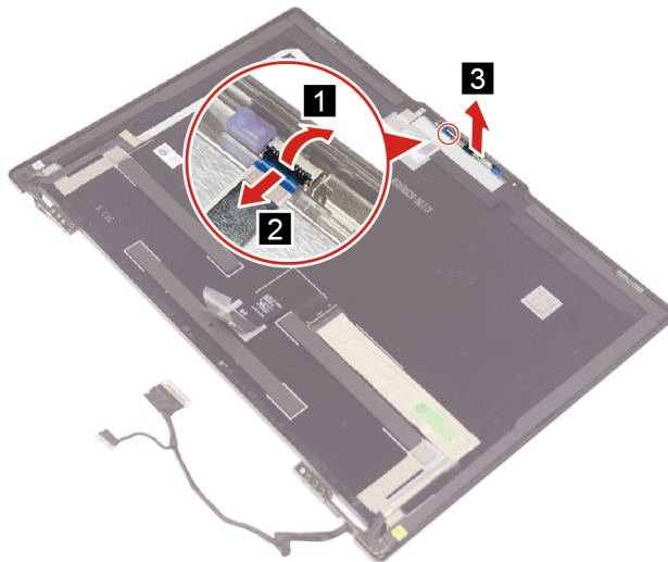
Figure 42. Disconnect the camera cable and remove the camera board
