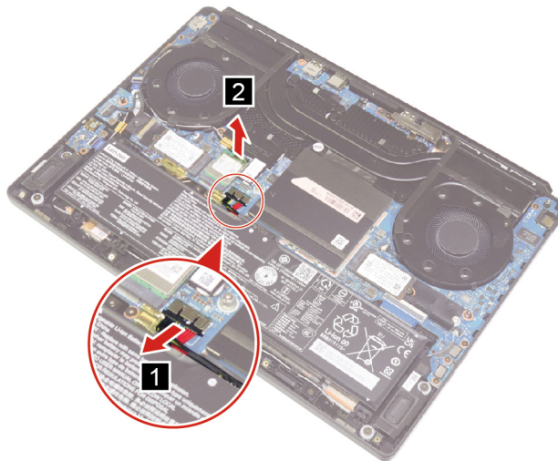
Figure 7. Disconnect the battery pack cable and remove the mylar
