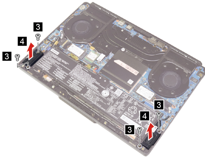
Figure 12. Remove four screws and speakers
