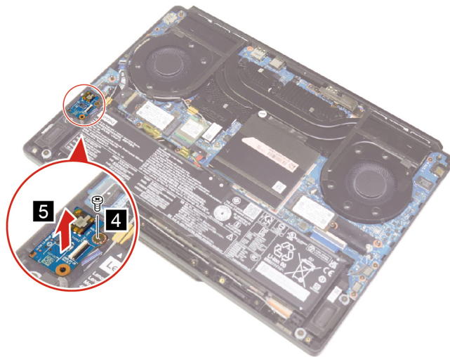
Figure 14. Remove one screw and the audio board
