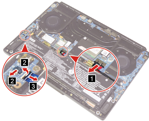
Figure 13. Disconnect the battery pack cable, the audio board cable, and the speaker cable
