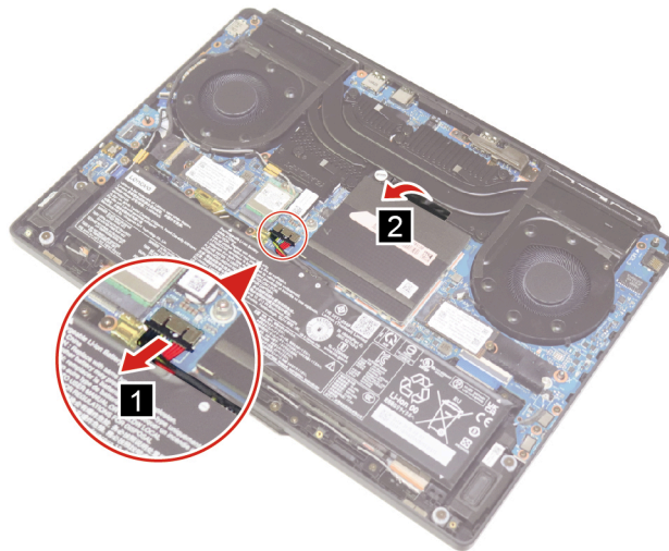
Figure 19. Disconnect the battery pack cable and peel back the mylar
