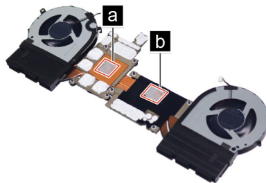
Figure 22. Areas on the thermal module where thermal interface materials should be applied (for AMD models)
