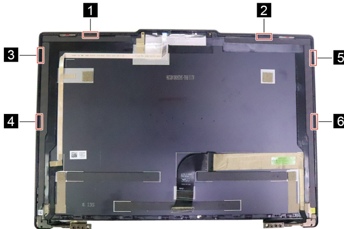
Figure 41. The locations where the rubber pads should be inserted
