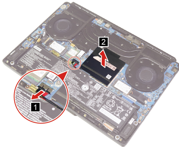
Figure 9. Disconnect the battery pack cable and remove the memory module shielding
