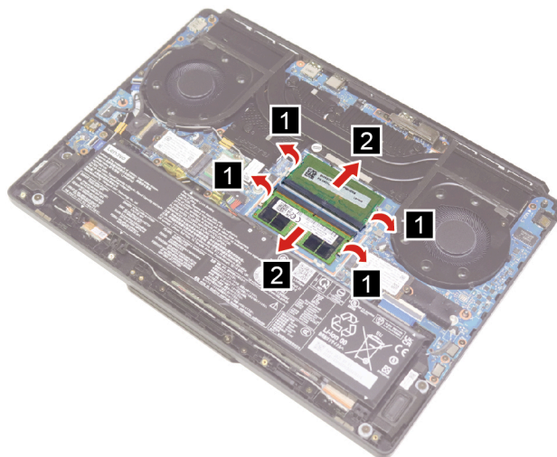
Figure 10. Open the latches and remove the memory module
