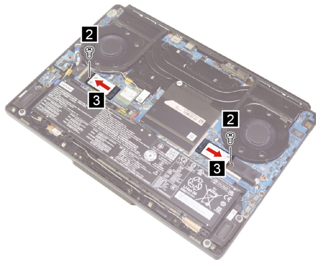
Figure 6. Remove two screws and the solid-state drives
