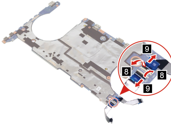
Figure 30. Disconnect and remove the USB board cable and audio board cable
