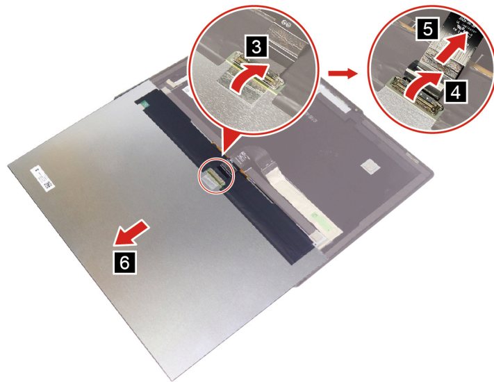
Figure 39. Disconnect the EDP cable and remove the LCD/OLED panel
