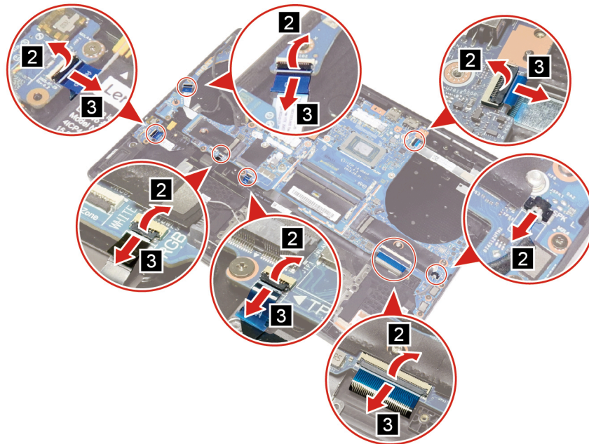
Figure 28. Disconnect the USB board cable, audio board cable, keyboard backlight cable, touchpad cable, keyboard cable, speaker cable, and camera cable
