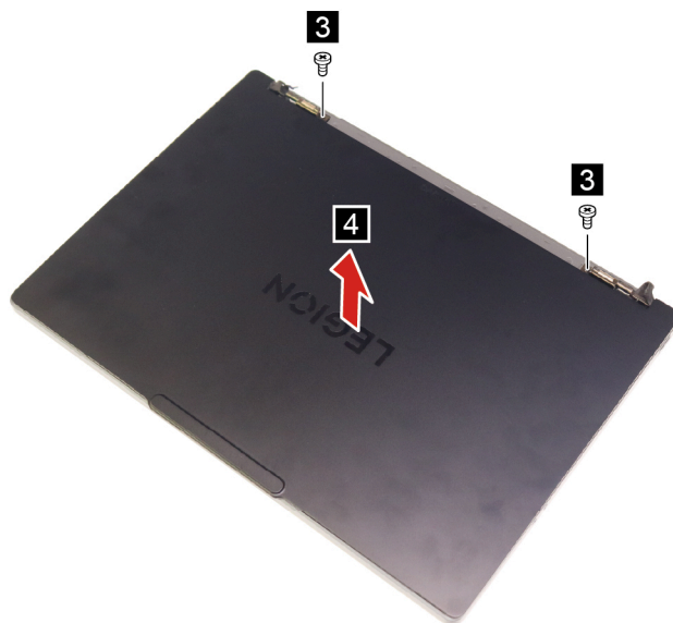
Figure 34. Remove the LCD/OLED module
