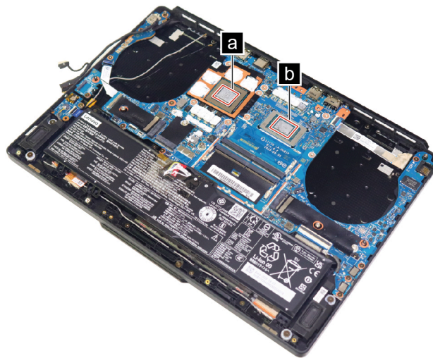
Figure 24. Areas on the system board where thermal interface materials are applied (for AMD models)
