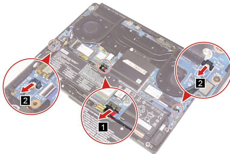
Figure 11. Disconnect the battery pack cable and speaker cables
