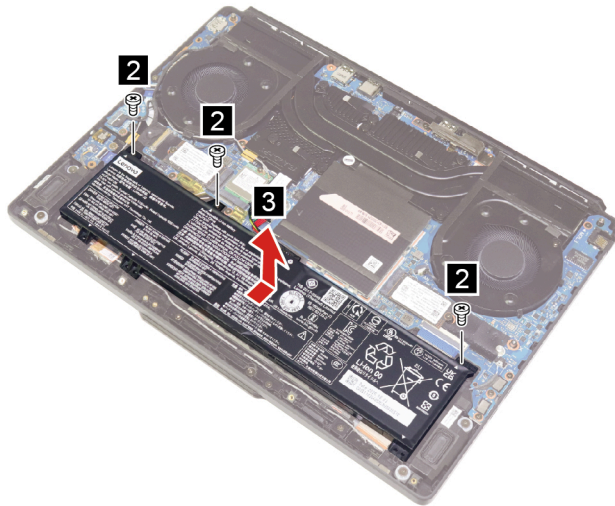
Figure 4. Remove three screws and the battery pack
