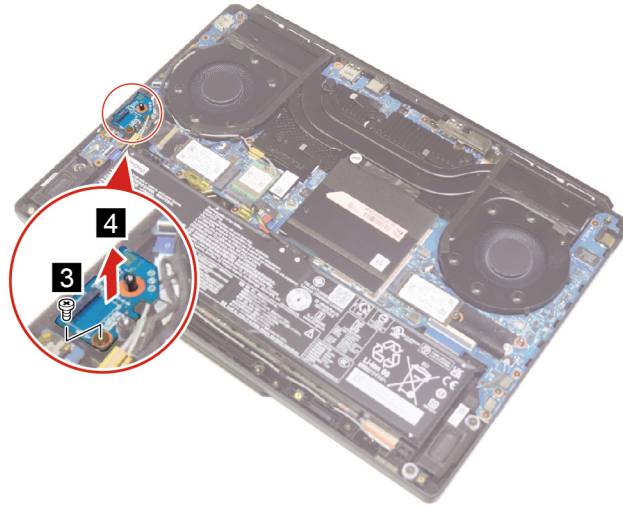
Figure 16. Remove one screw and the PMIC board
