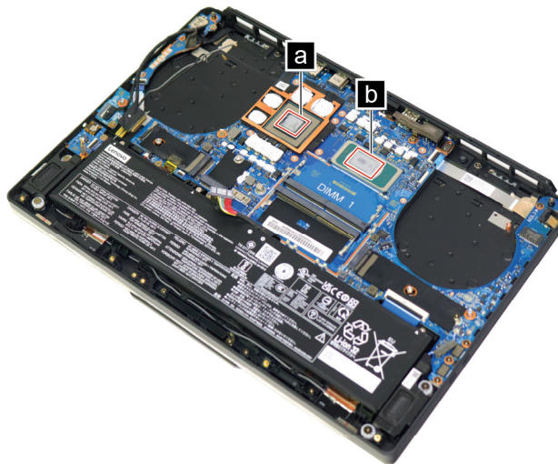
Figure 25. Areas on the system board where thermal interface materials are applied (for Intel models)
