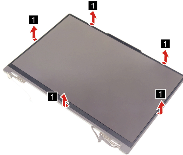
Figure 35. Remove the LCD/OLED bezel
