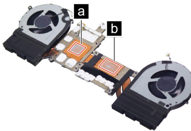
Figure 23. Areas on the thermal module where thermal interface materials should be applied (for Intel models)
