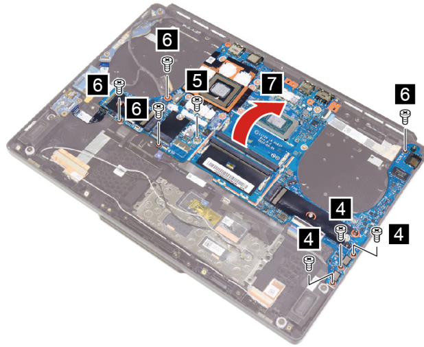
Figure 29. Remove eight screws and the system board
