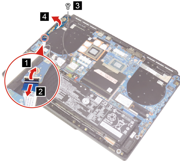
Figure 26. Disconnect the USB board cable and remove one screw and the USB board
