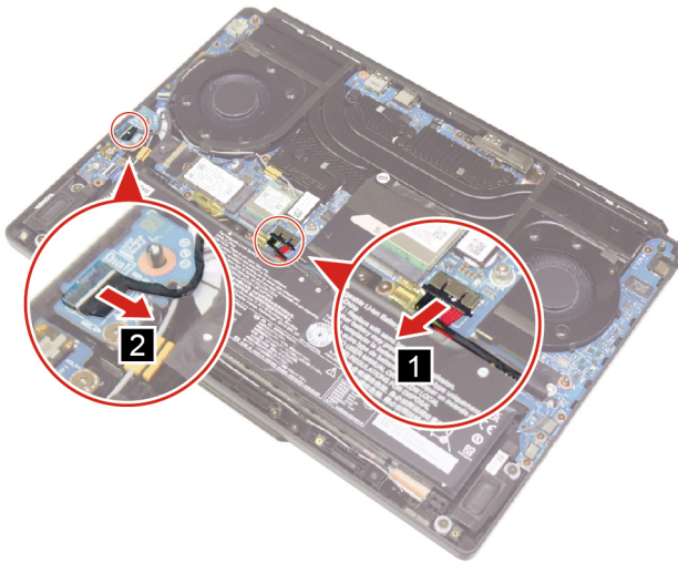
Figure 15. Disconnect the battery pack cable and EDP cable
