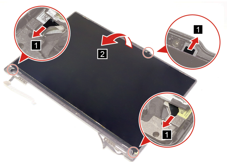
Figure 38. Detach three pieces of stretch-release tape and turn over the LCD/OLED panel
