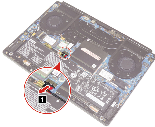
Figure 5. Disconnect the battery pack cable
