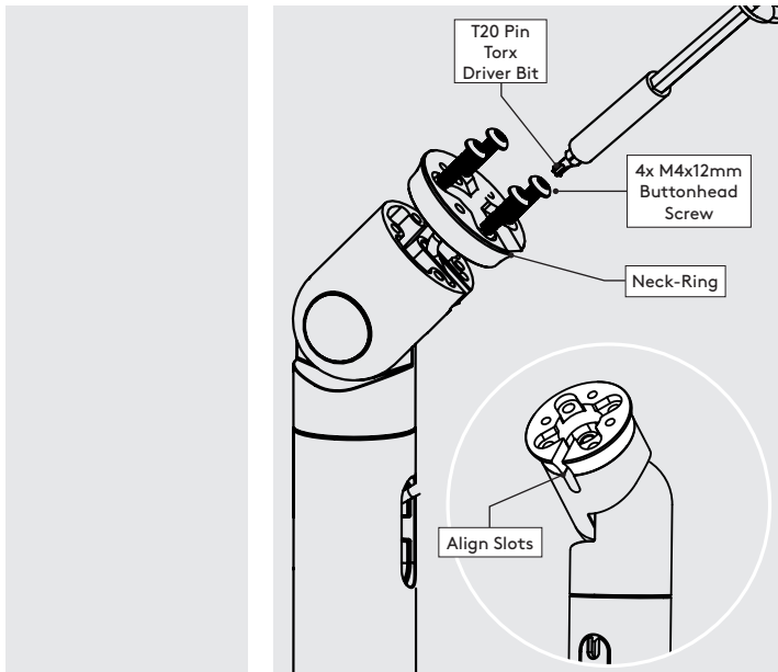
B7 Go to step 1. 1 Attach Neck-Ring to the Twist with 4x M4x12 Buttonhead Screws as shown. The slots must be aligned.
