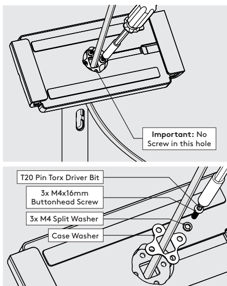
4 Attach the Clip Mount to the Neck-Ring as shown.
