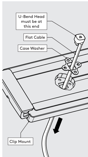
2 Feed the Flat Cable through the Case Washer & Clip Mount as shown.
