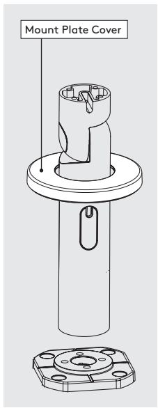
B3 Locate the Cover onto the Twist.
