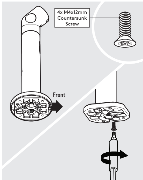
B4 Join the Twist & Mount Plate in the orientation shown.
