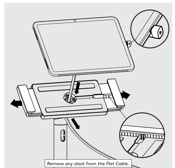
6 Open the Clip Mount Jaws & Lower the Tablet
