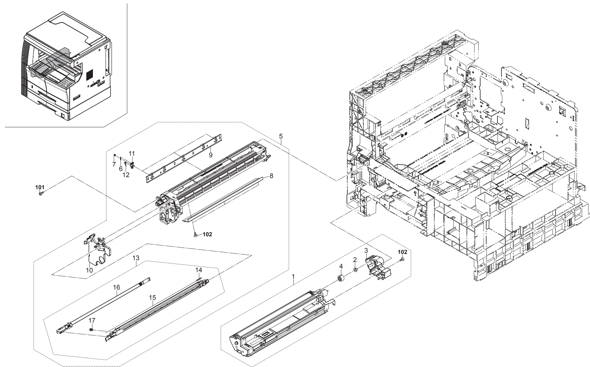
FIG. 11 Imaging Unit
