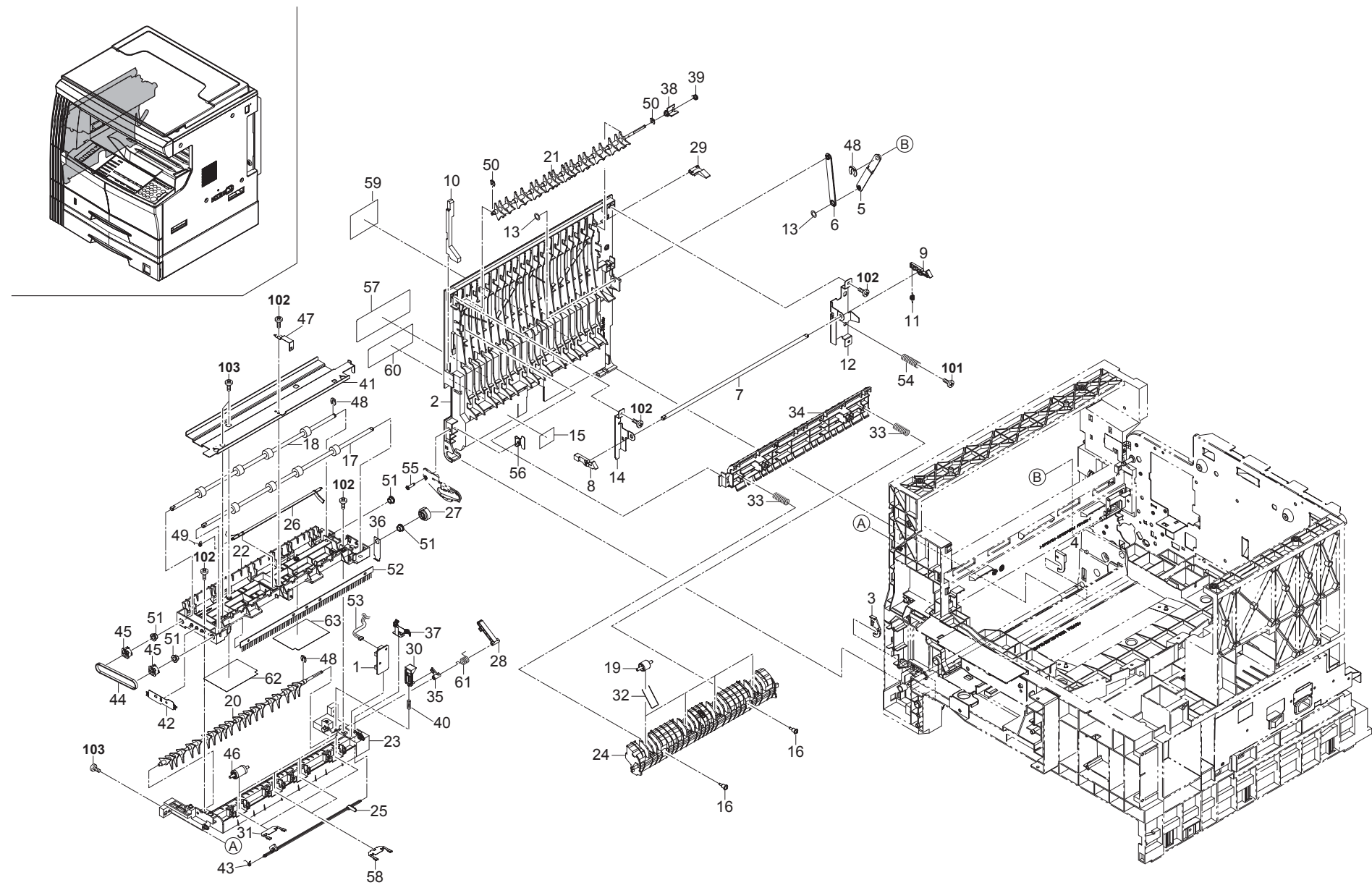
FIG. 9 Exit Section
