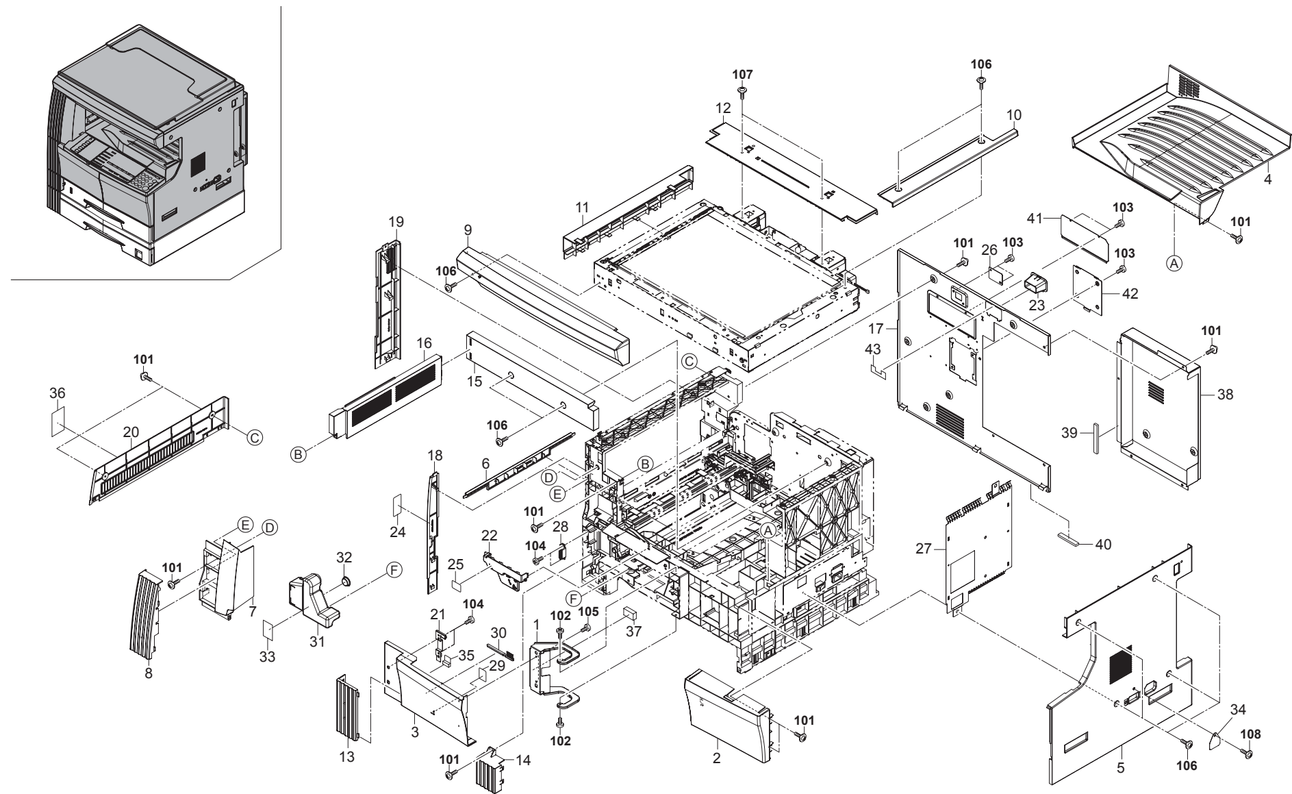
FIG. 1 Exterior Covers
