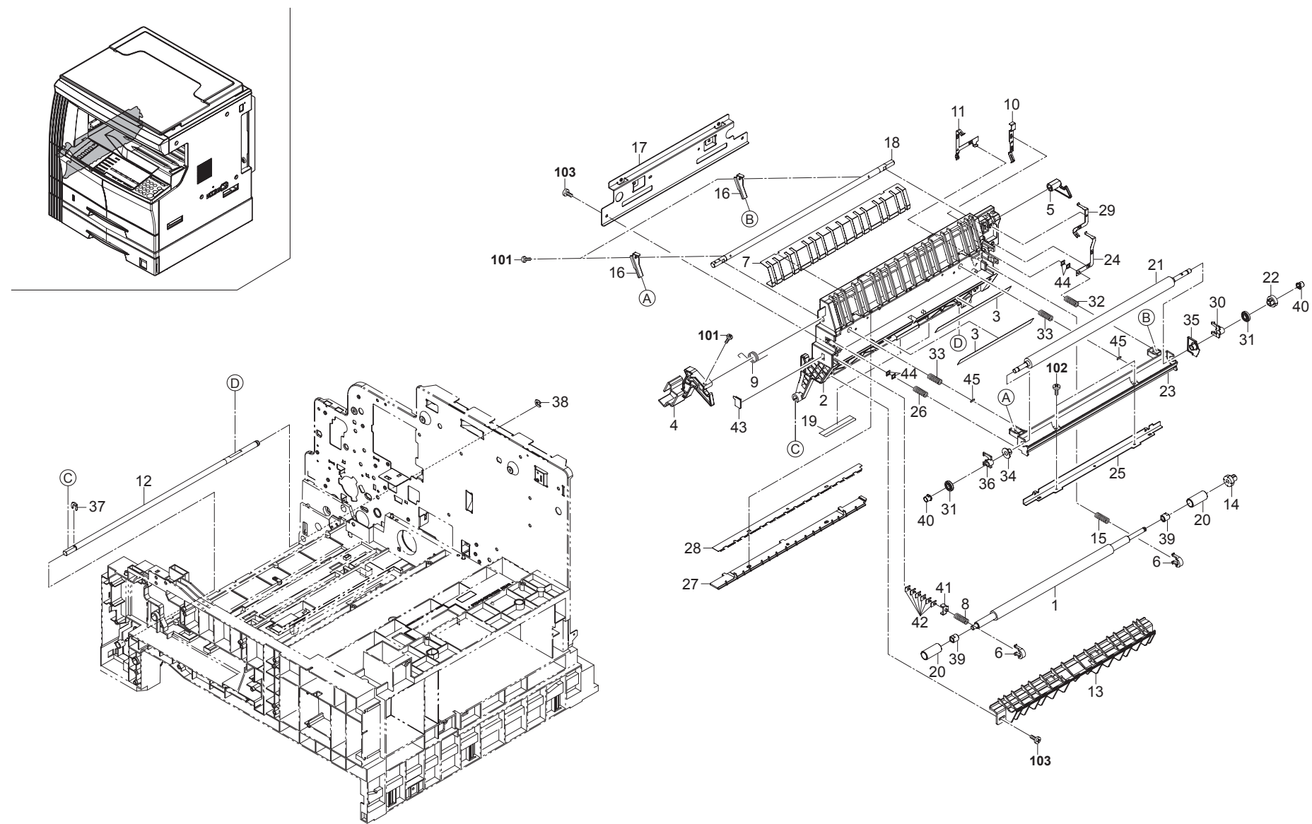
FIG. 6 Conveying Section
