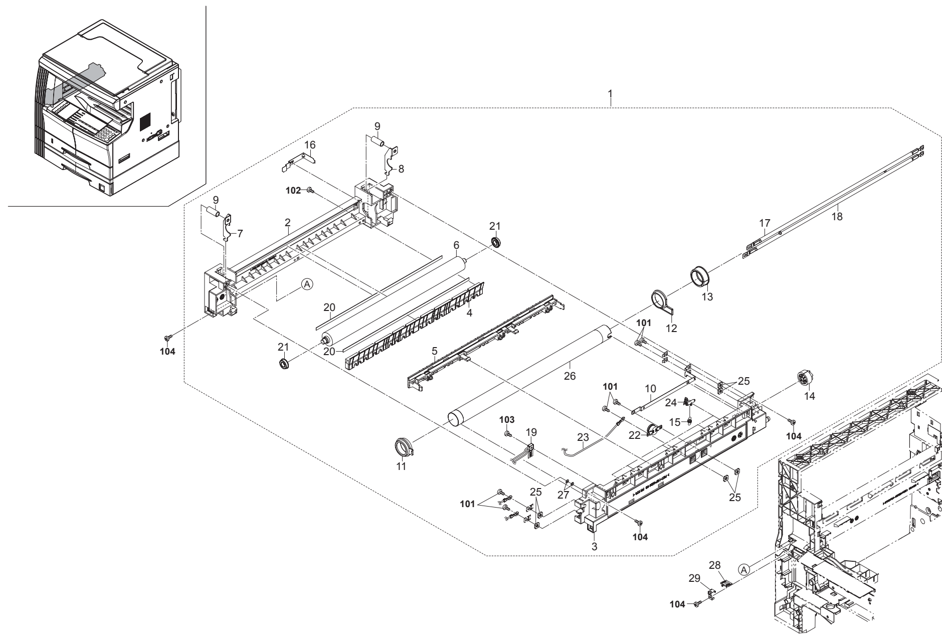
FIG. 12 Fuser Unit
