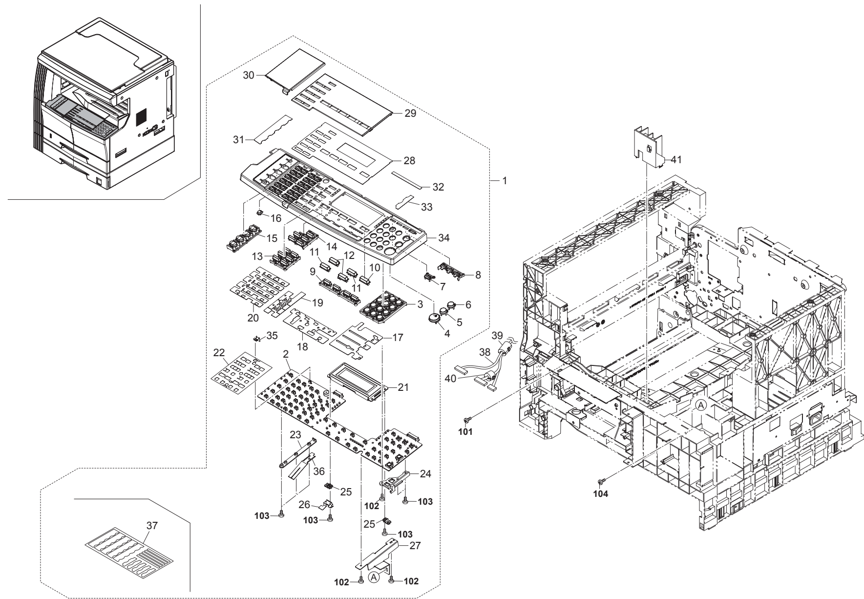
FIG. 15 Operation Unit
