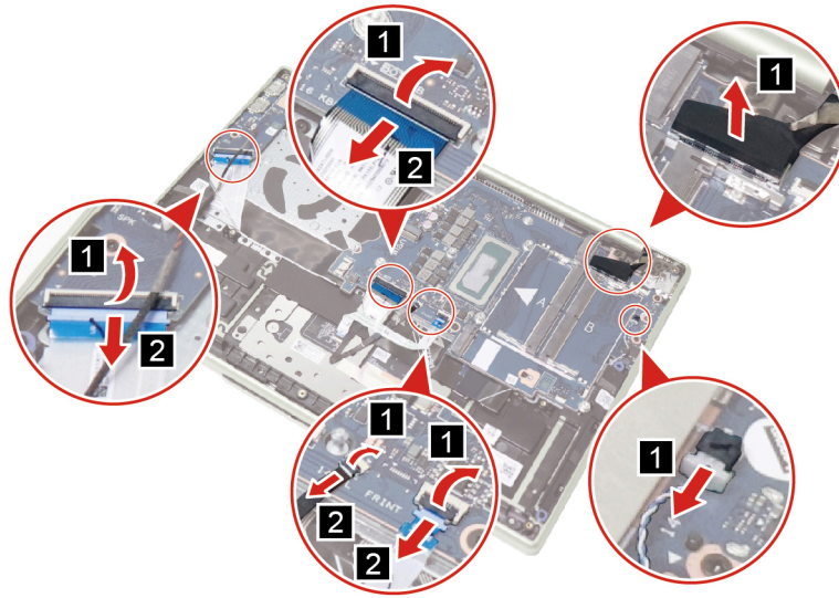
Figure 26. Disconnect cables
