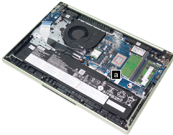
Figure 17. Area on the system board where thermal interface materials are applied (for AMD models)
