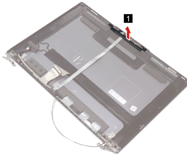
Figure 55. Remove the OLED bracket
