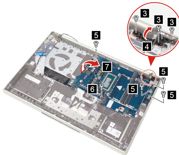
Figure 27. Remove eight screws and the system board
