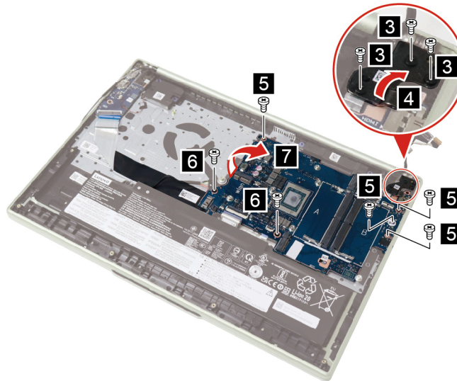
Figure 30. Remove eight screws and the system board
