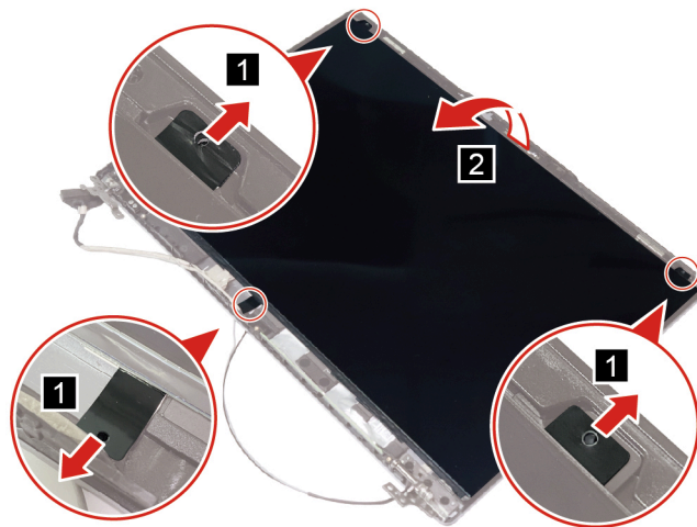
Figure 53. Pull out five pieces of the removable tape and turn over the OLED panel
