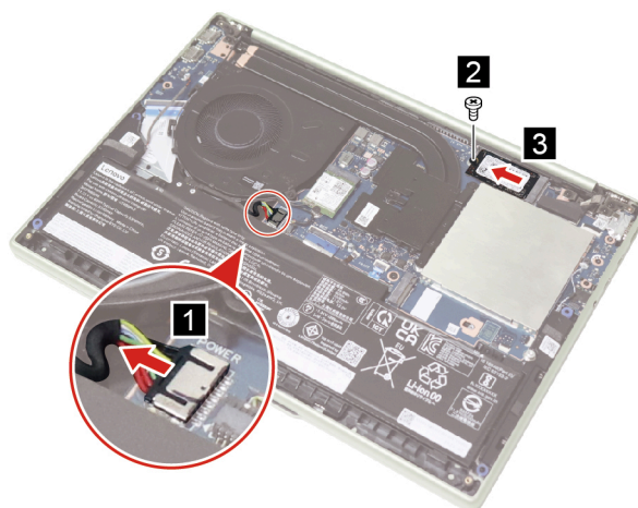
Figure 6. Disconnect the battery pack cable, remove one screw, and remove the M.2 solid-state drive
