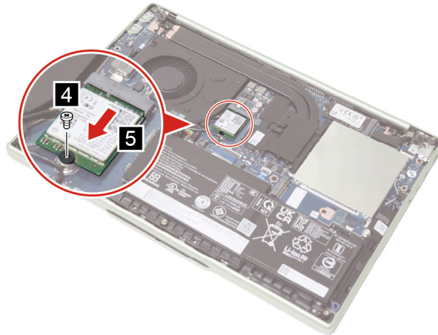
Figure 8. Remove one screw and the Wi-Fi card
