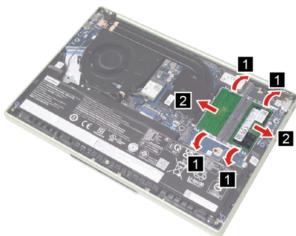
Figure 11. Open the latches and remove the memory module
