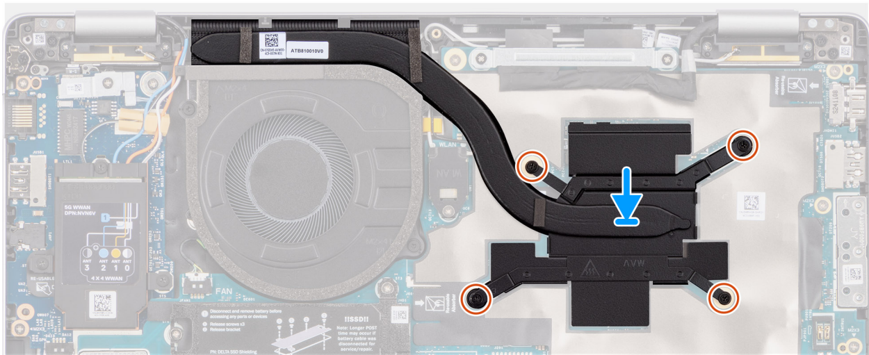
Figure 41. Installing the heat sink
