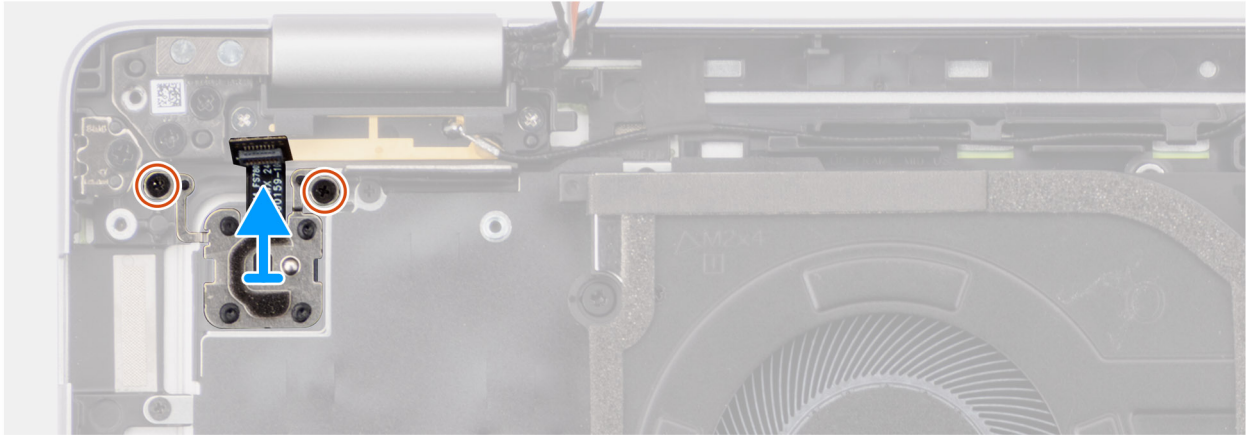
Figure 59. Remove the power button with optional fingerprint reader
