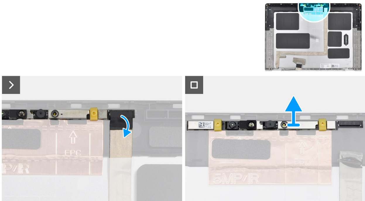
Figure 79. Removing the IR camera
