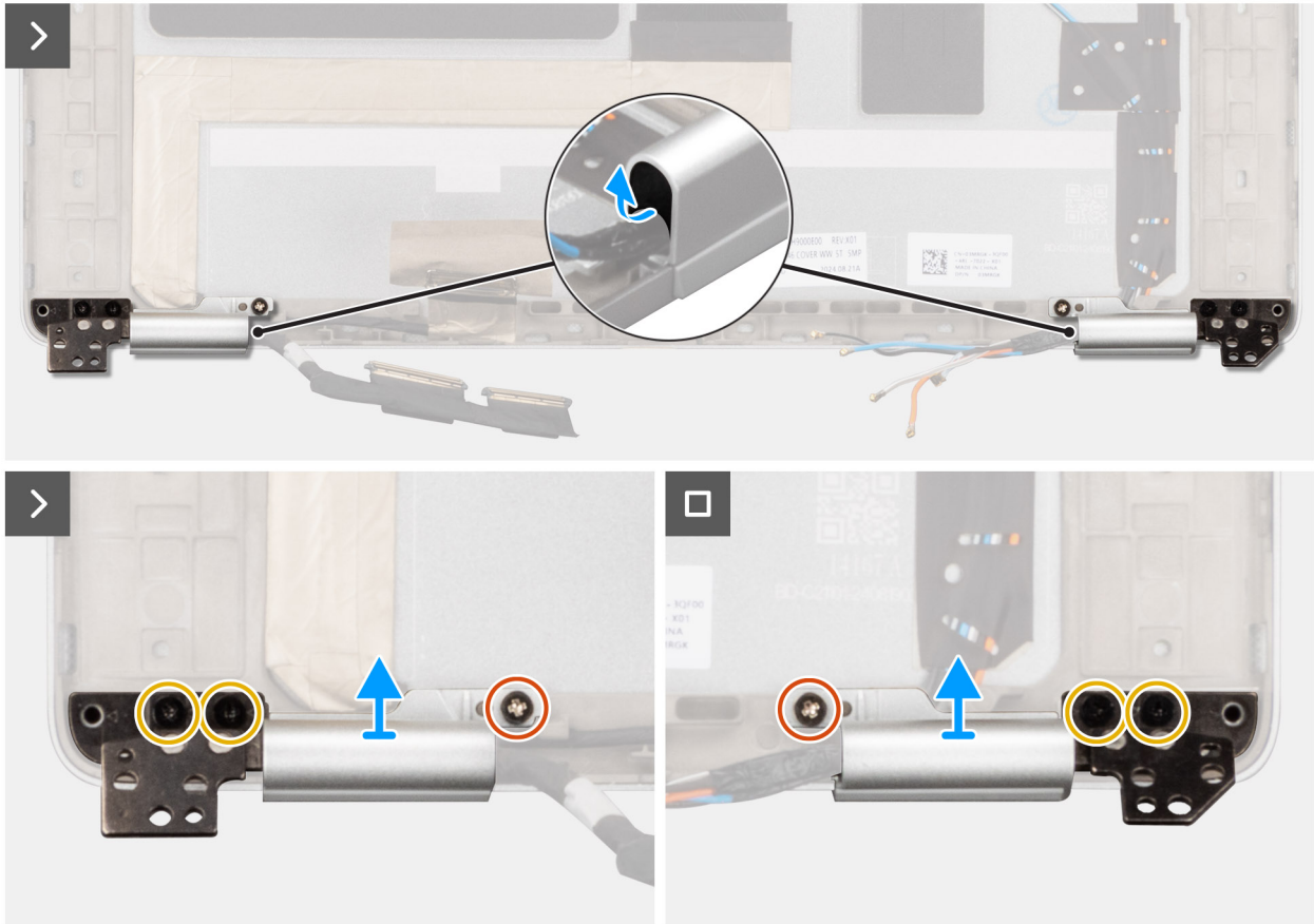
Figure 77. Removing the display hinges
