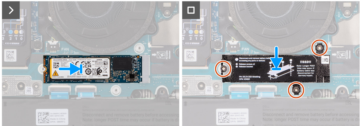
Figure 34. Installing the M.2 2280 SSD
