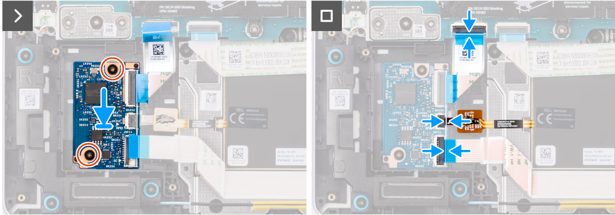
Figure 43. Installing the USH board
