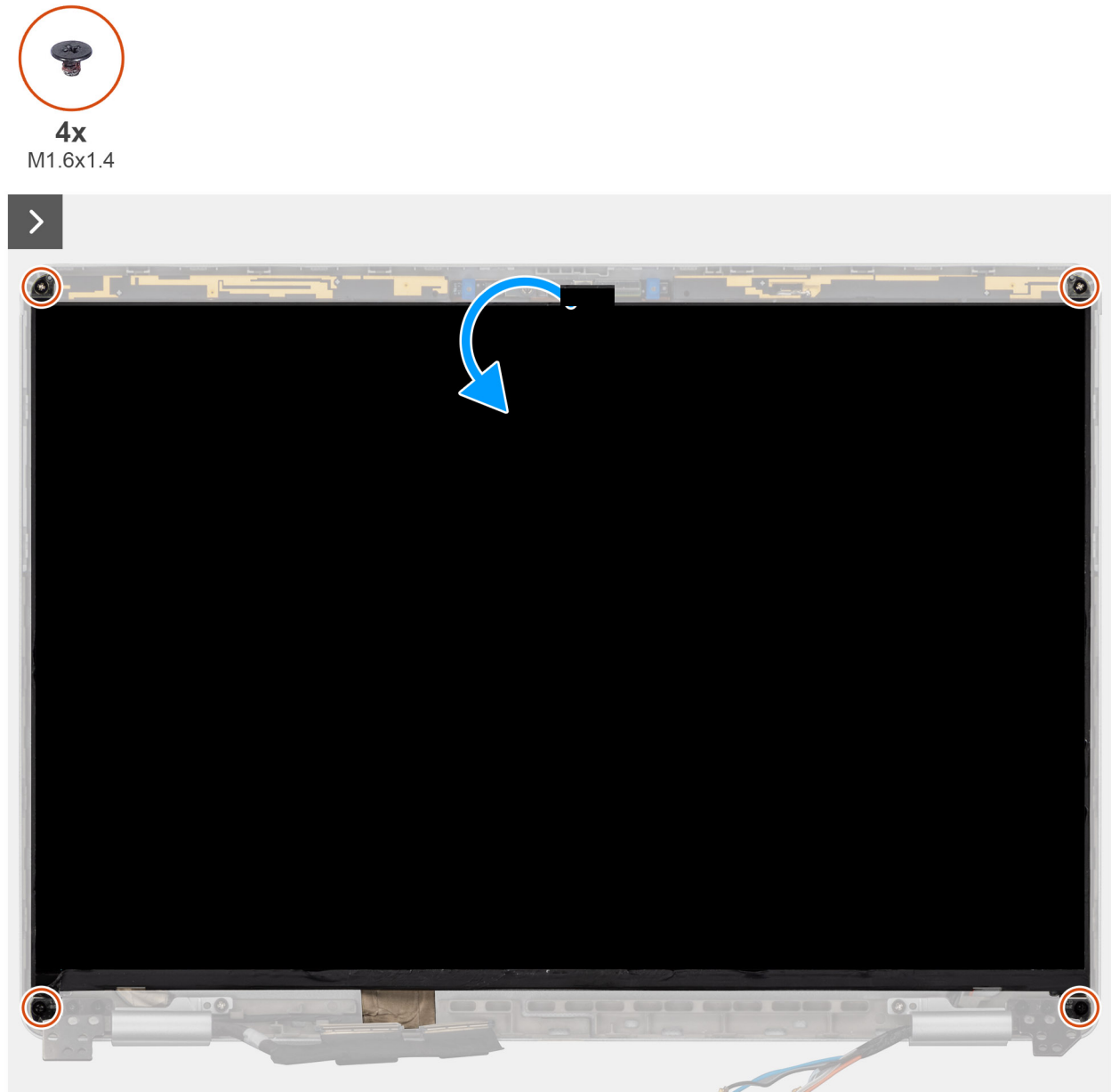
Figure 72. Removing the display panel
