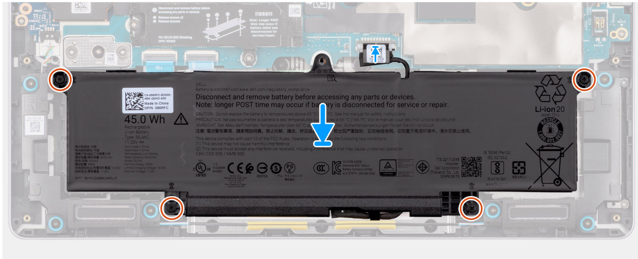
Figure 24. Installing the battery
