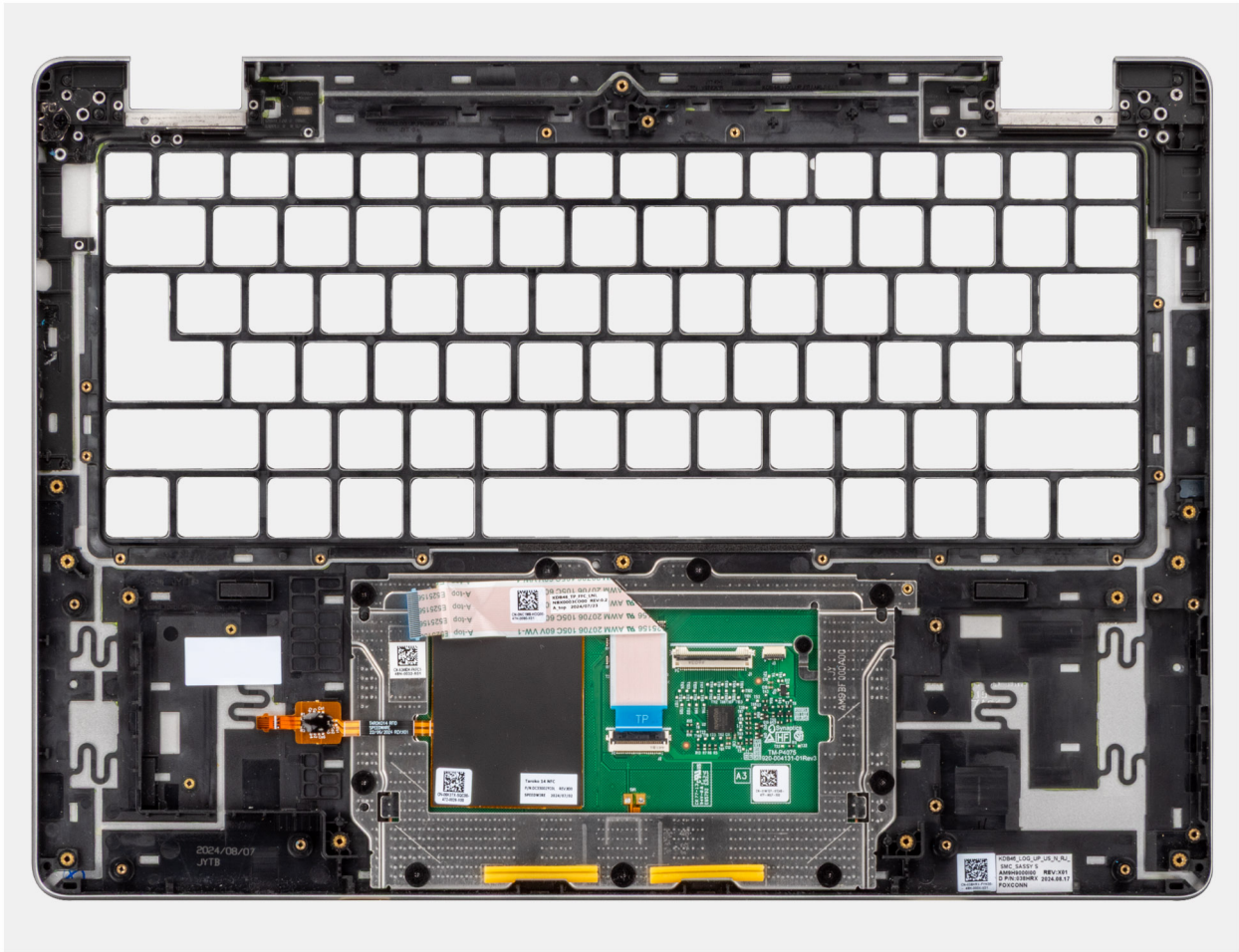
Figure 101. Palm-rest assembly
