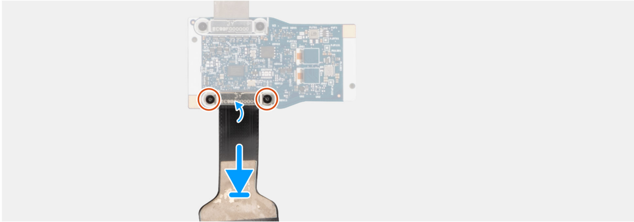
Figure 90. Installing the display cable for MIPI camera to middle board
