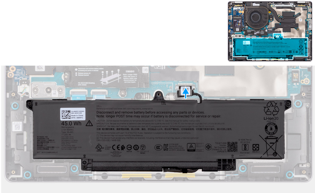
Figure 20. Connecting the battery cable
