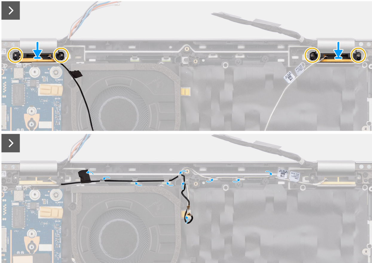
Figure 53. Installing the WLAN antenna modules
