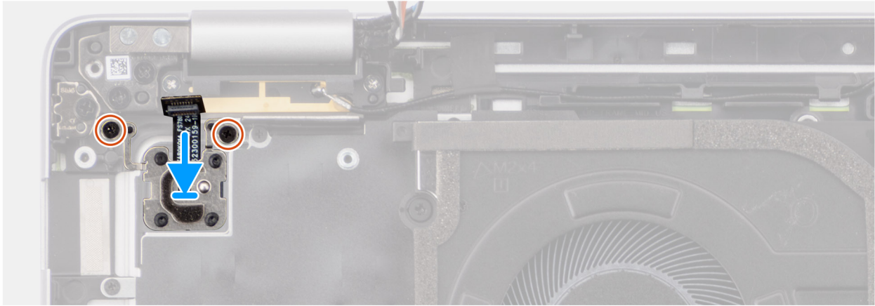
Figure 60. Installing the power button with optional fingerprint reader
