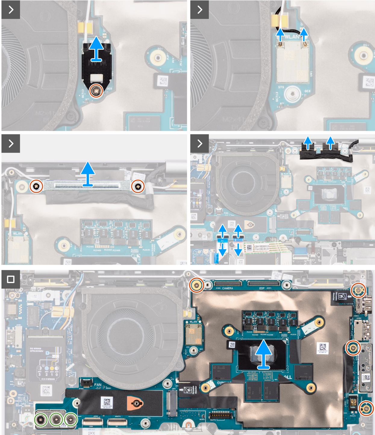
Figure 47. Removing the system board
