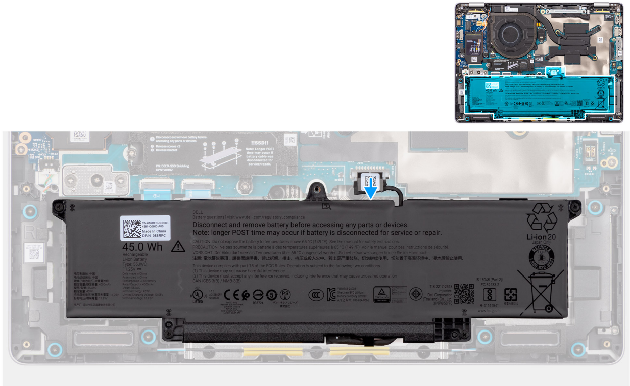
Figure 19. Disconnecting the battery cable
