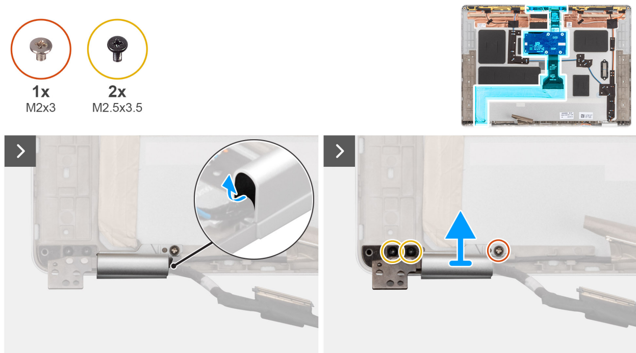
Figure 85. Removing the display cable for RGB/IR camera
