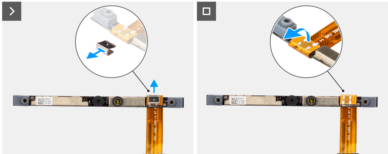
Figure 119. Removing the camera
