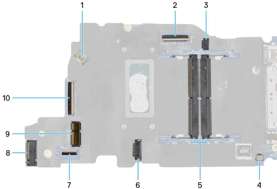
Figure 57. System-board connectors
