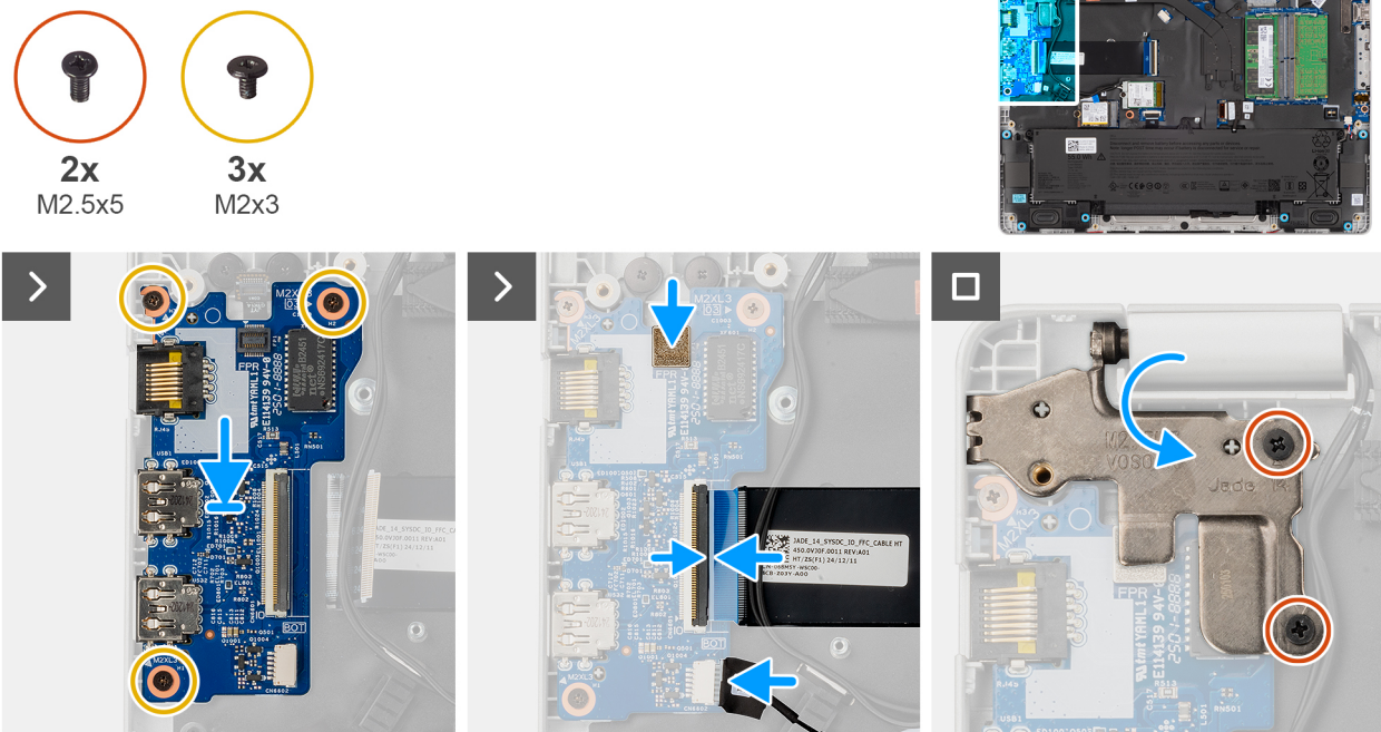
Figure 52. Installing the I/O board
