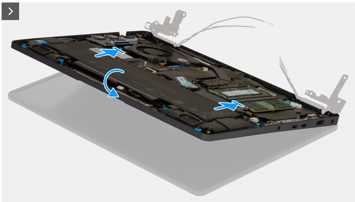
Figure 102. Installing the display assembly
