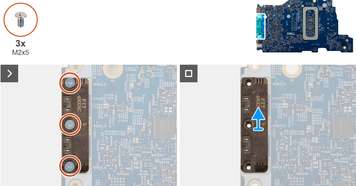
Figure 75. Removing the USB Type-C module
