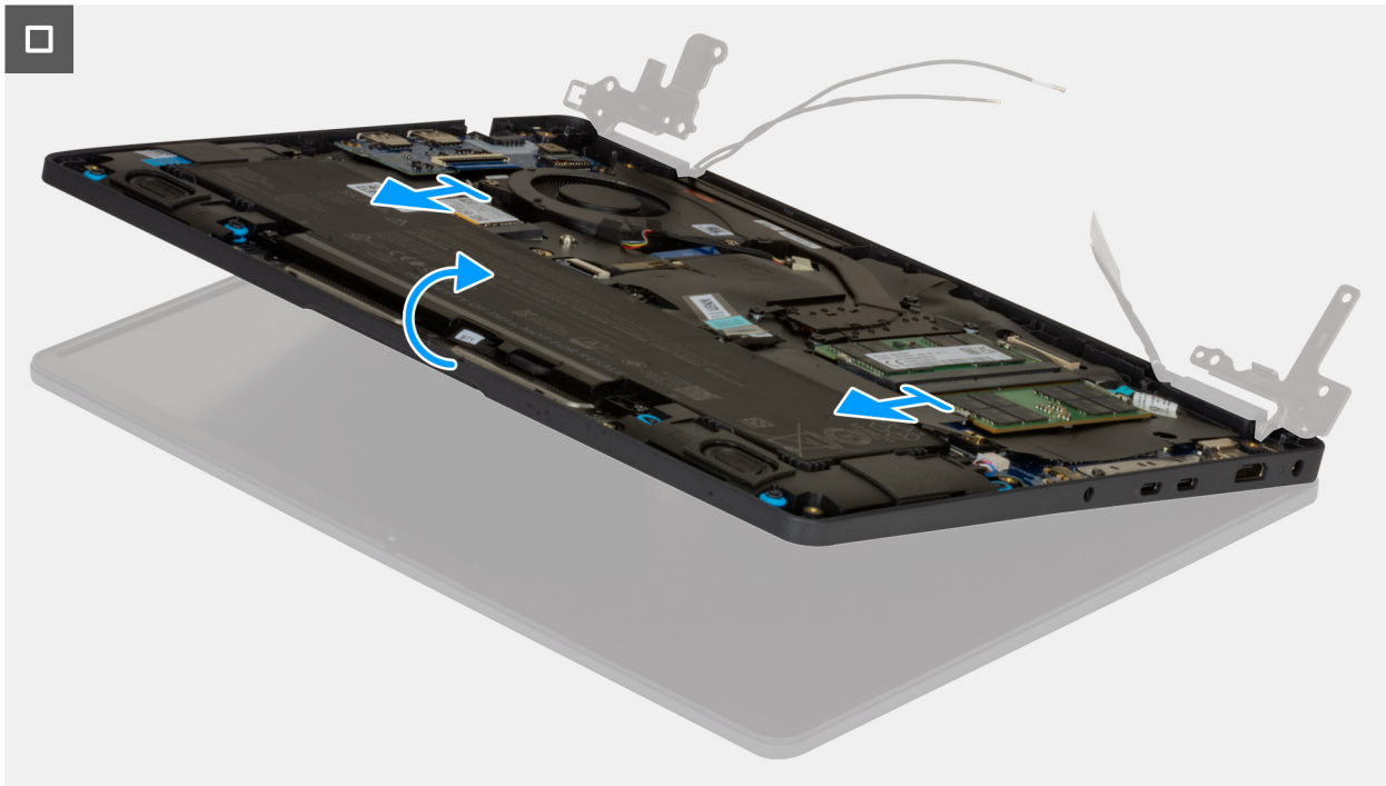
Figure 100. Removing the display assembly
