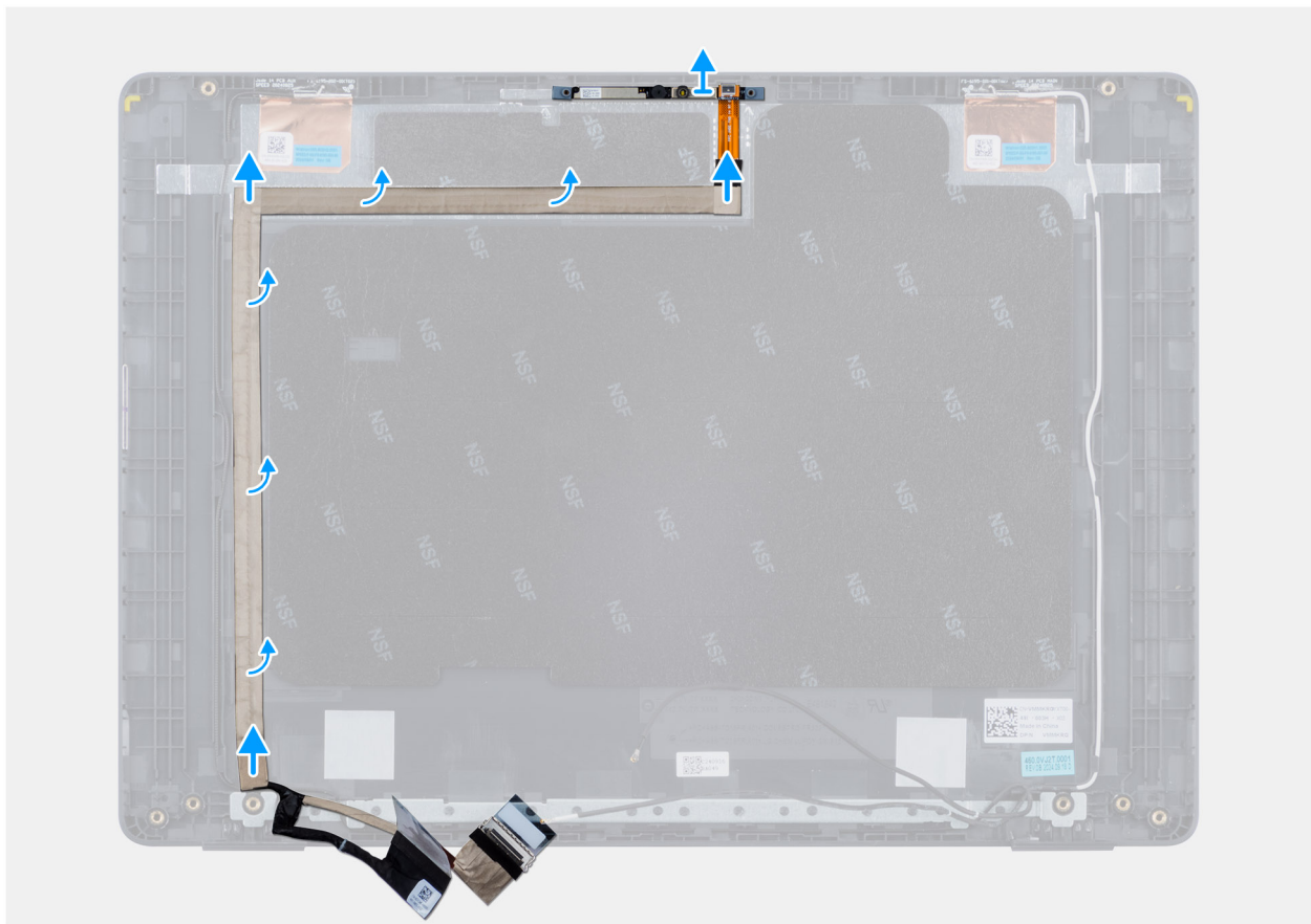
Figure 121. Removing the eDP cable
