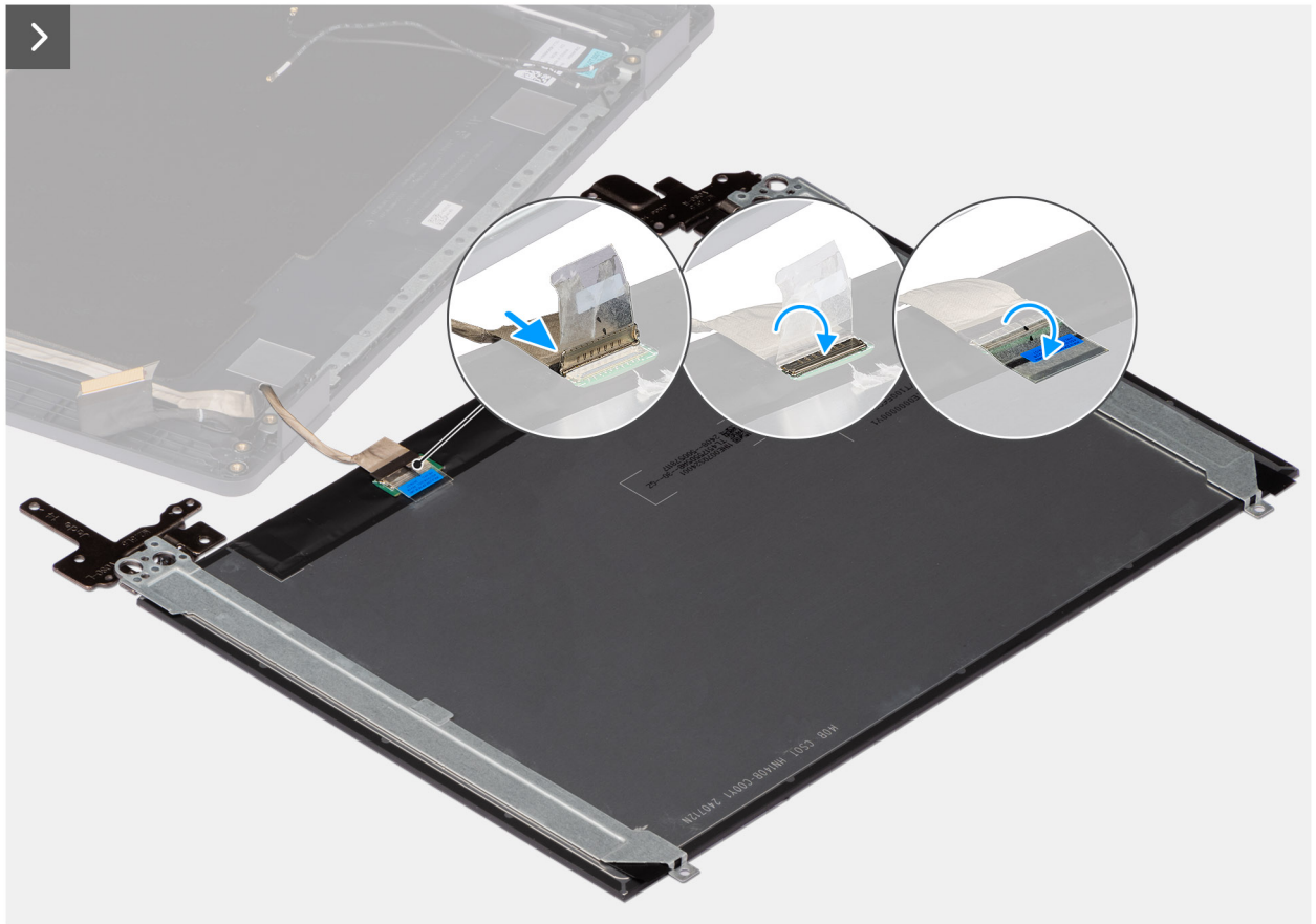
Figure 116. Installing the display-panel assembly
