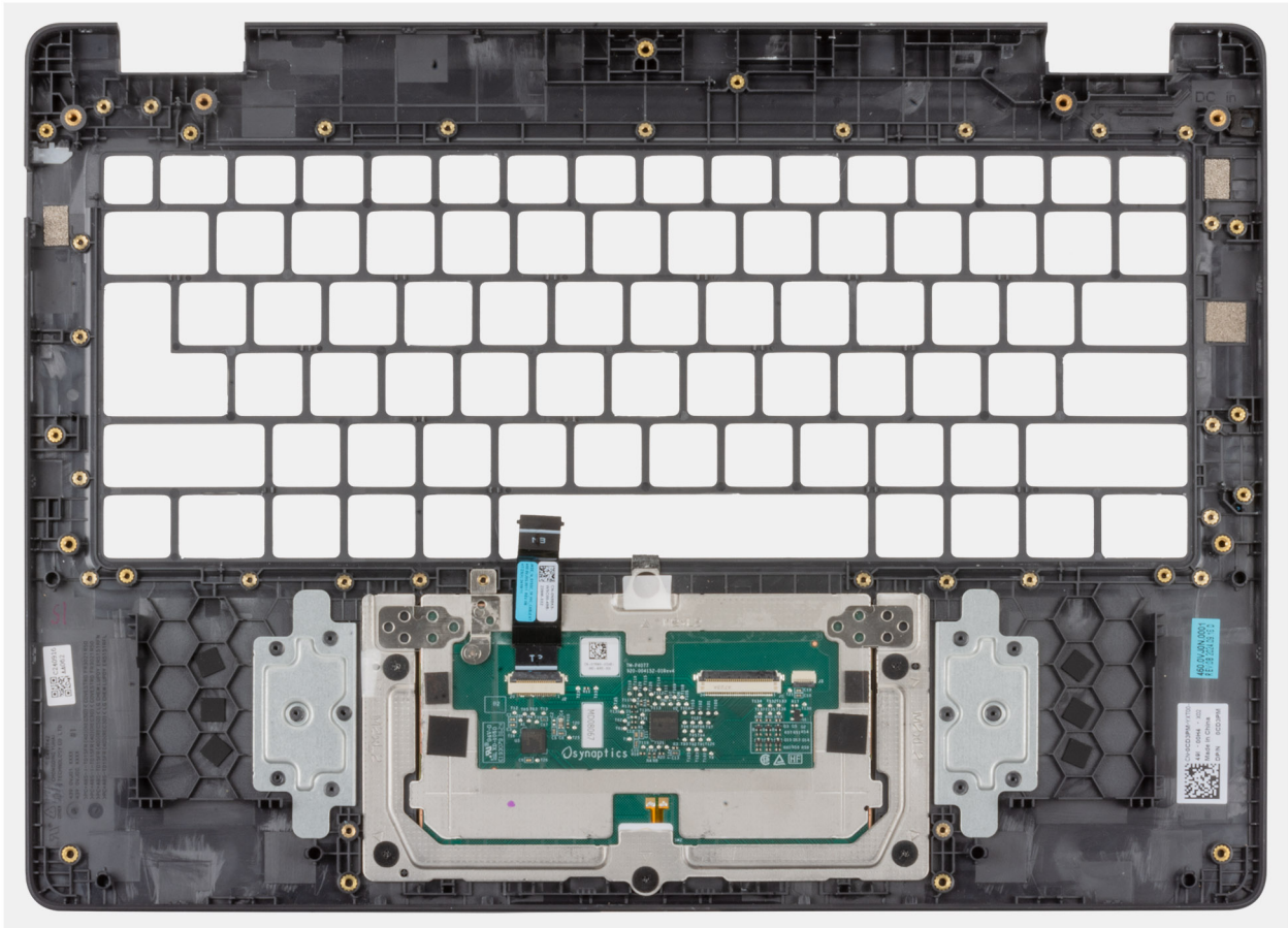
Figure 95. Removing the palm-rest and assembly
