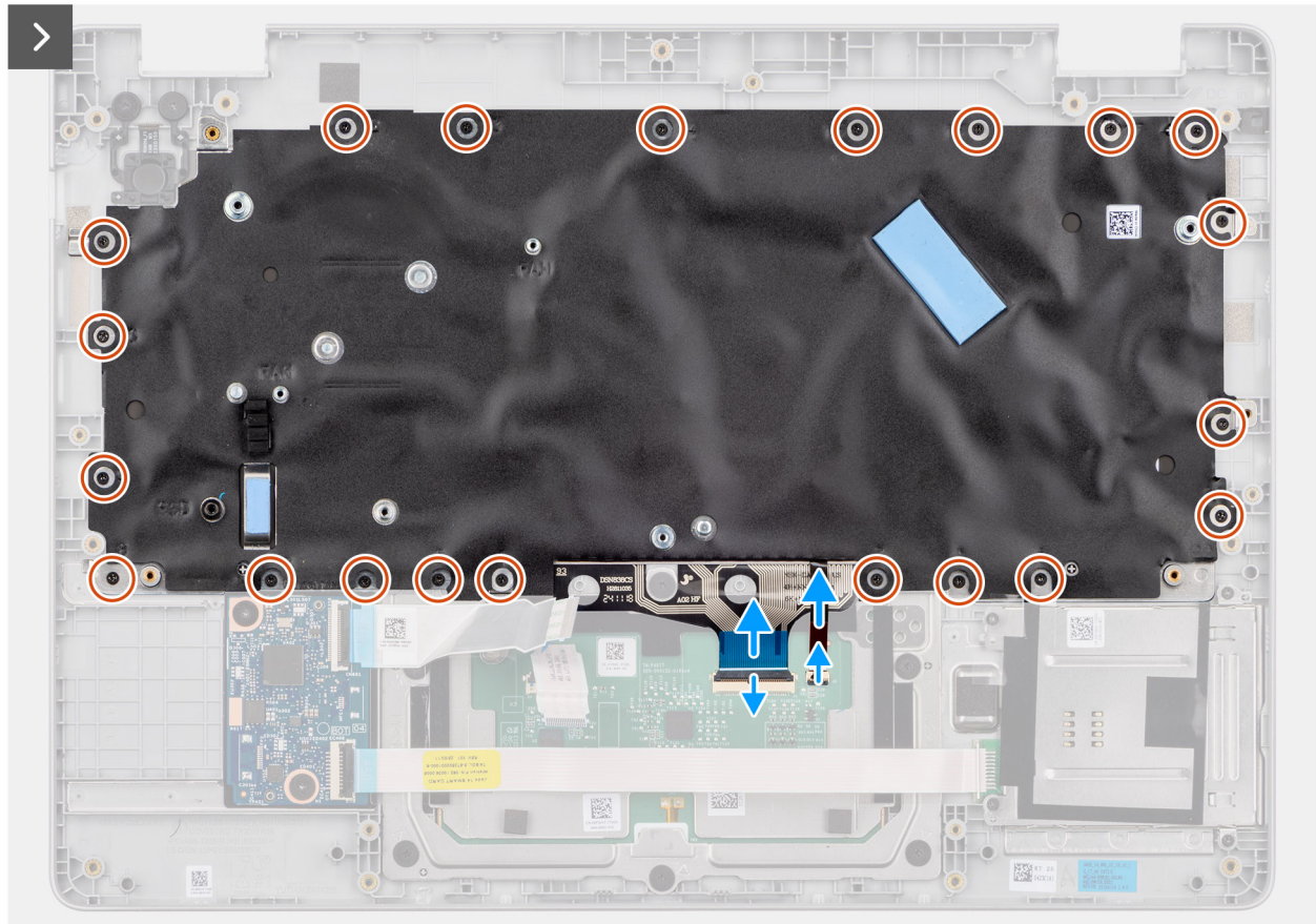
Figure 85. Removing the keyboard
