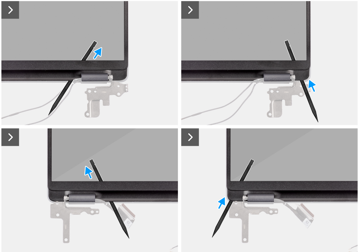
Figure 106. Removing the display bezel
