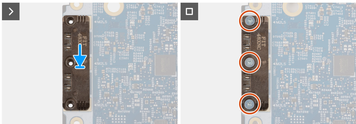
Figure 76. Installing the USB Type-C module
