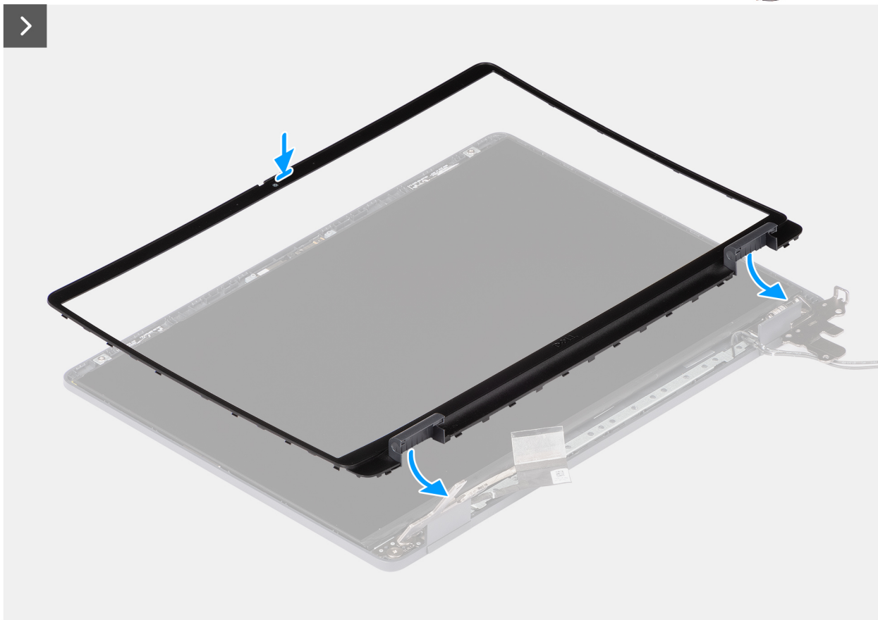
Figure 109. Installing the display bezel
