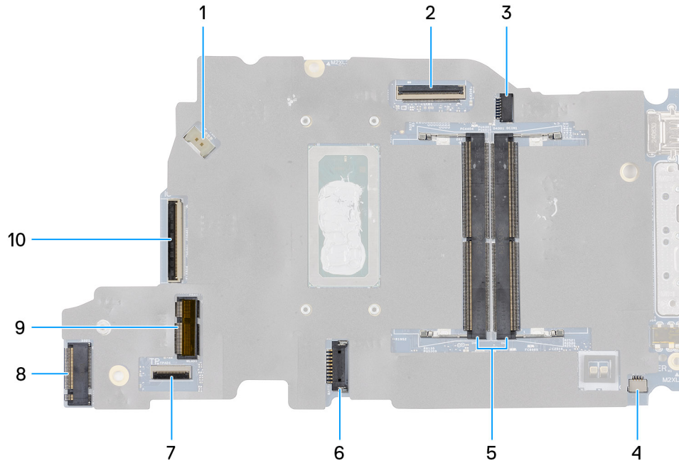
Figure 60. System-board connectors
