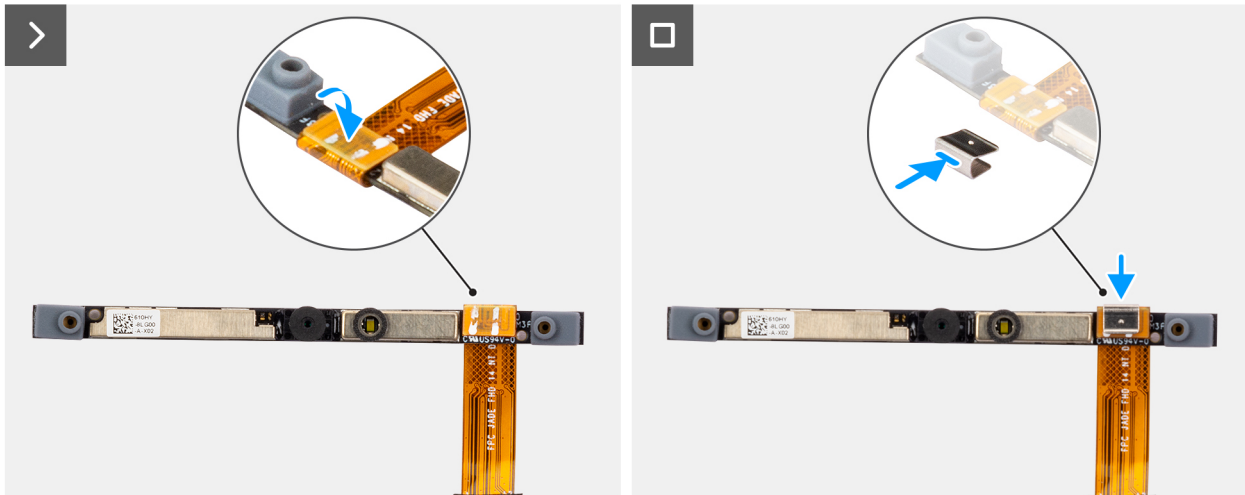
Figure 120. Installing the camera
