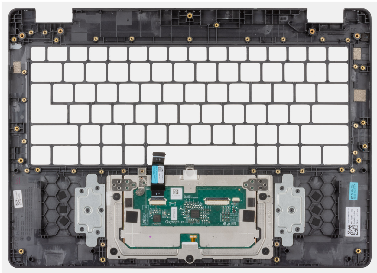
Figure 96. Installing the palm-rest assembly
