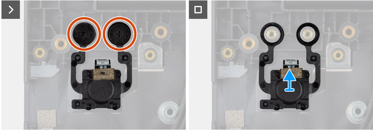
Figure 55. Removing the power button with fingerprint reader
