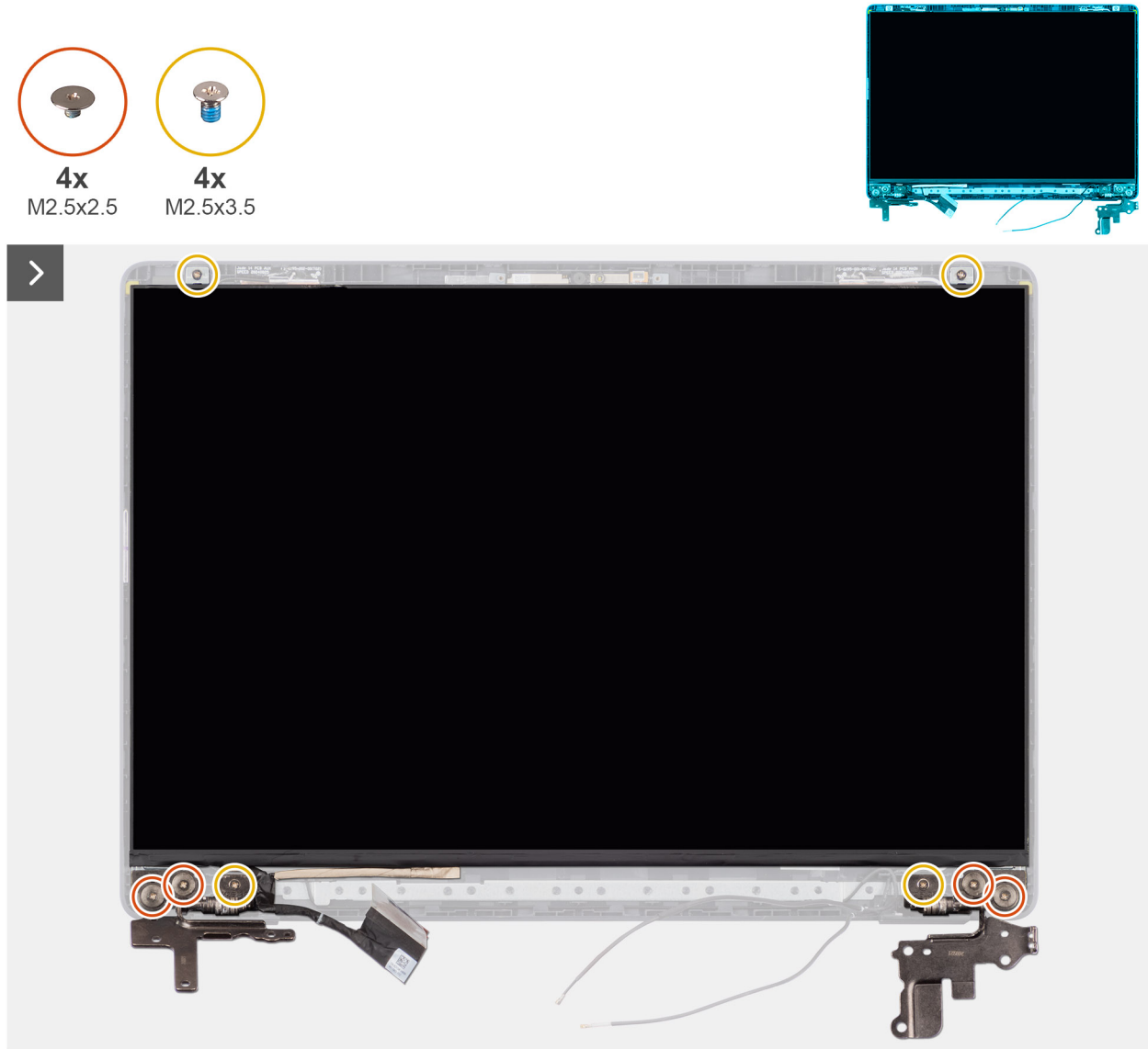
Figure 111. Removing the display-panel assembly assembly
