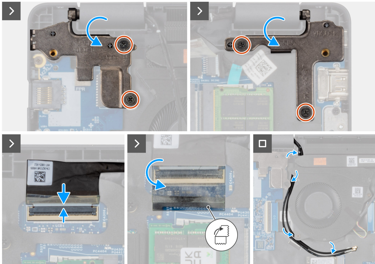
Figure 103. Installing the display assembly
