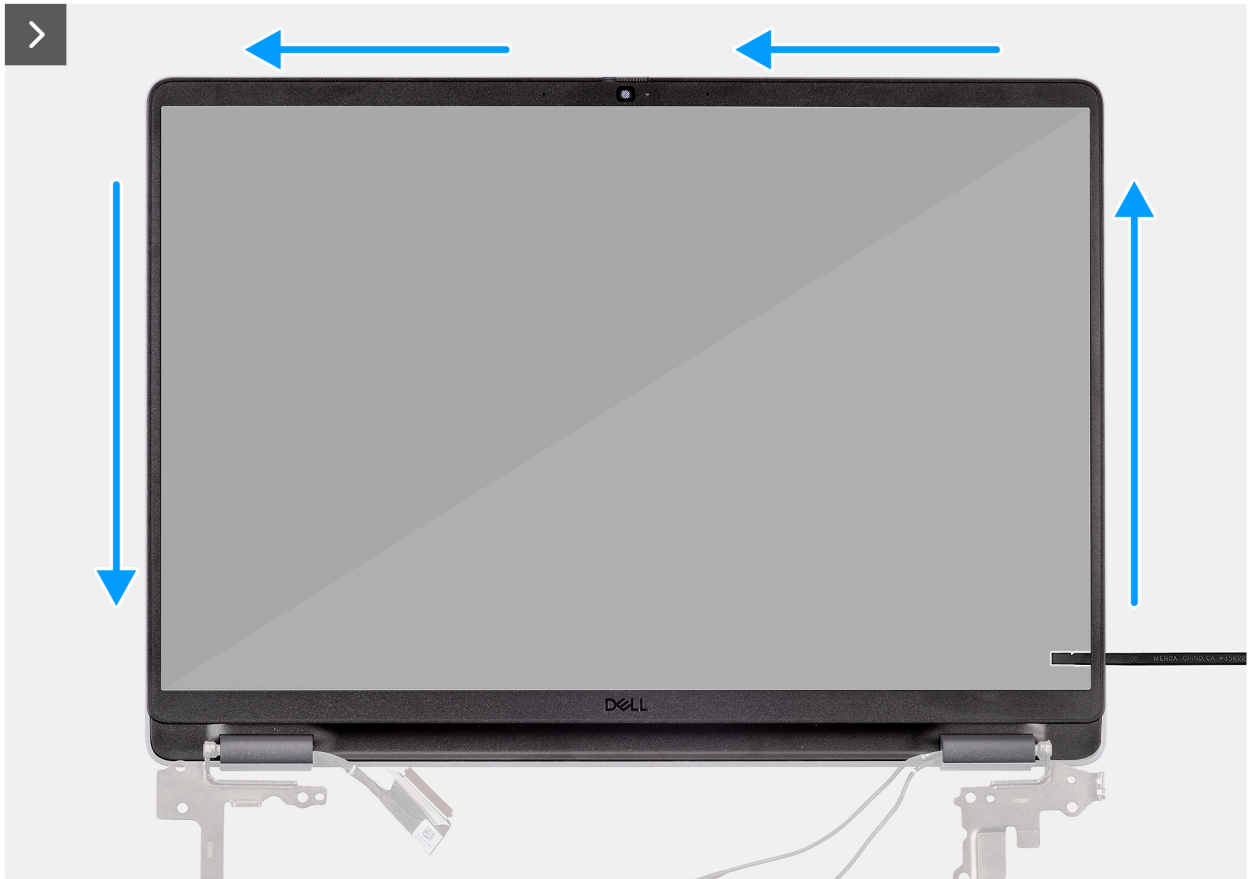
Figure 107. Removing the display bezel
