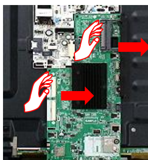
PUSH the PCB to Direction
