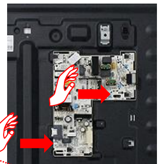
PUSH the PCB to Direction
