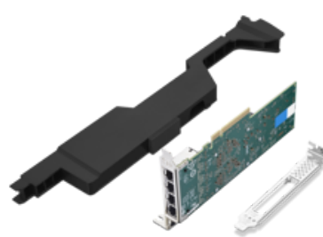
ThinkStation Intel E610-XT4 10GbE 4-Port PCIe Ethernet Adapter
