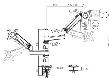
Dimensions (mm)
