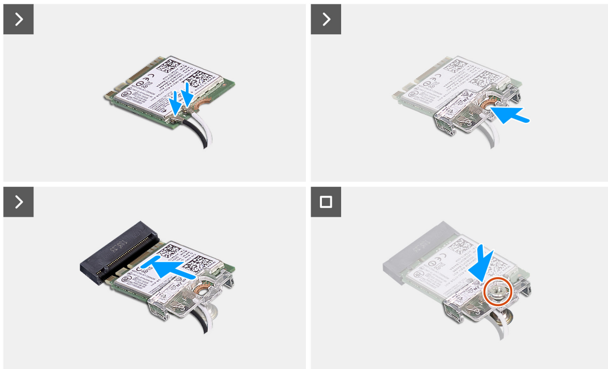
Figure 25. Installing the wireless card
