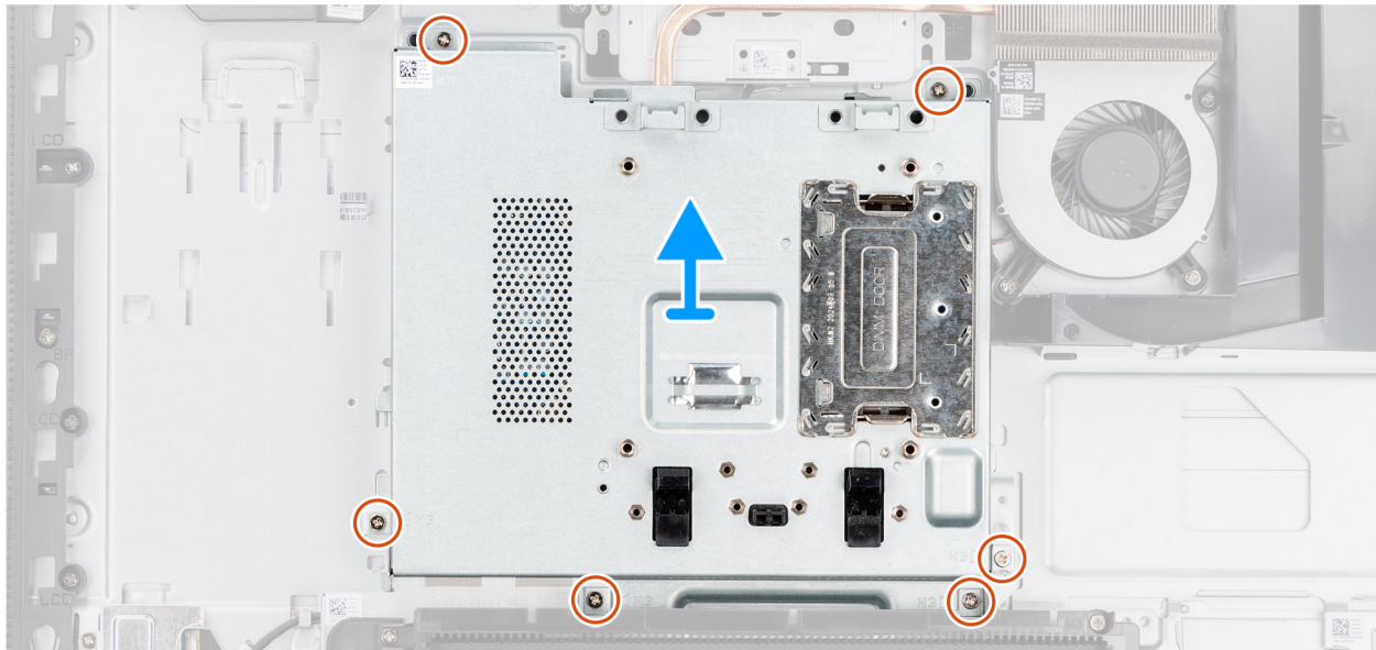
Figure 22. Removing the system-board shield
