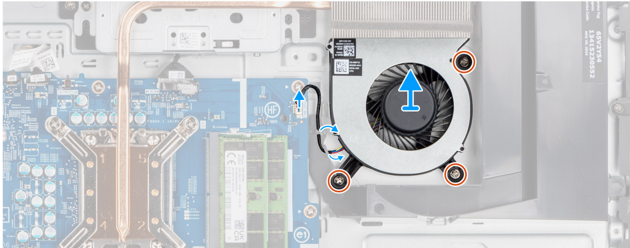
Figure 37. Removing the fan
