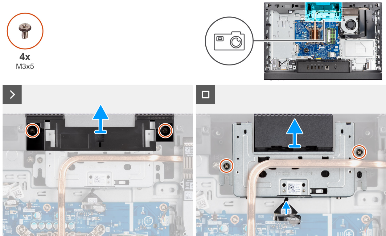
Figure 35. Removing the retractable-camera assembly
