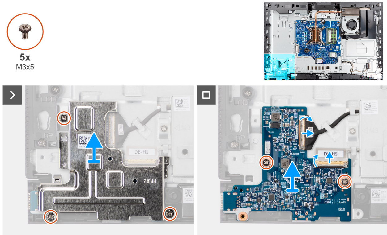
Figure 53. Removing the power-button and I/O board
