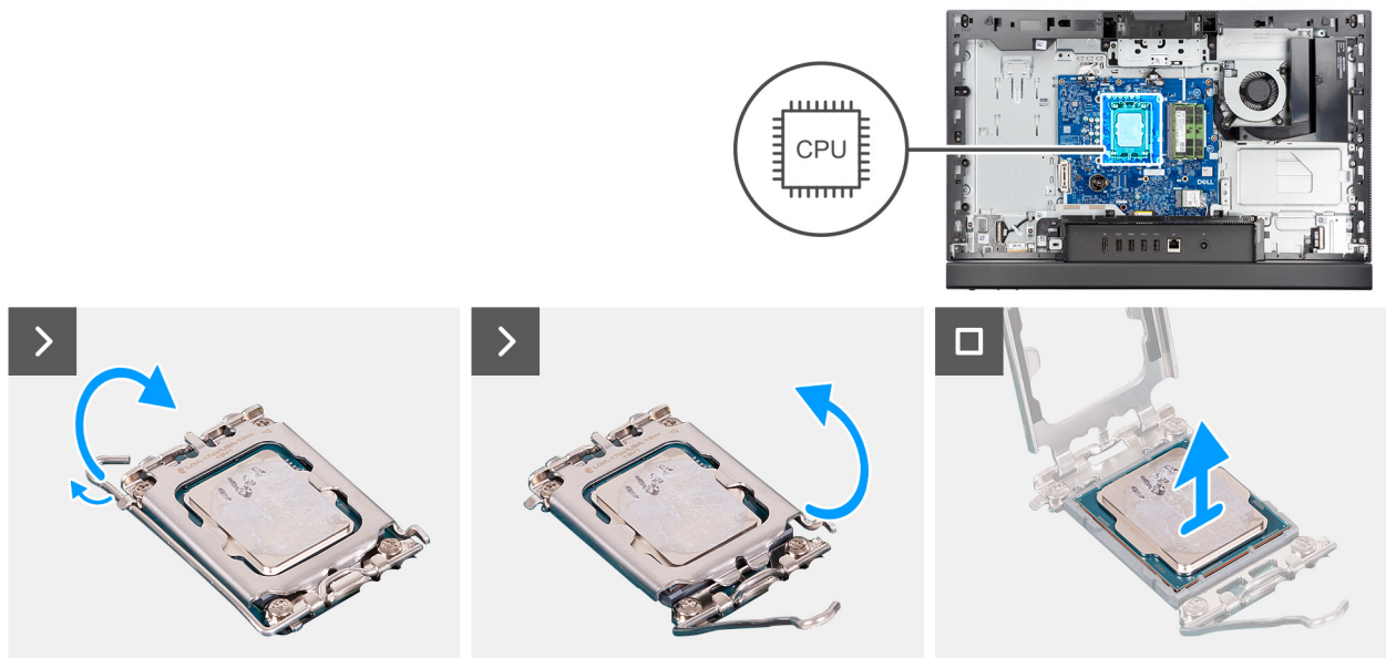
Figure 45. Removing the processor
