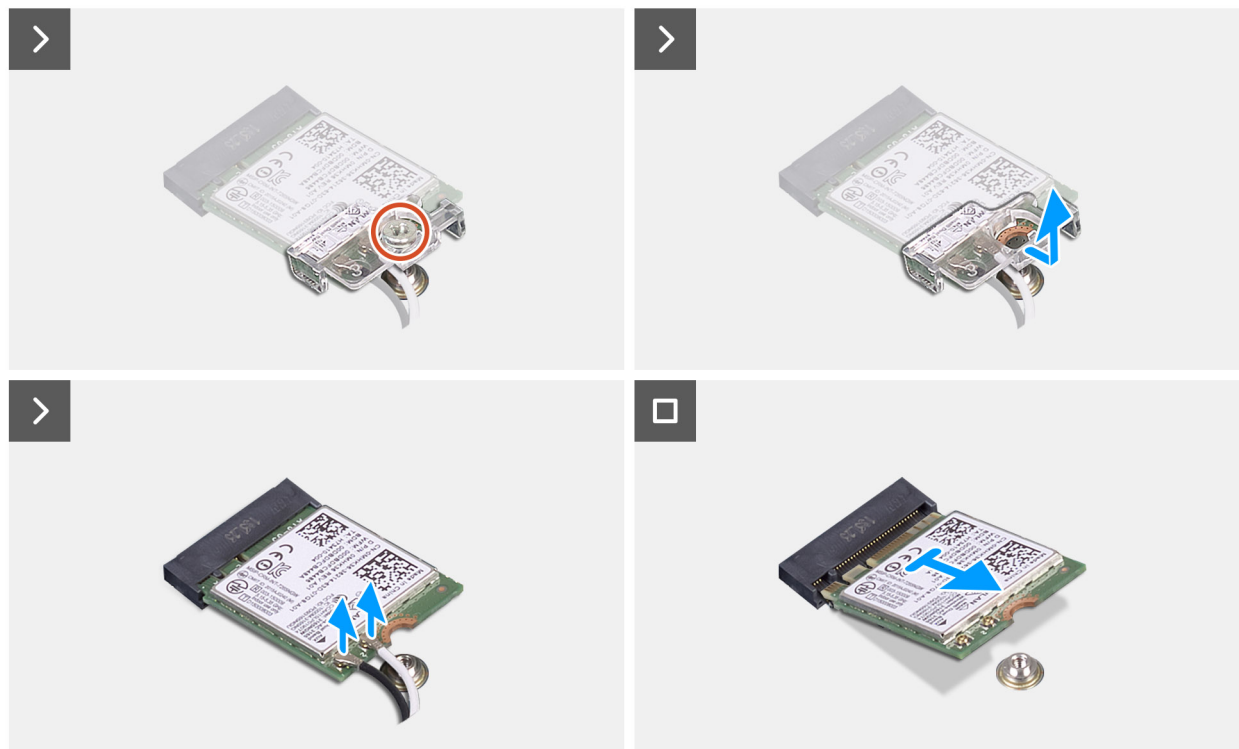
Figure 24. Removing the wireless card
