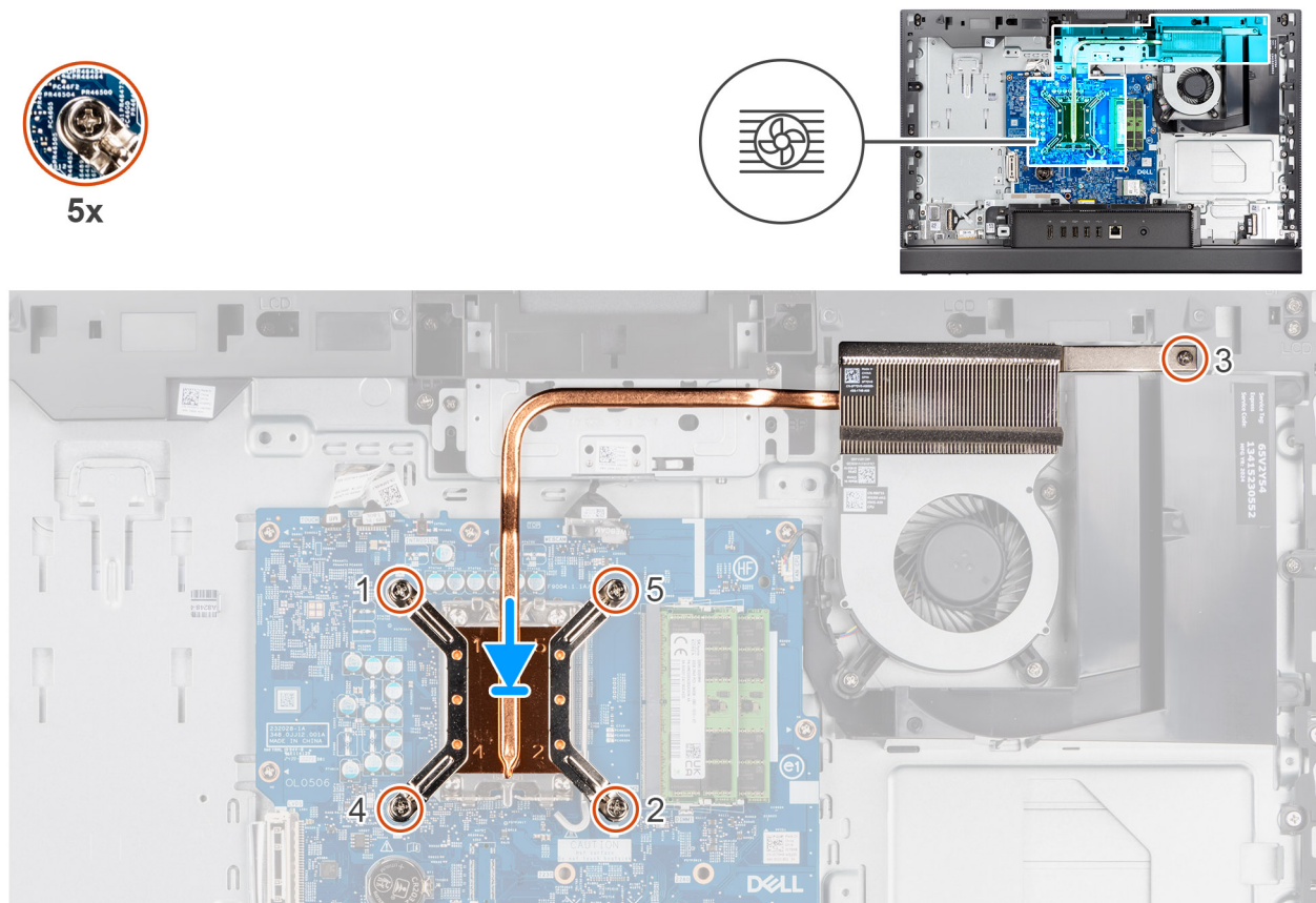
Figure 44. Installing the heat sink
