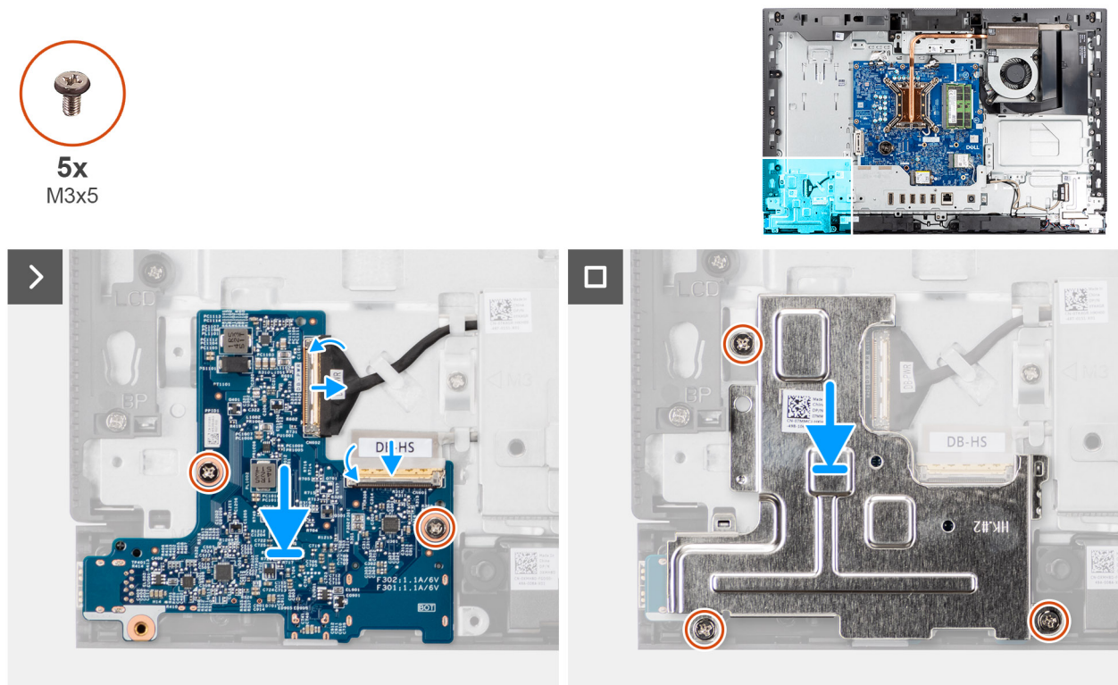
Figure 54. Installing the power-button and I/O board
