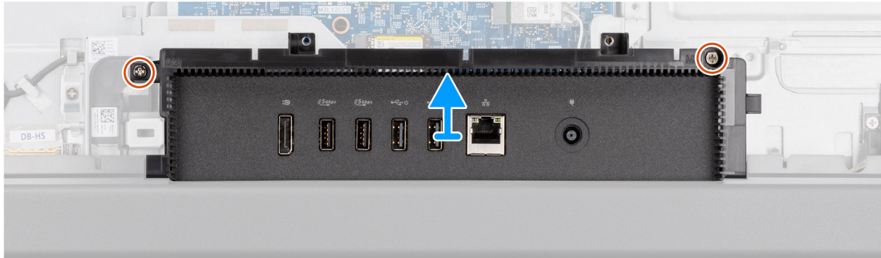
Figure 31. Removing the I/O cover
