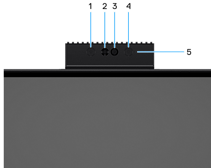
Figure 5. Retractable camera with a 5MP RGB + Infrared camera
