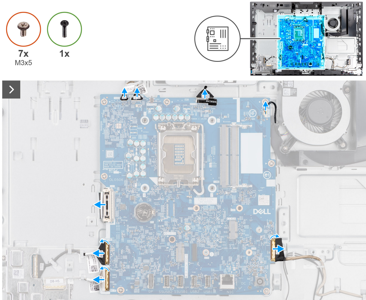
Figure 48. Removing the system board
