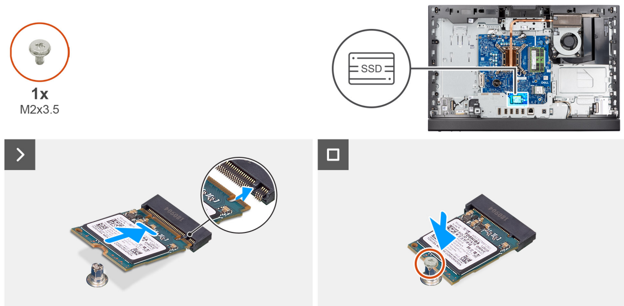
Figure 27. Installing the M.2 2230 solid-state drive
