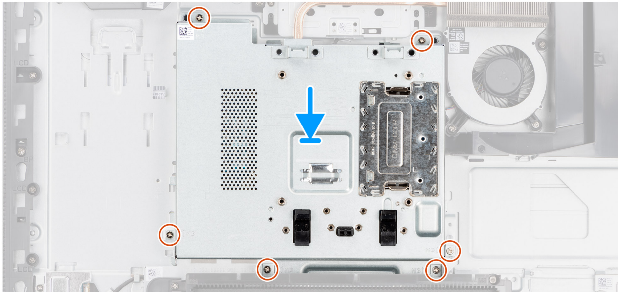
Figure 23. Installing the system-board shield
