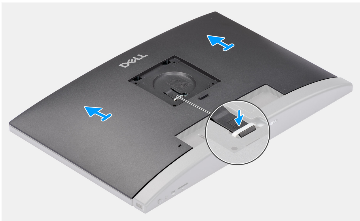
Figure 18. Removing the back cover
