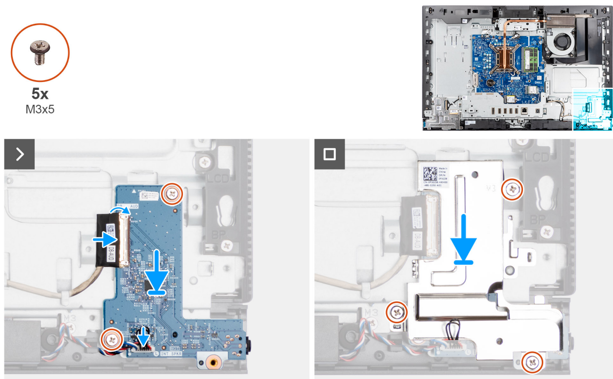
Figure 56. Installing the audio board
