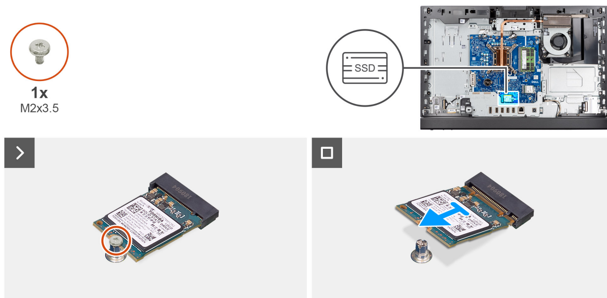
Figure 26. Removing the M.2 2230 solid-state drive
