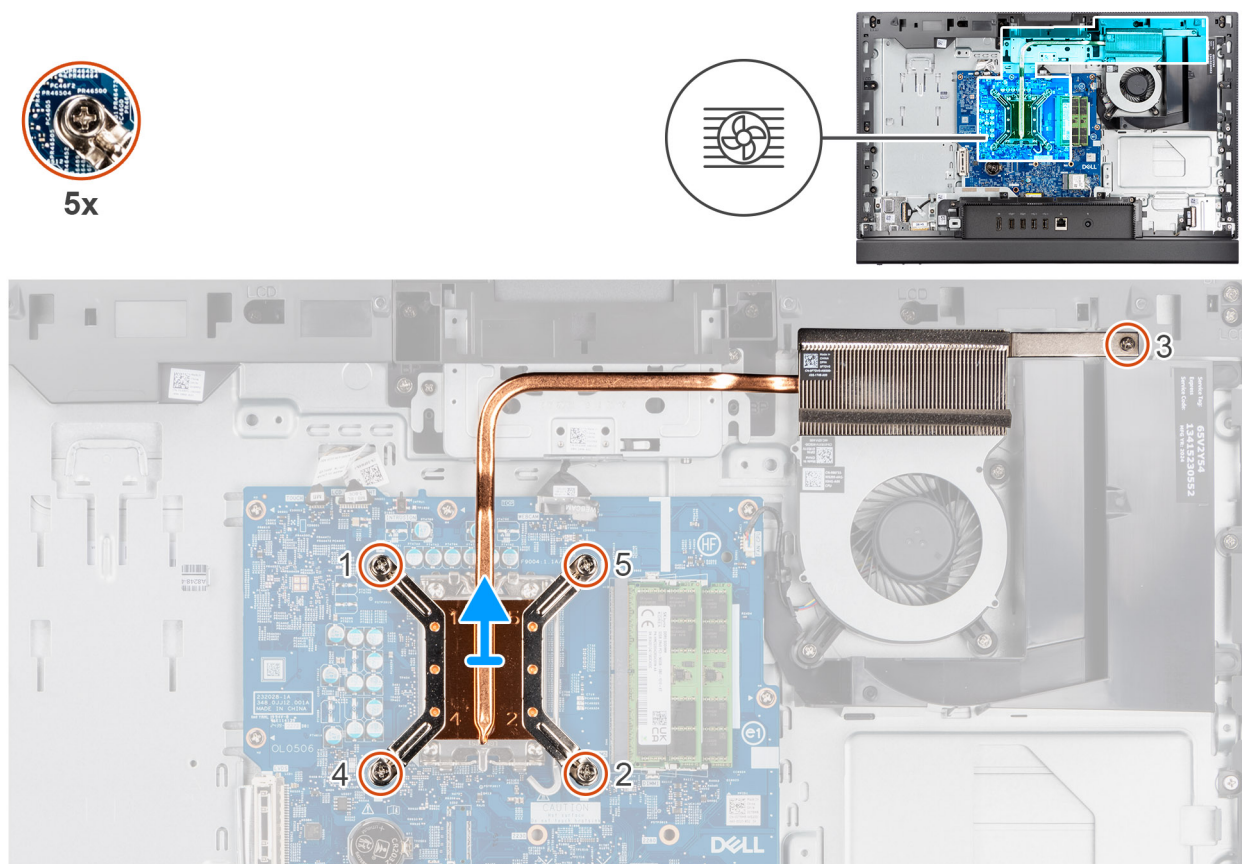
Figure 43. Removing the heat sink
