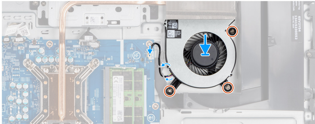
Figure 38. Installing the fan
