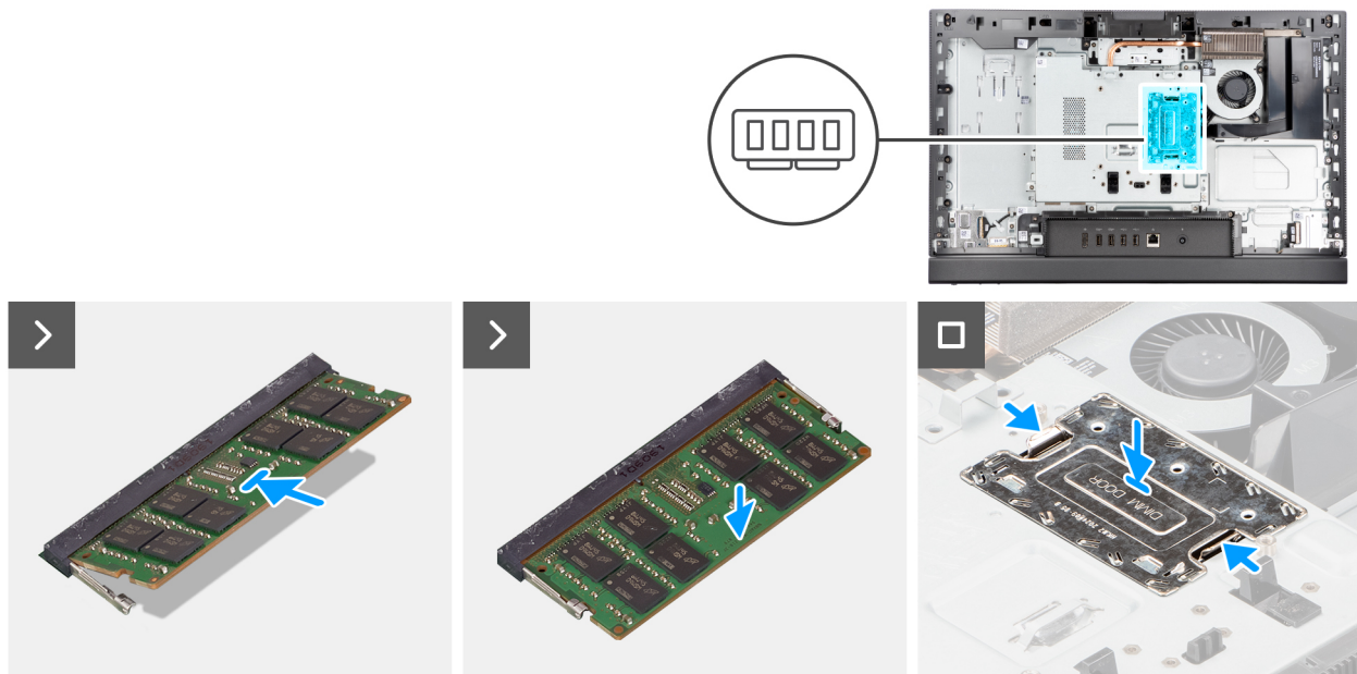
Figure 21. Installing the memory
