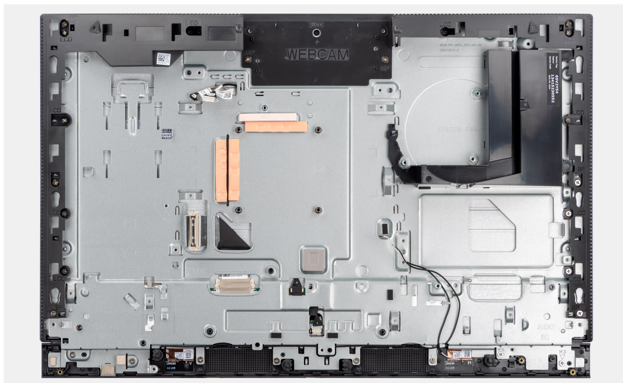
Figure 58. Removing the display-assembly base
