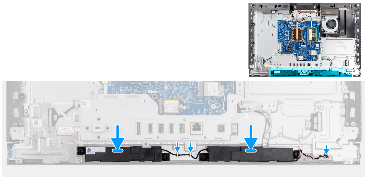
Figure 42. Installing the speakers
