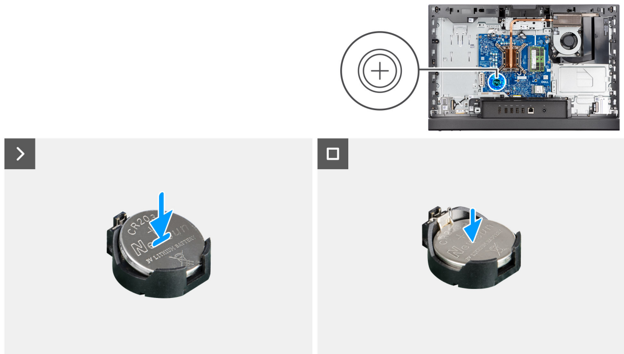
Figure 30. Installing the coin-cell battery
