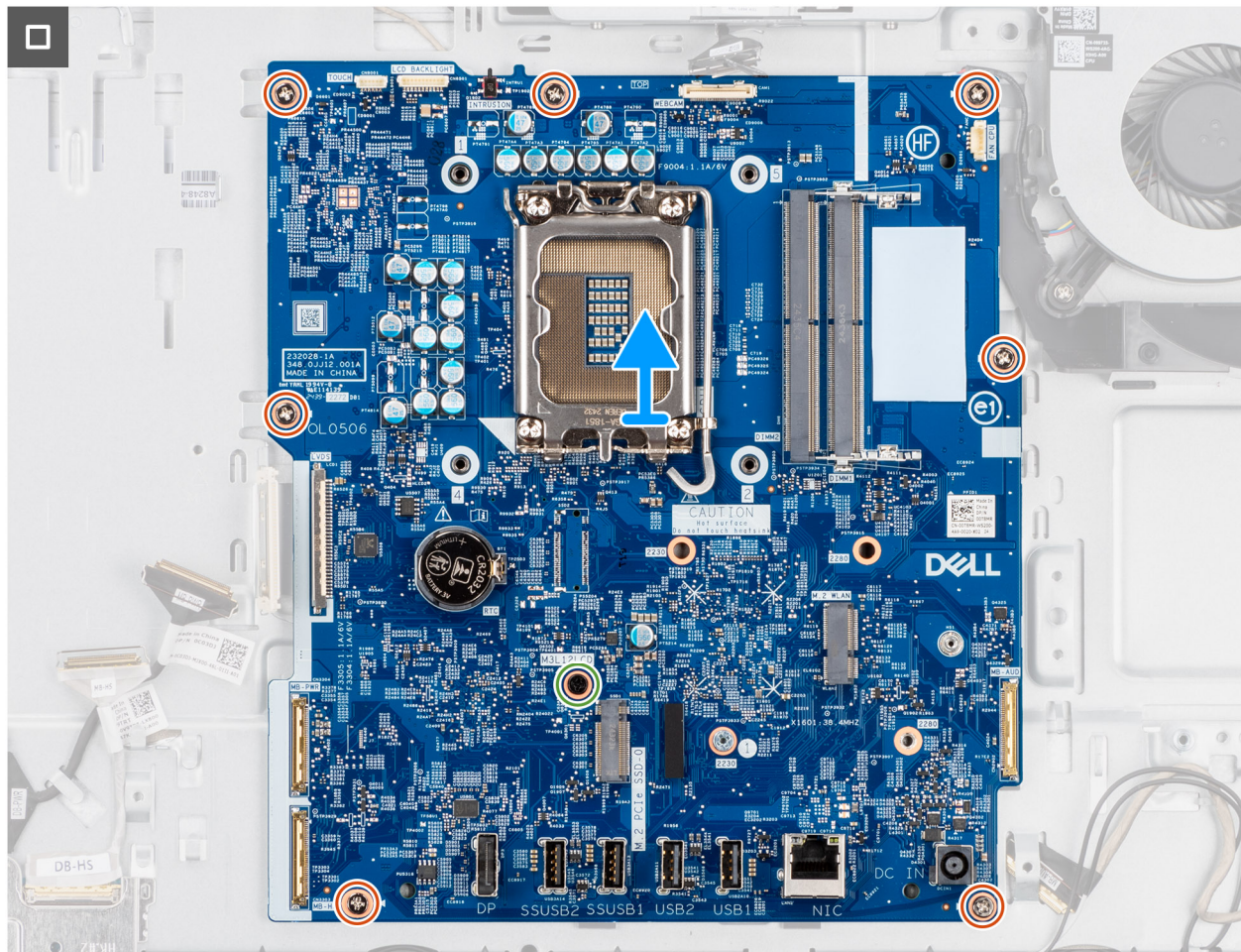
Figure 49. Removing the system board
