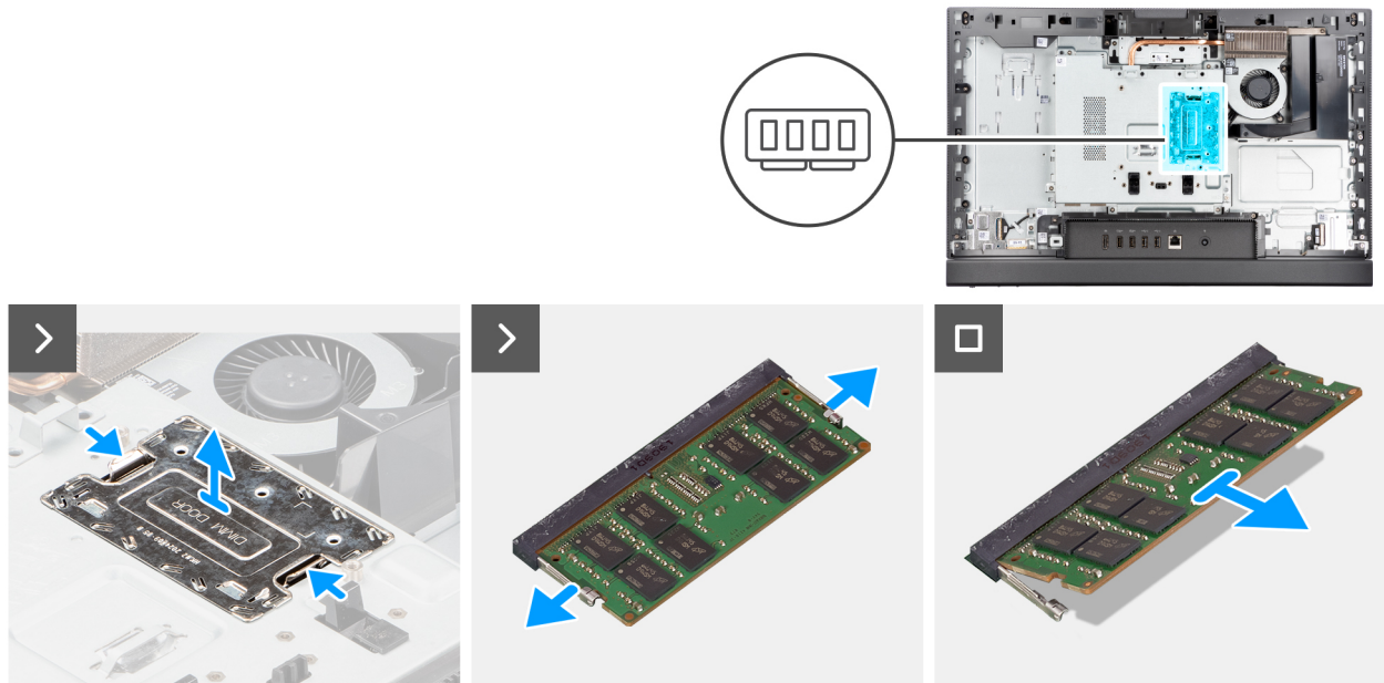
Figure 20. Removing the memory
