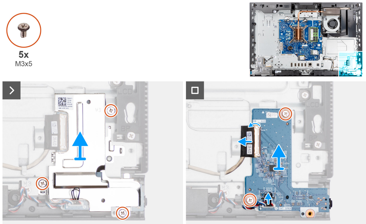
Figure 55. Removing the audio board
