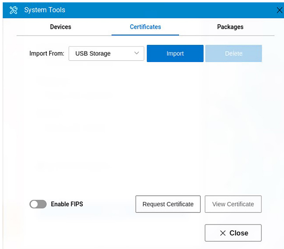
Figure 66. Certificates
