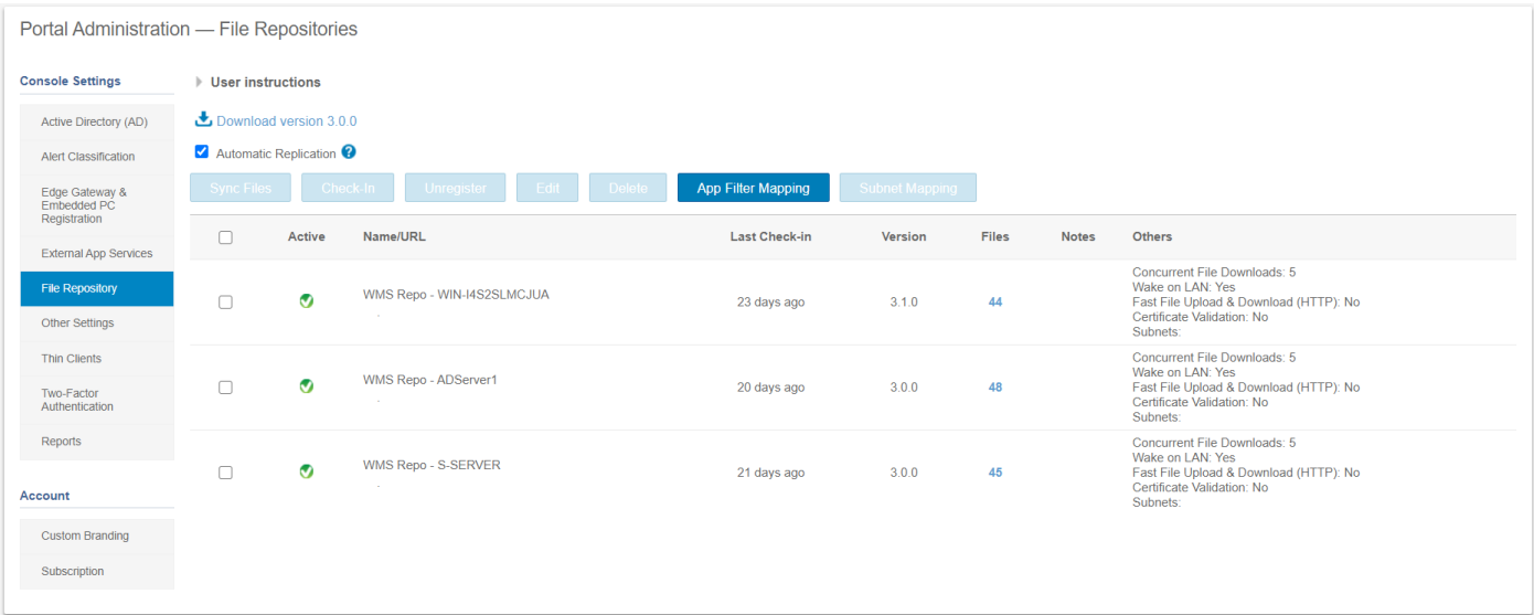
Figure 72. File repository
