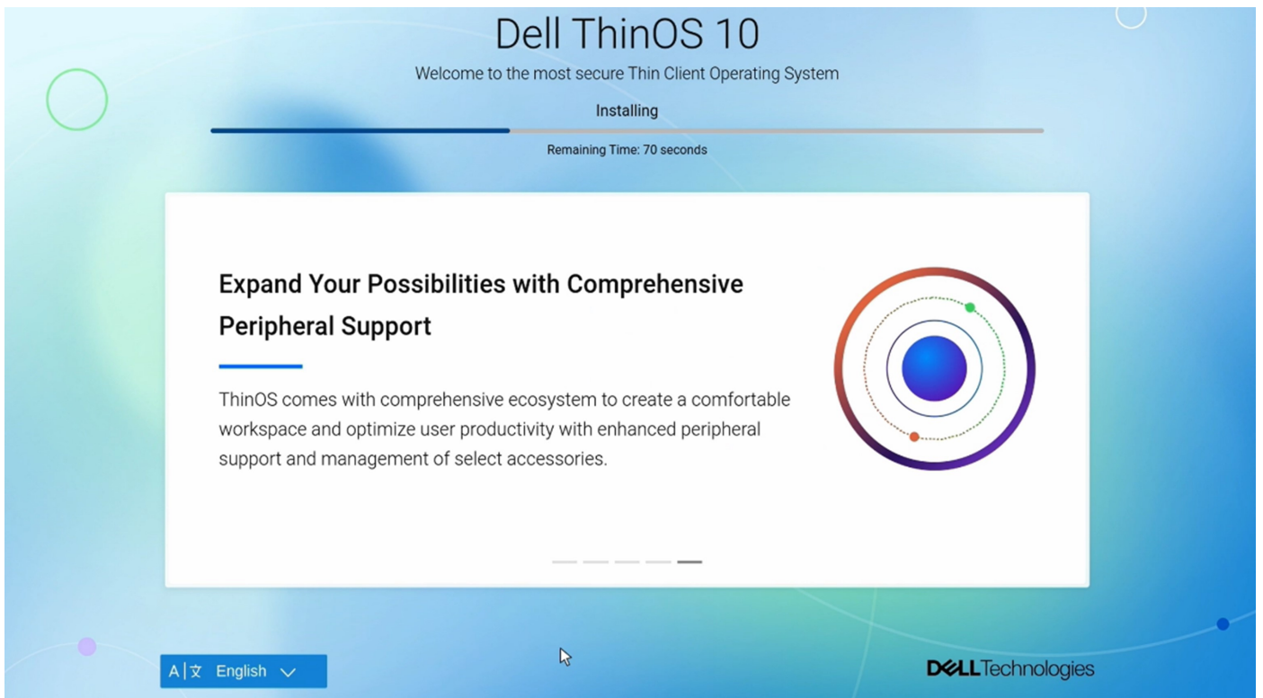
Figure 14. Peripheral support
