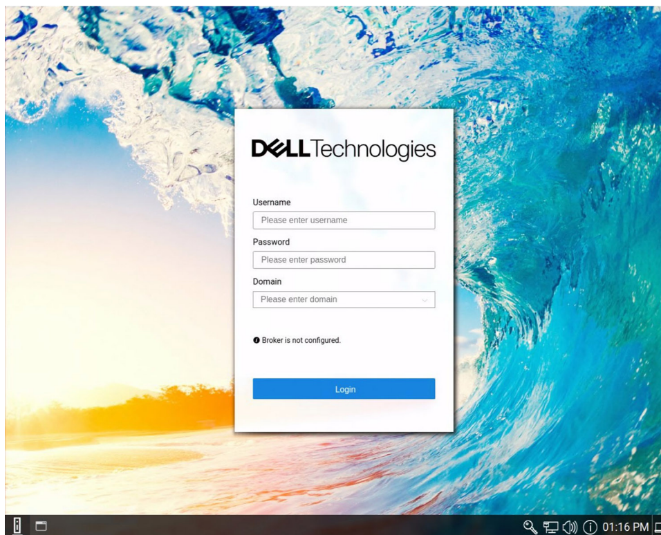
Figure 18. Classic Desktop
