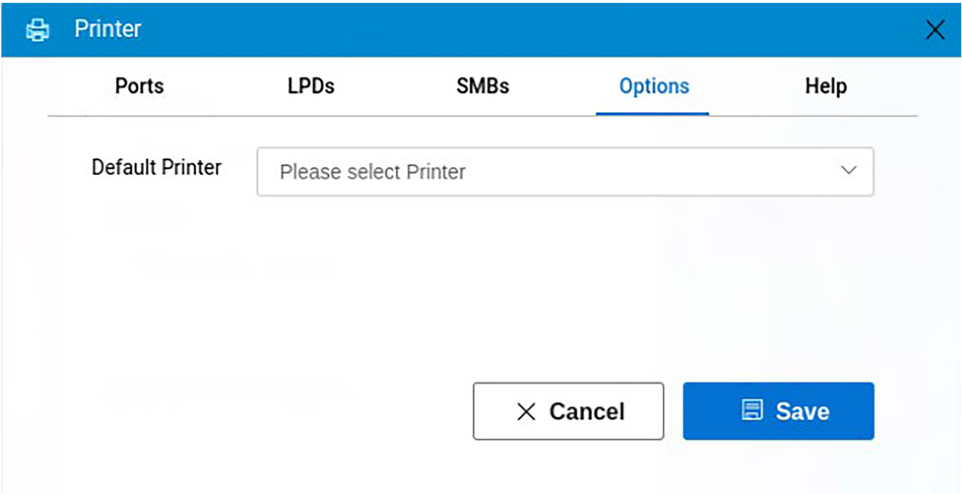
Figure 64. Options
