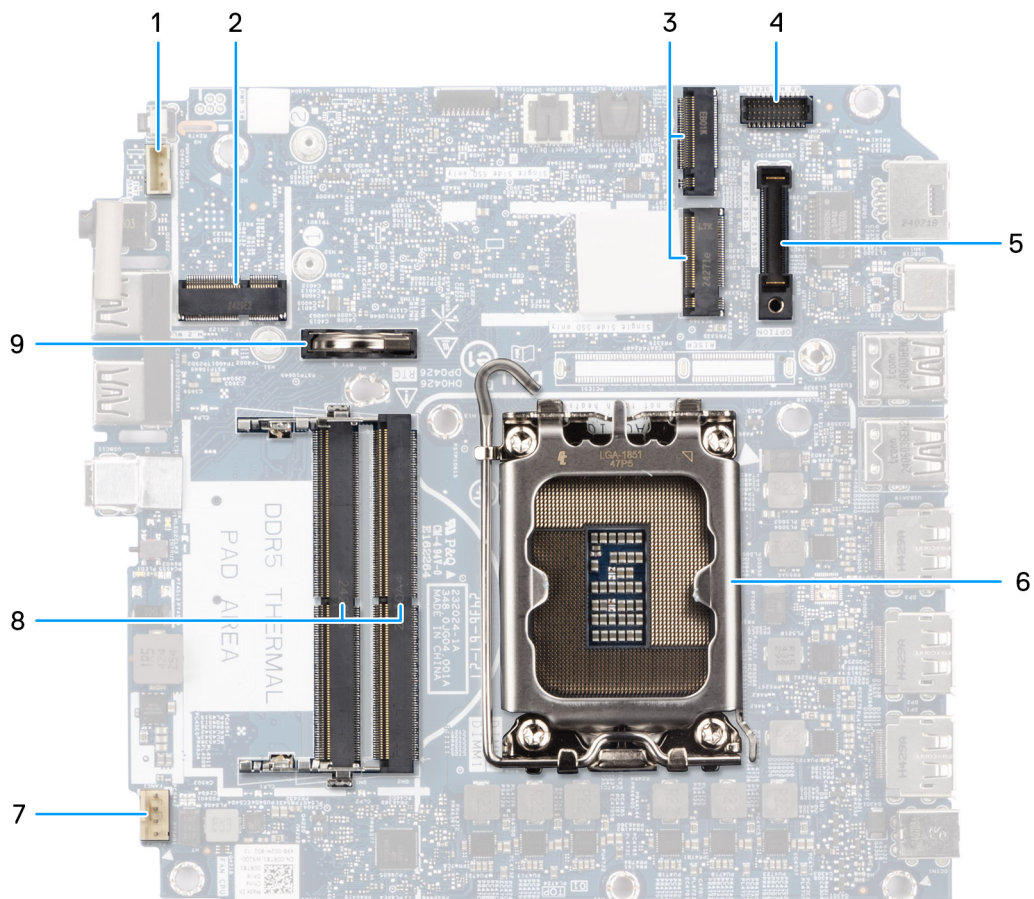
Figure 81. System board connectors
