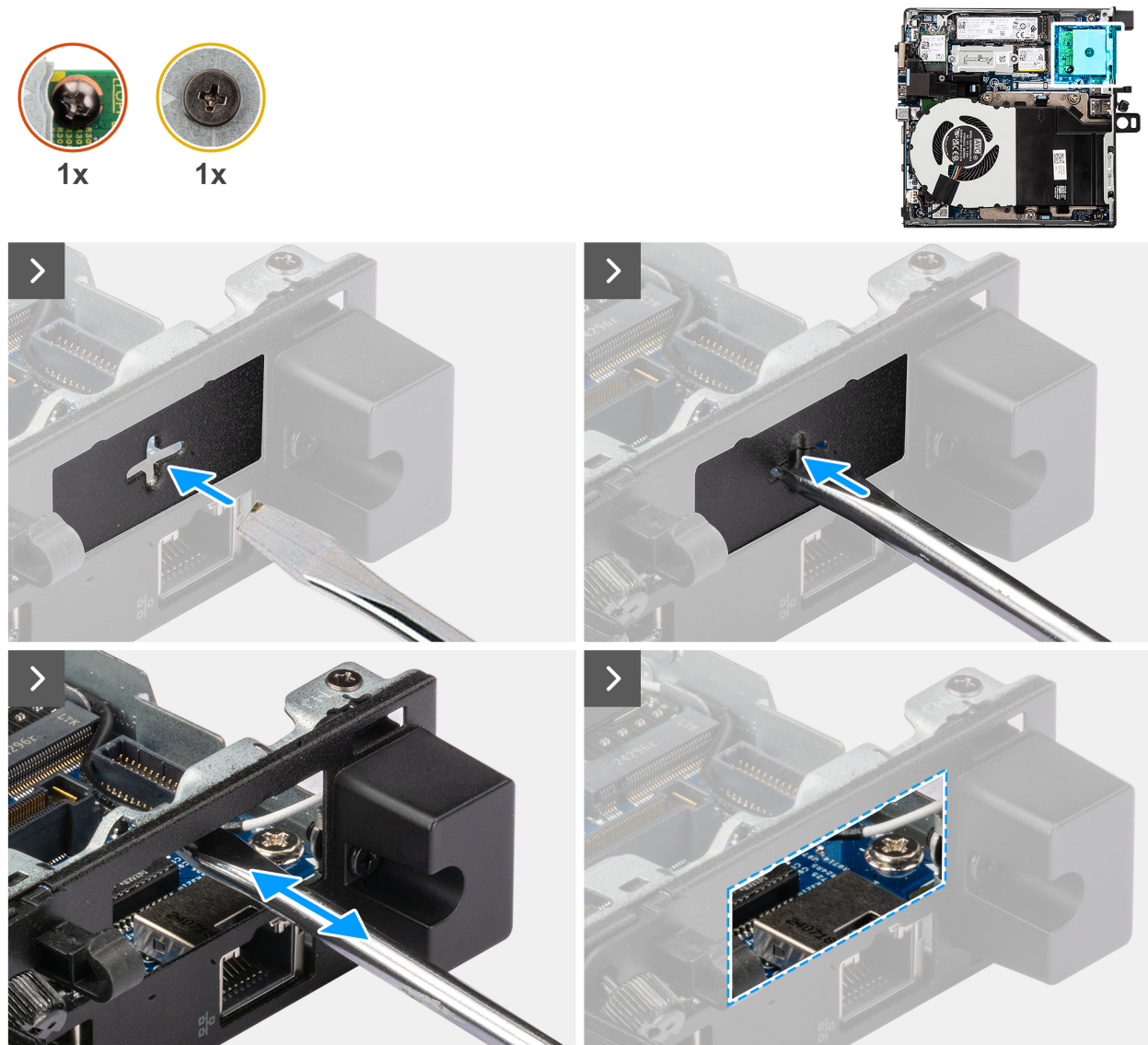
Figure 43. Installing the USB Type-C port module
