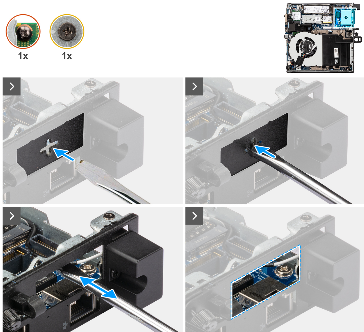
Figure 46. Installing the Thunderbolt port and USB Type-C port module
