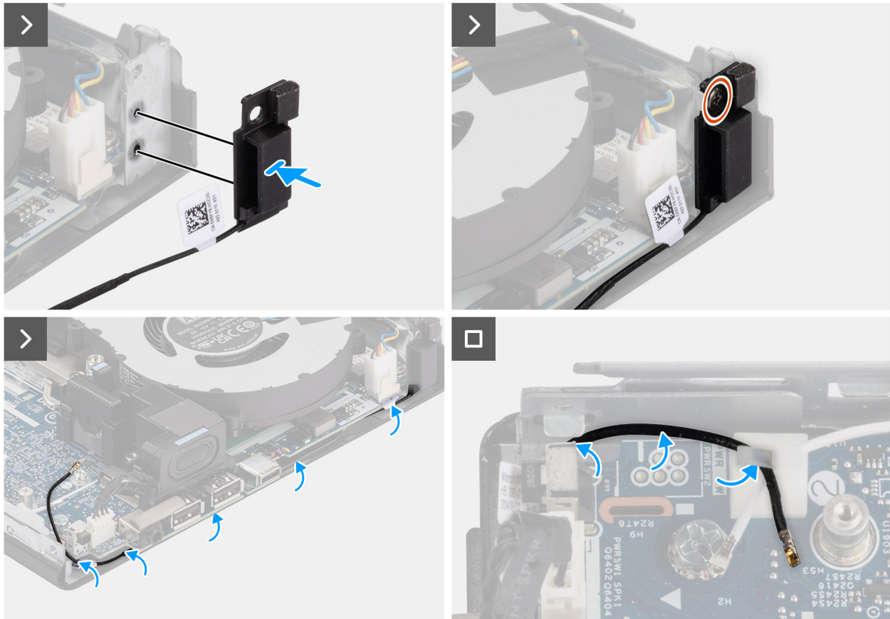
Figure 72. Installing the antenna module (black cable)
