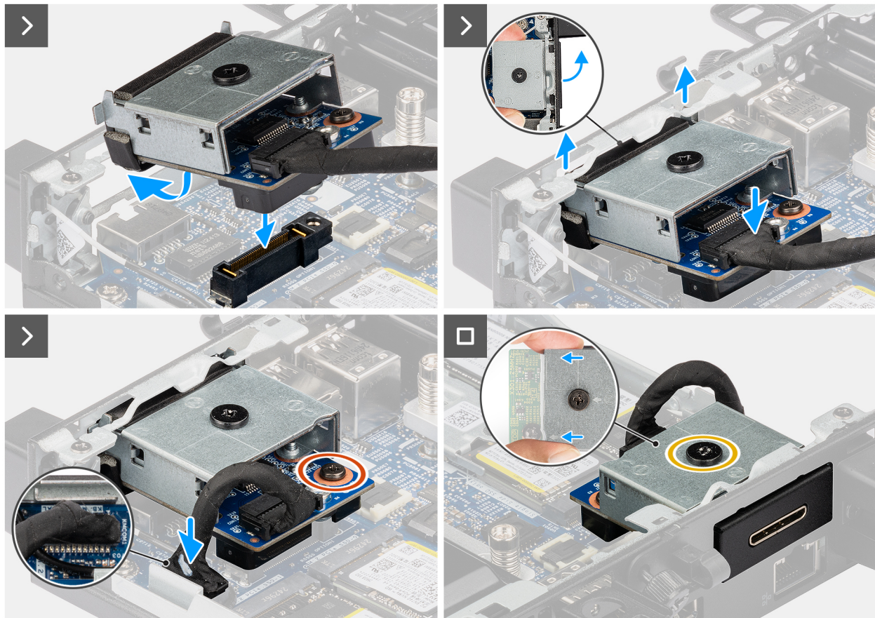
Figure 59. Installing the PS2 port module
