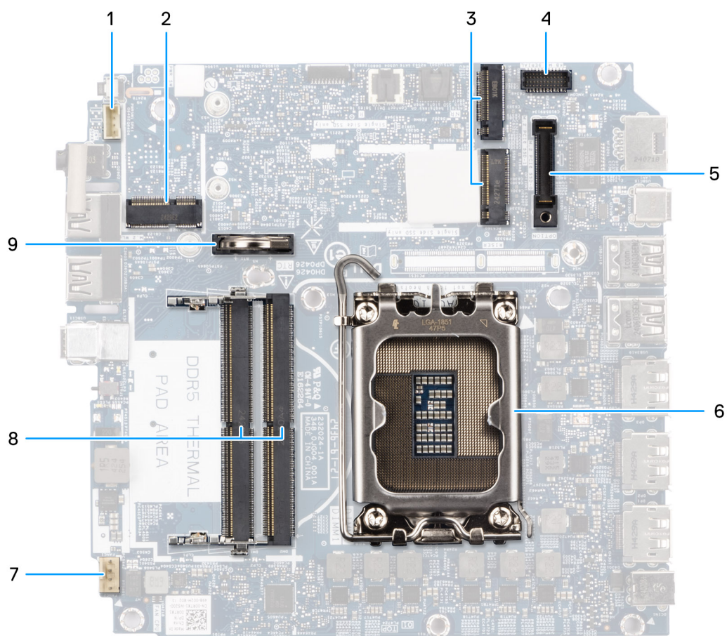
Figure 84. System board connectors
