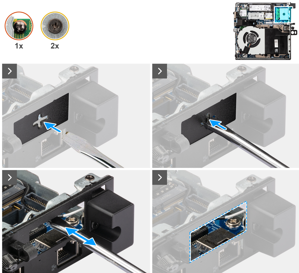
Figure 64. Installing fiber optic port module
