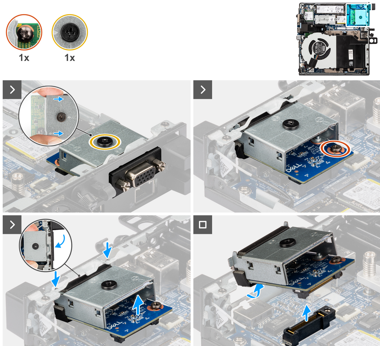
Figure 54. Removing the VGA port module
