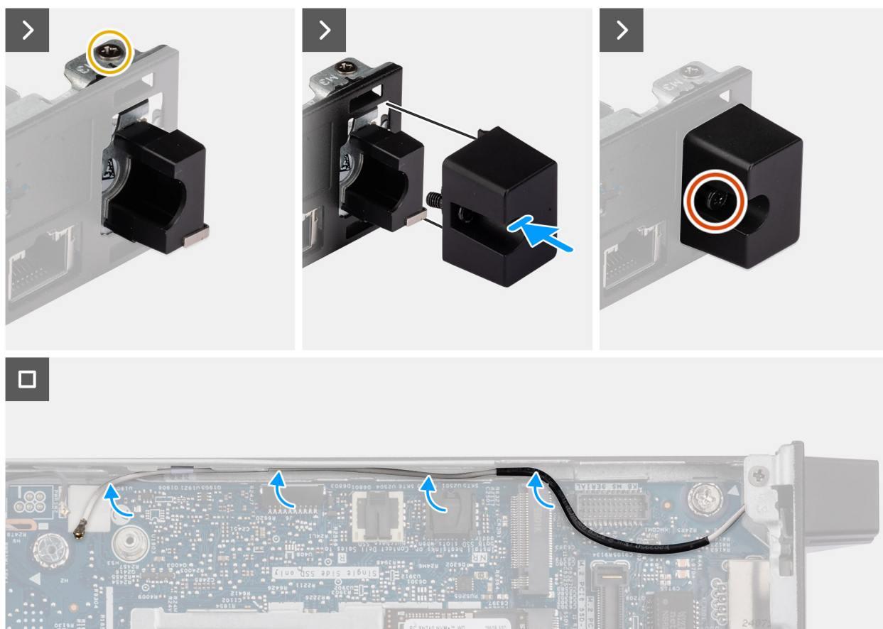
Figure 76. Installing the antenna module (white cable)
