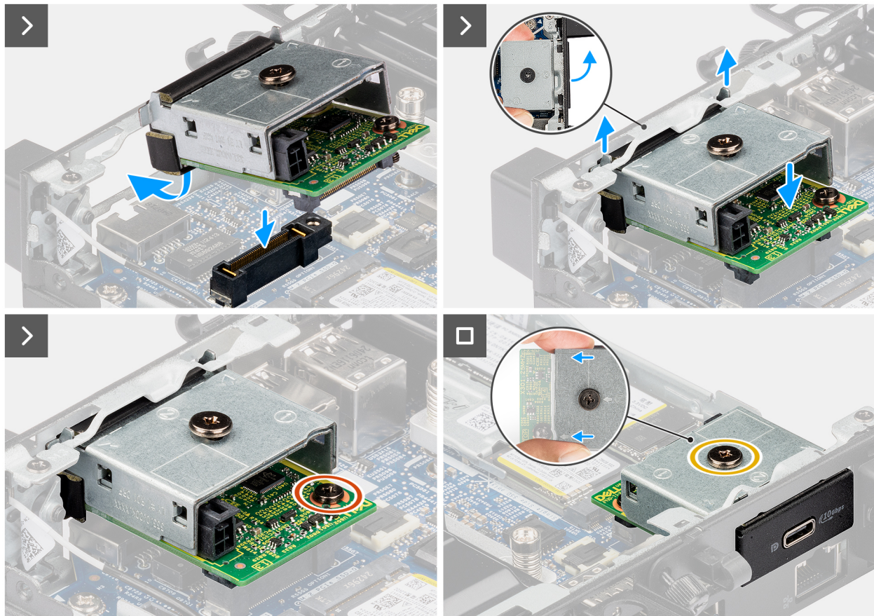
Figure 44. Installing the USB Type-C port module
