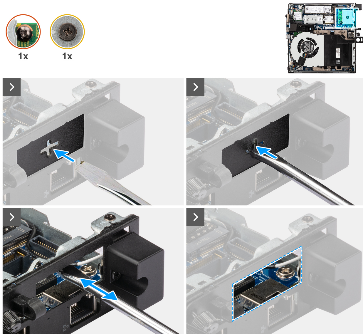
Figure 49. Installing DisplayPort module
