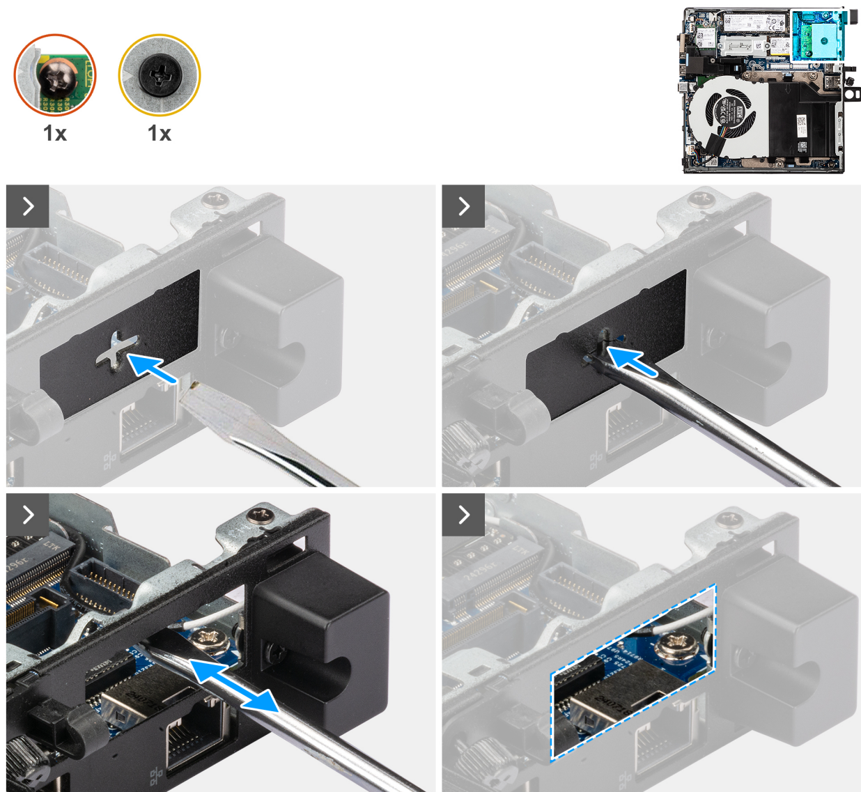
Figure 55. Installing VGA port module
