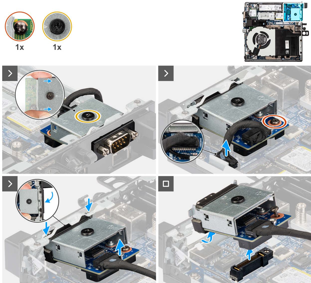
Figure 60. Removing the serial port module
