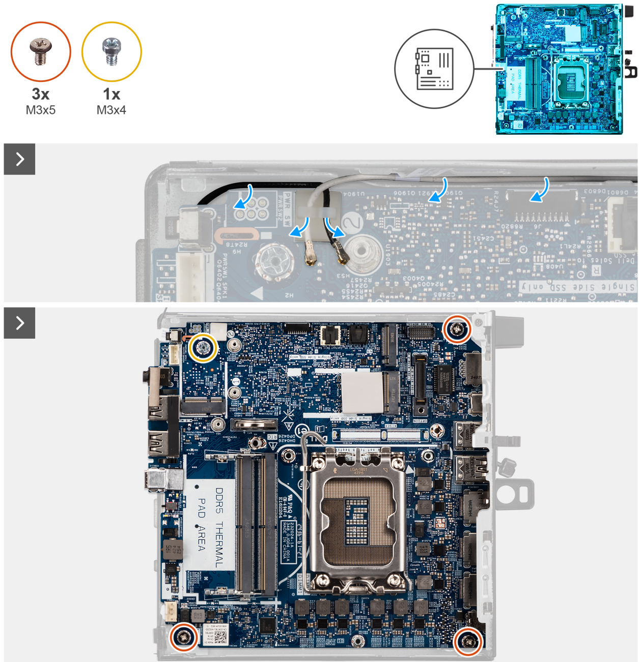
Figure 82. Removing the system board
