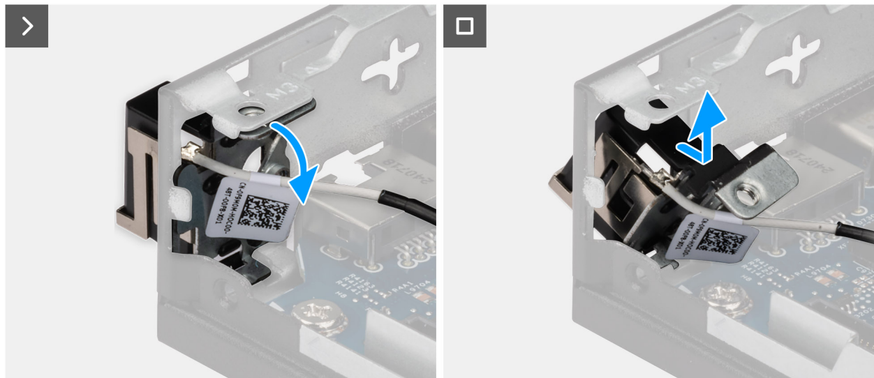
Figure 74. Removing the antenna module (white cable)
