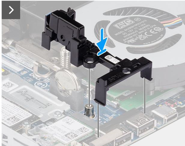
Figure 80. Installing the speaker holder
