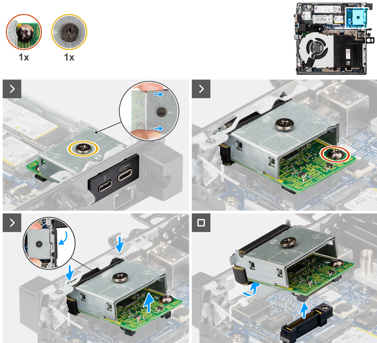
Figure 45. Removing the Thunderbolt port and USB Type-C port module
