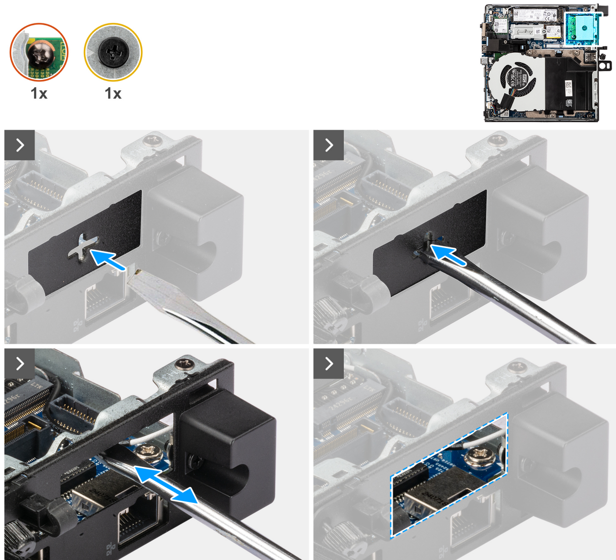
Figure 52. Installing HDMI port module
