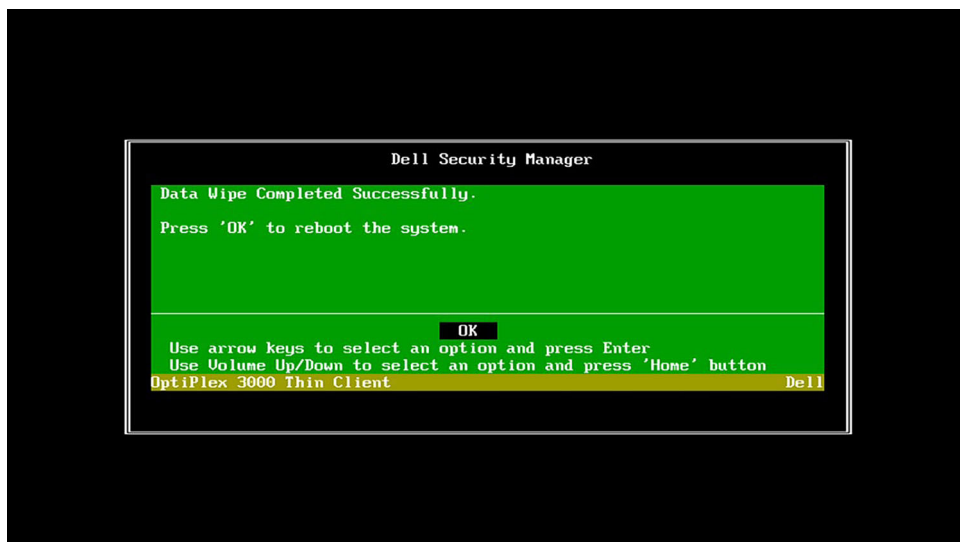
Figure 10. Dell Security Manager screen
