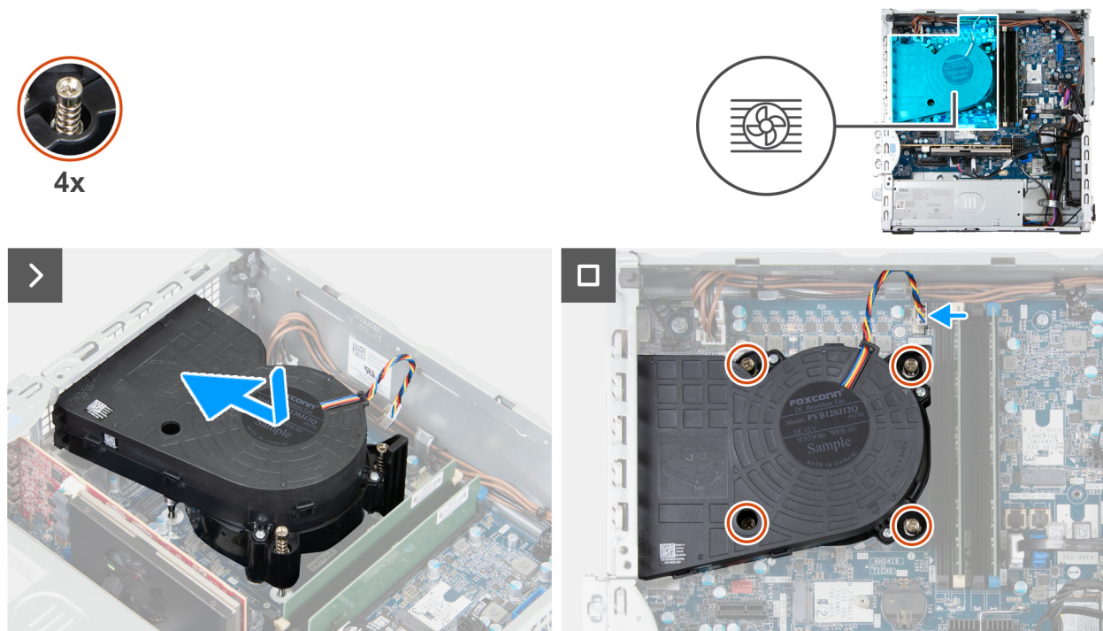
Figure 76. Installing the processor fan and heat-sink assembly (Dell Pro Slim Plus QBS1250)
