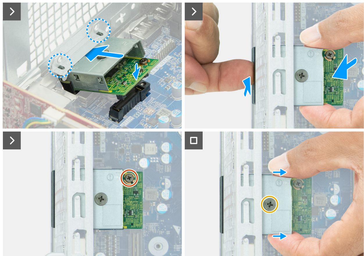
Figure 80. Installing the optional-port module
