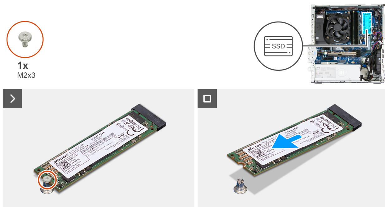
Figure 31. Removing the M.2 2280 solid state drive from slot 2
