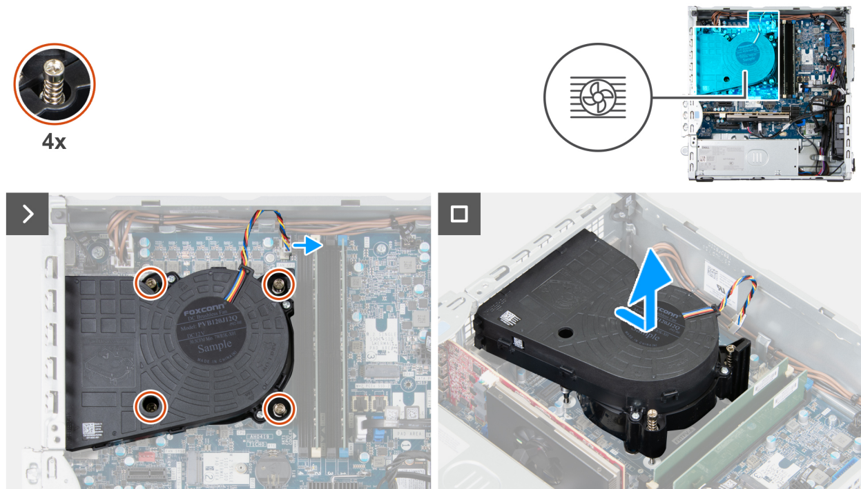
Figure 74. Removing the processor-fan and heat-sink assembly (Dell Pro Slim Plus QBS1250)
