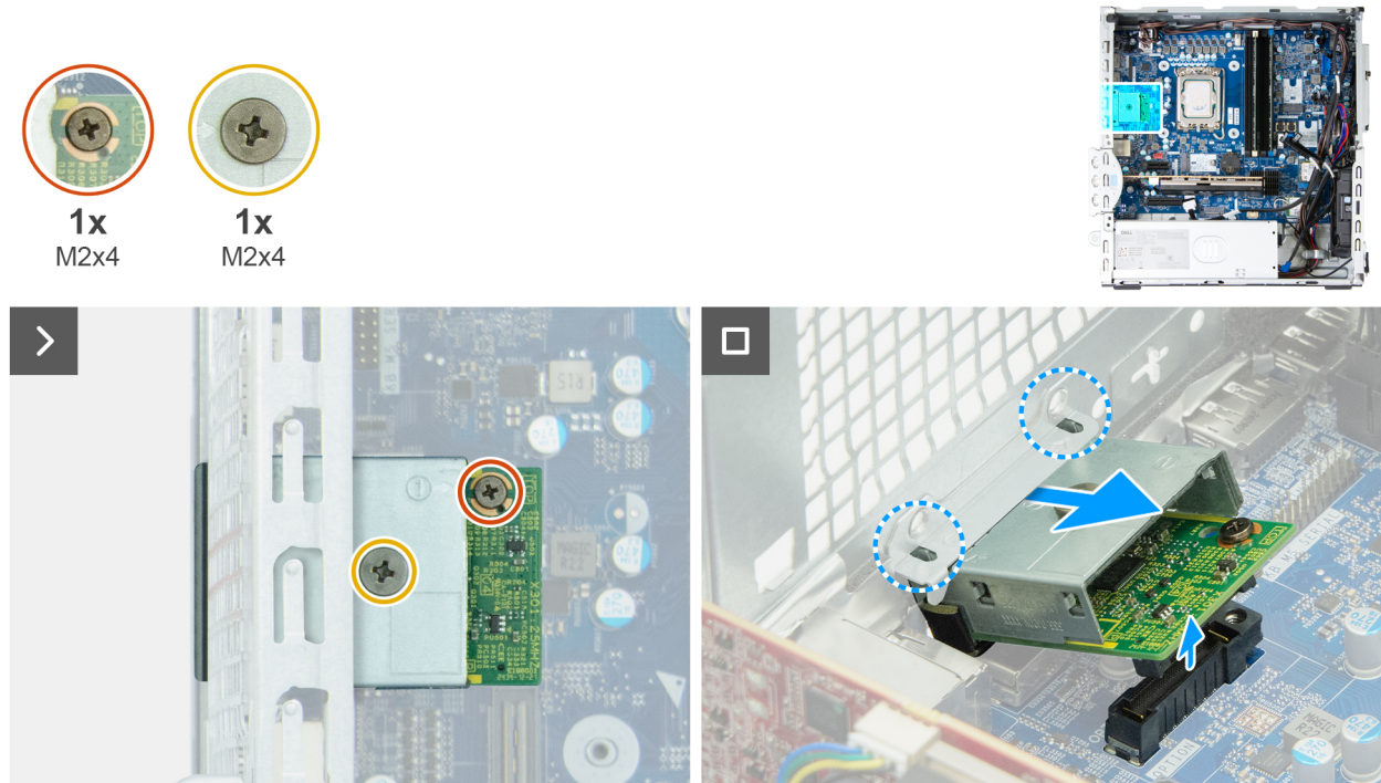
Figure 78. Removing the optional-port module
