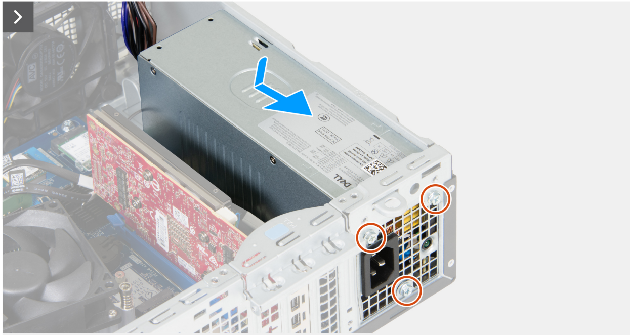
Figure 72. Installing the power-supply unit
