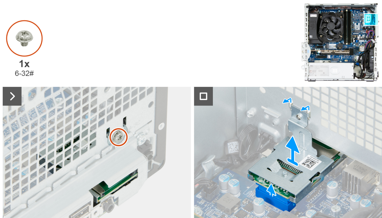
Figure 66. Removing the media-card reader
