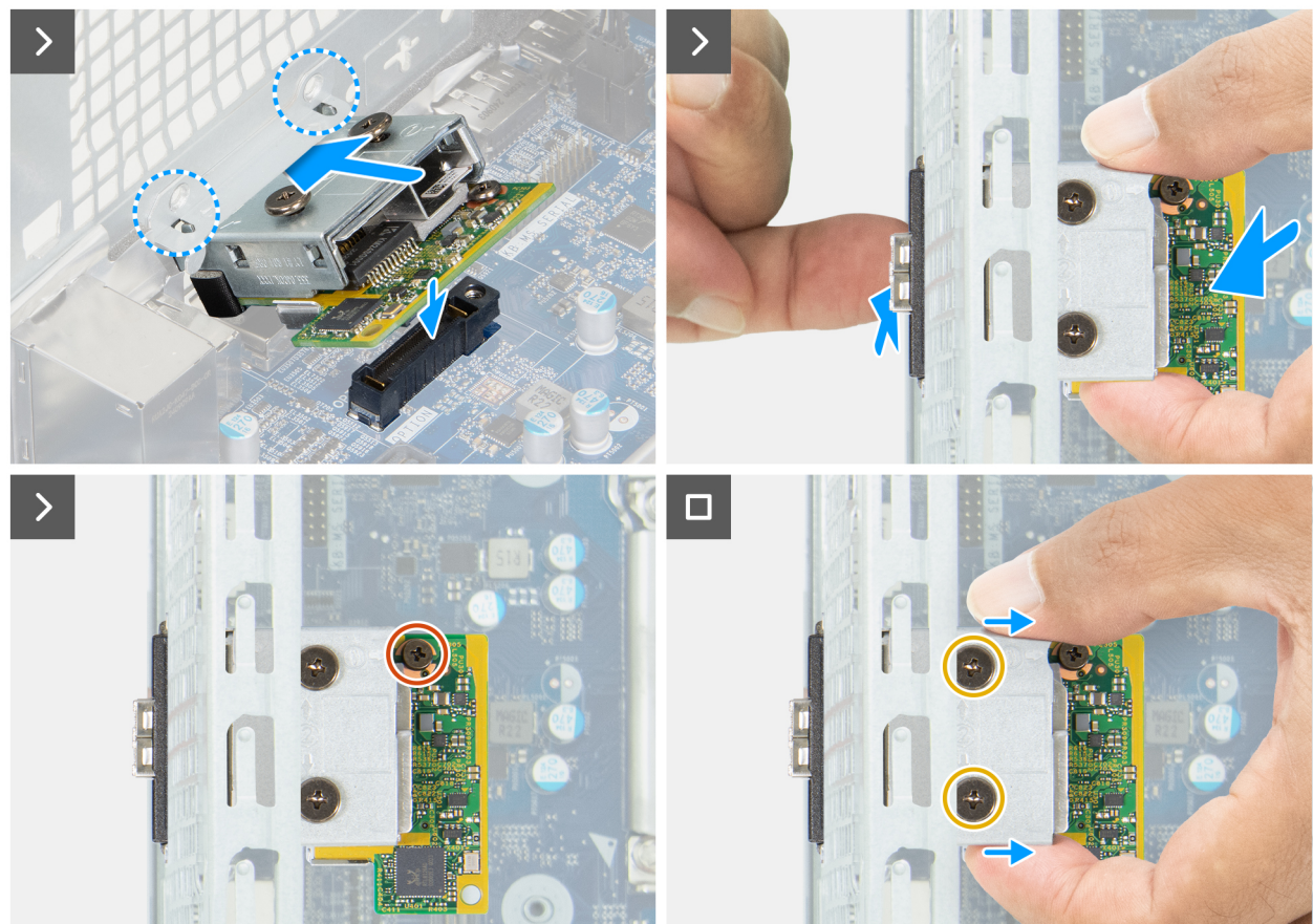
Figure 83. Installing the fiber-optic port module
