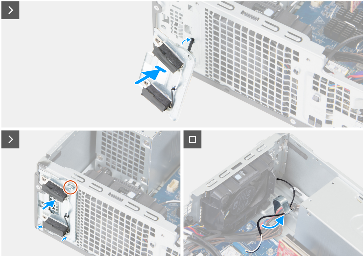
Figure 69. Installing the antenna modules
