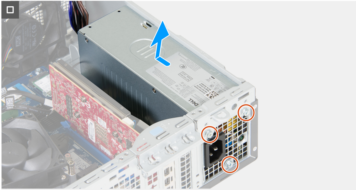
Figure 71. Installing the power-supply unit
