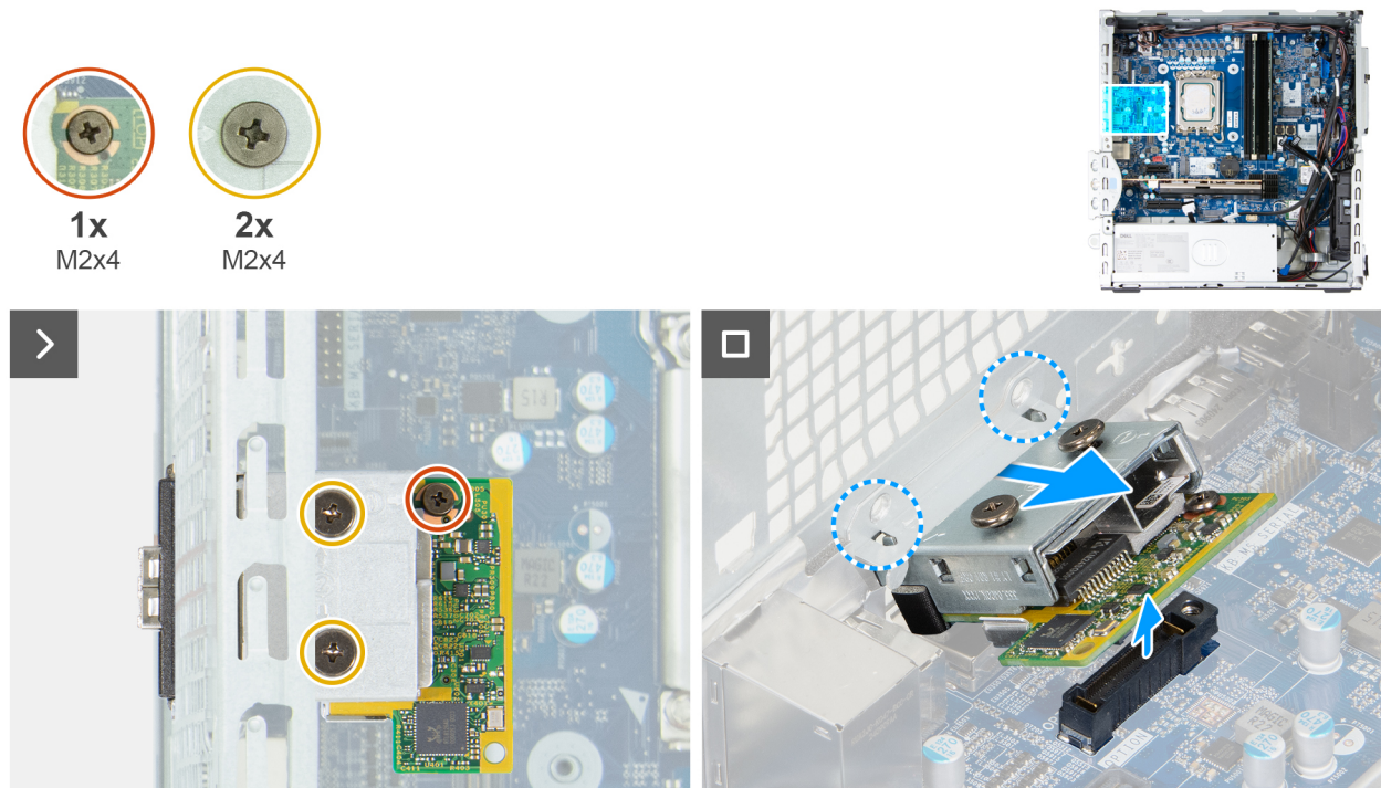
Figure 81. Removing the fiber-optic port module
