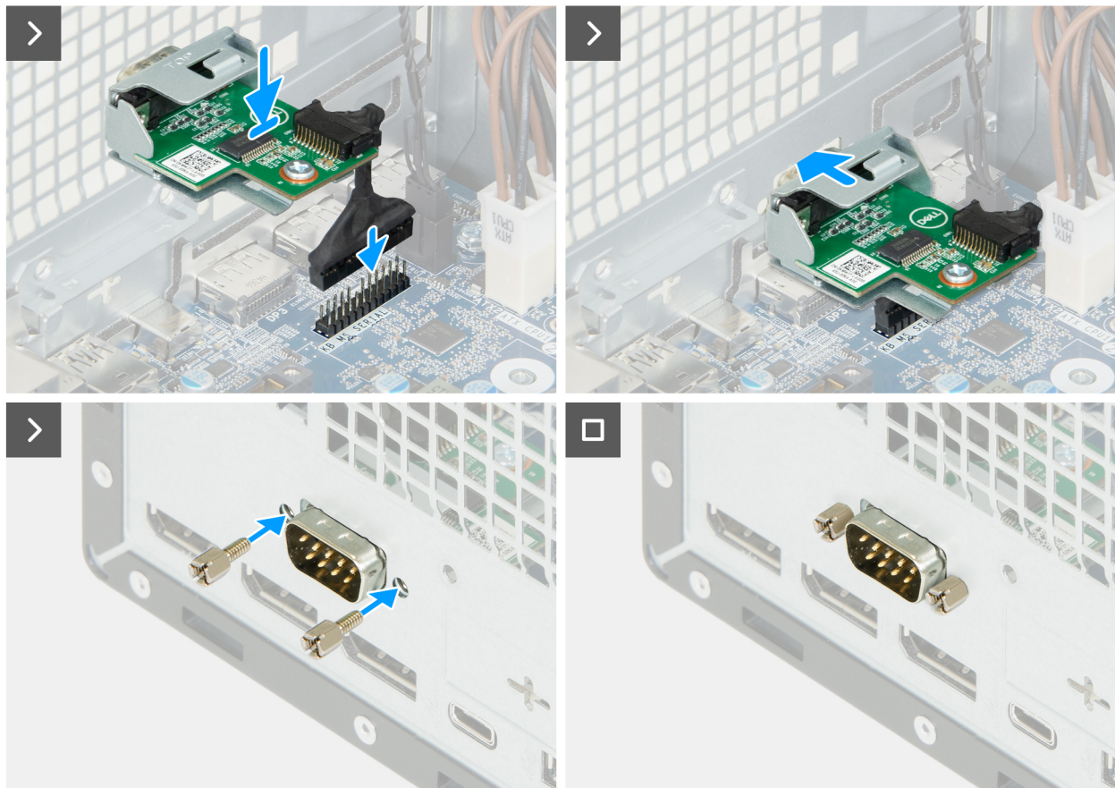
Figure 65. Installing the serial-port module
