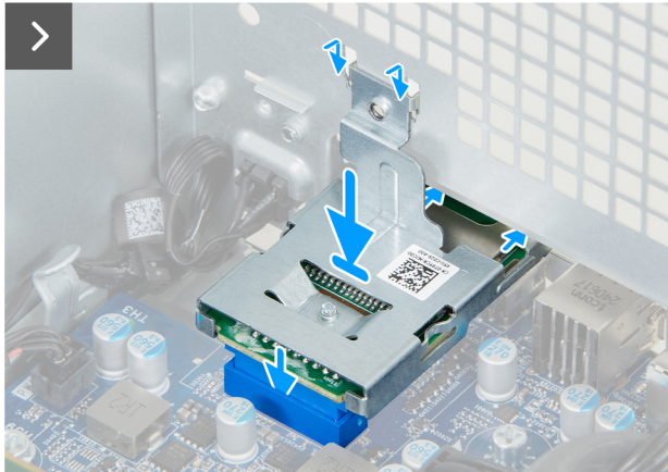
Figure 67. Installing the media-card reader
