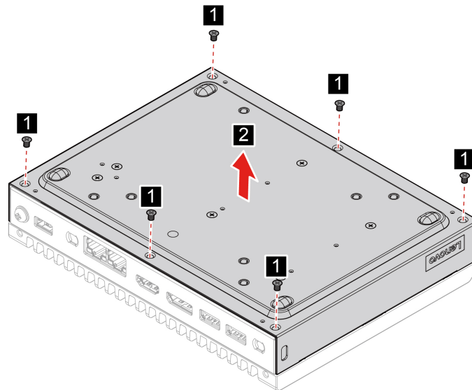
Figure 14: Remove bottom cover - SE10n Gen2 Type 2
