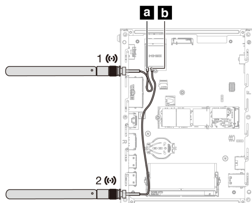
Figure 9: Antenna location and cable connection - SE10n Gen2 Type 2
