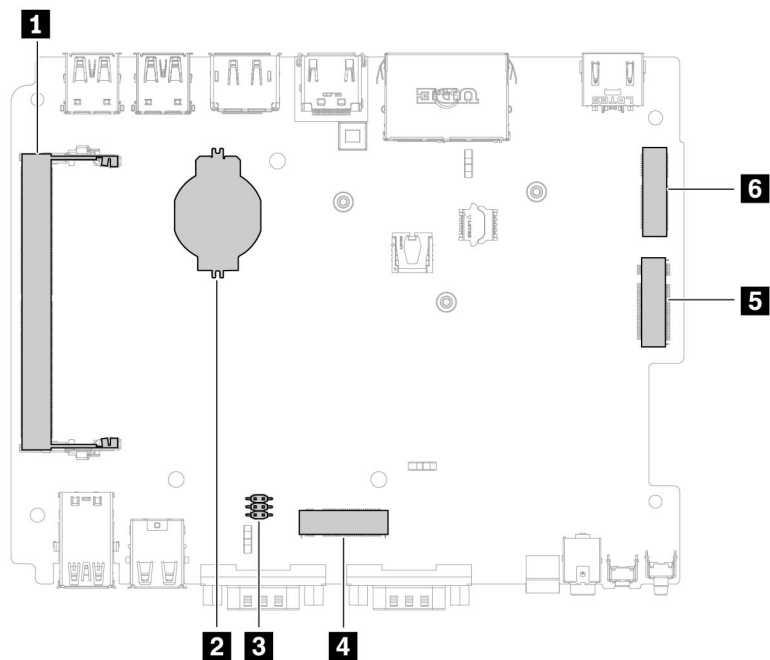
Figure 10: System board — front view
