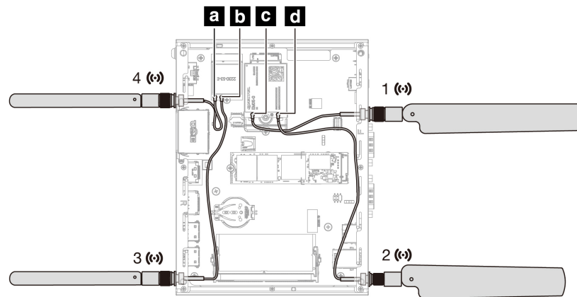
Figure 8: Antenna location and cable connection - SE10n Gen2 Type 1
