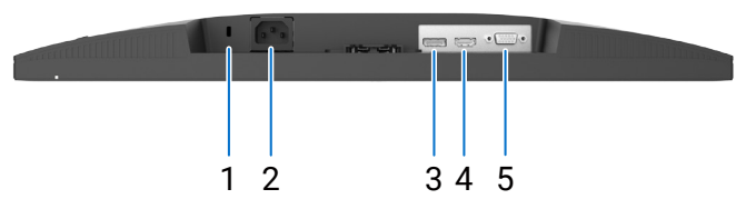
Figure 4. Bottom view
