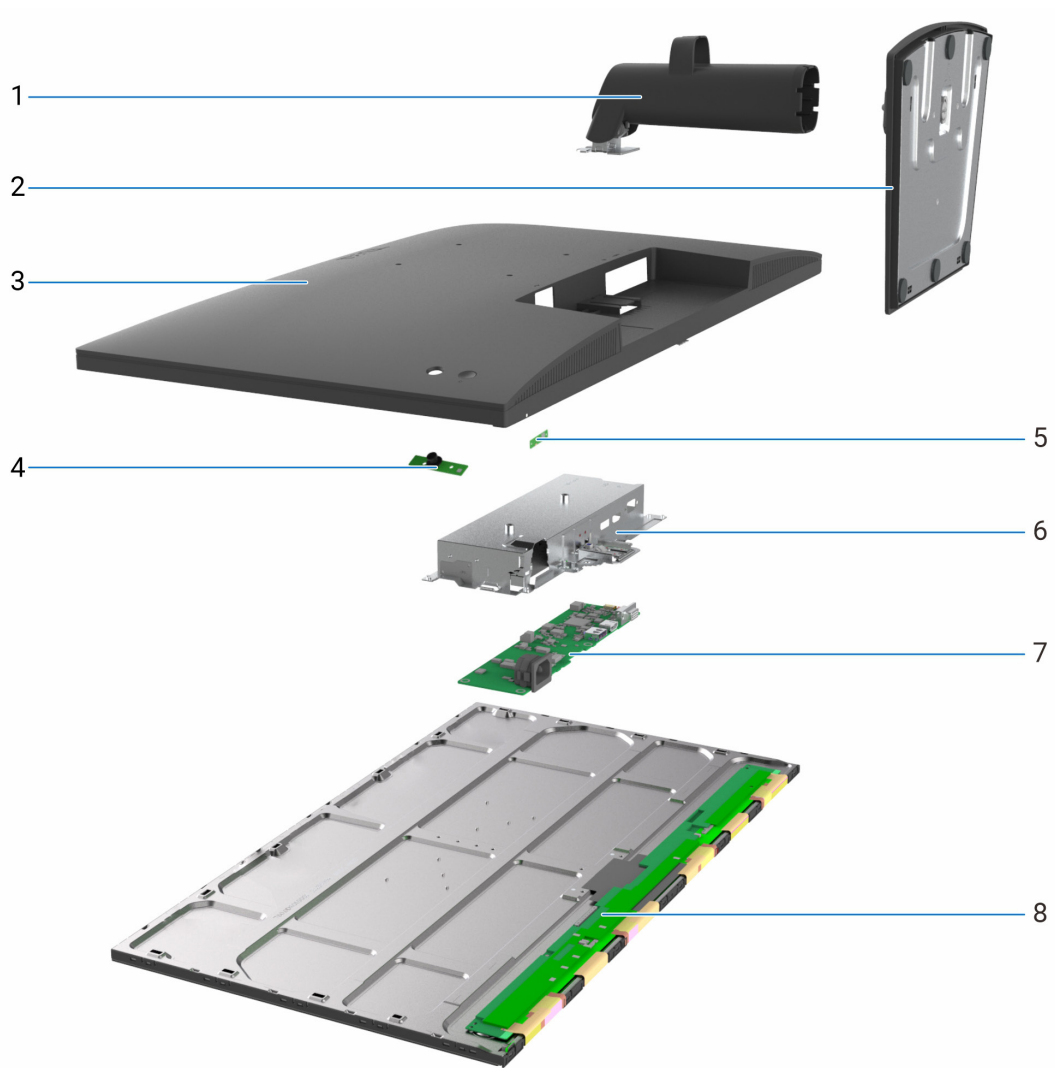
Figure 5. Major Components of E2226H monitor
