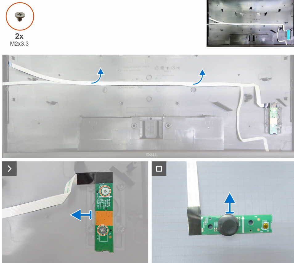
Figure 13. Removing the keypad board
