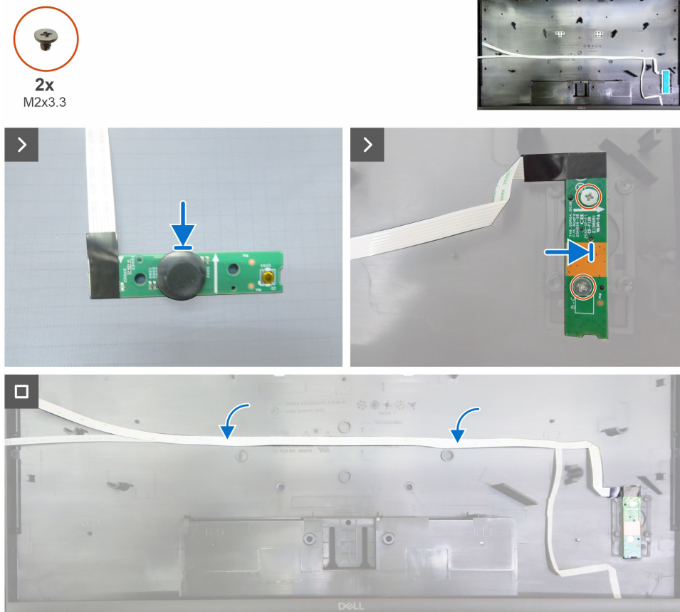
Figure 14. Installing the keypad board
