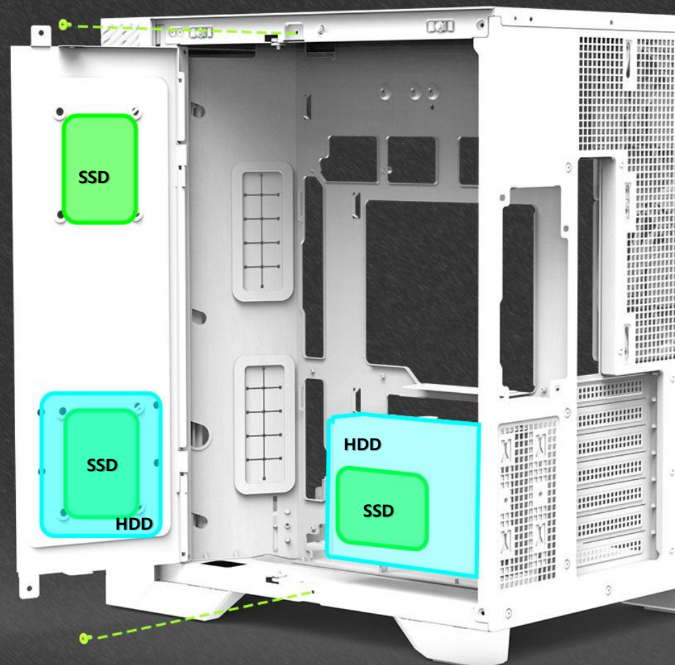
Storage Device Installation 1 x Combo(2.5" or 3.5"), 2 x 2.5", 2 x 3.5"
