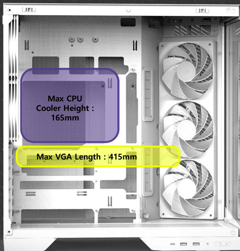
CPU Cooler Maximum Height 165mm
