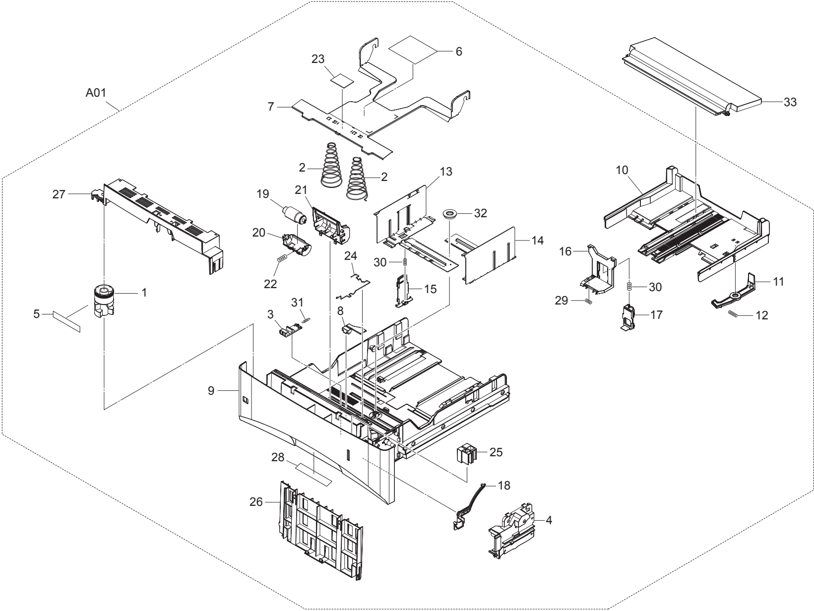
FIG. 4 Paper Cassette (FS-2000D)
