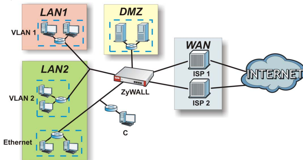
Figure 375 Example: Zones
