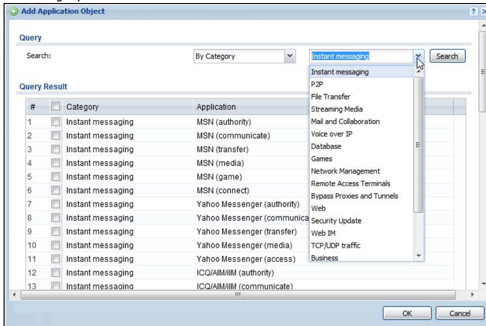
Figure 403 Configuration > Object > Application > Application > Add Application Rule > Add By Category
