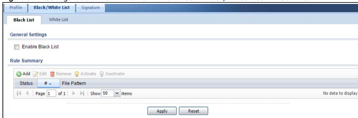
Figure 347 Configuration > UTM Profile > Anti-Virus > Black/White List > Black List
