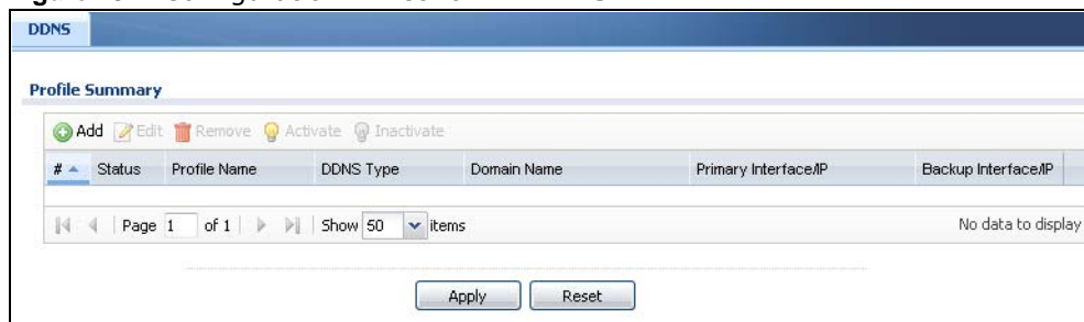
Figure 194 Configuration > Network > DDNS
