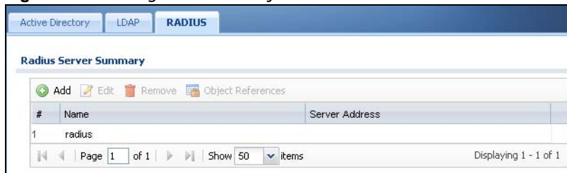
Figure 426 Configuration > Object > AAA Server > RADIUS
