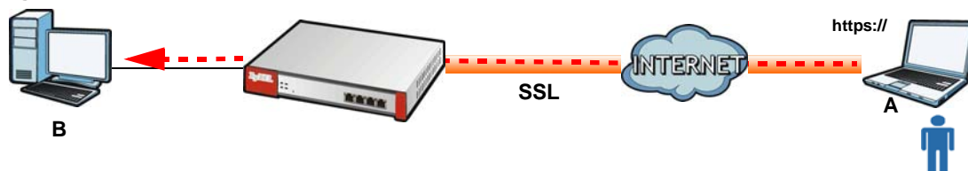
Figure 442 SSL-protected Remote Management
