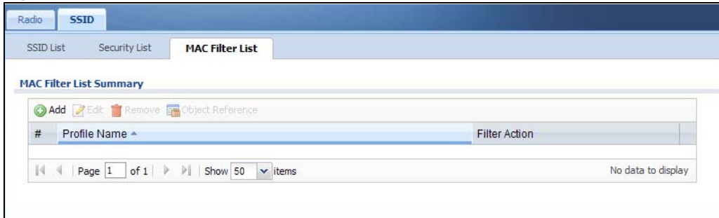
Figure 395 Configuration > Object > AP Profile > SSID > MAC Filter List
