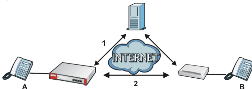
Figure 206 SIP ALG Example
