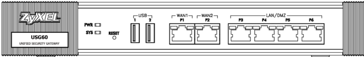
Figure 35 USG60 / USG60W Front Panel
