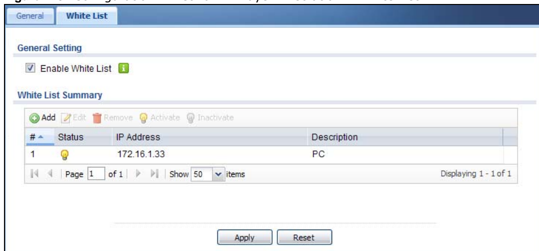
Figure 228 Configuration > Network > Layer 2 Isolation > White List
