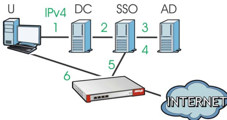
Figure 238 SSO Overview
