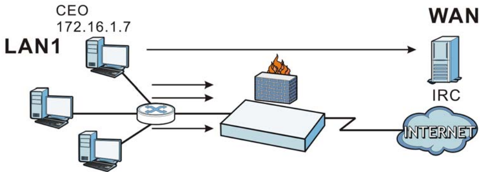
Figure 256 Limited LAN to WAN IRC Traffic Example
