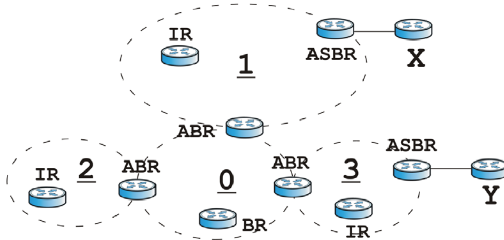
Figure 189 OSPF: Types of Routers
