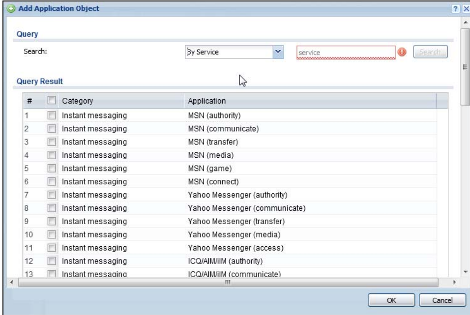
Figure 404 Configuration > Object > Application > Application > Add Application Rule > Add By Service
