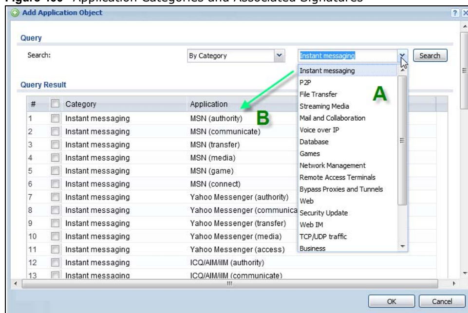
Figure 400 Application Categories and Associated Signatures
