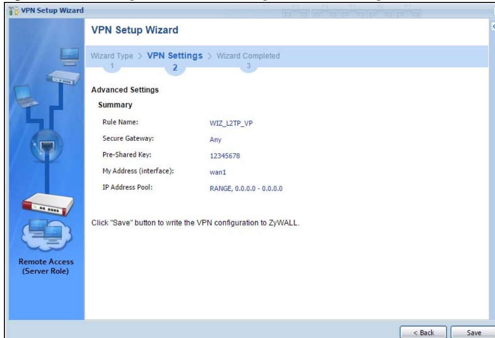
Figure 74 VPN Settings for L2TP VPN Settings Advanced Settings Wizard: Summary
