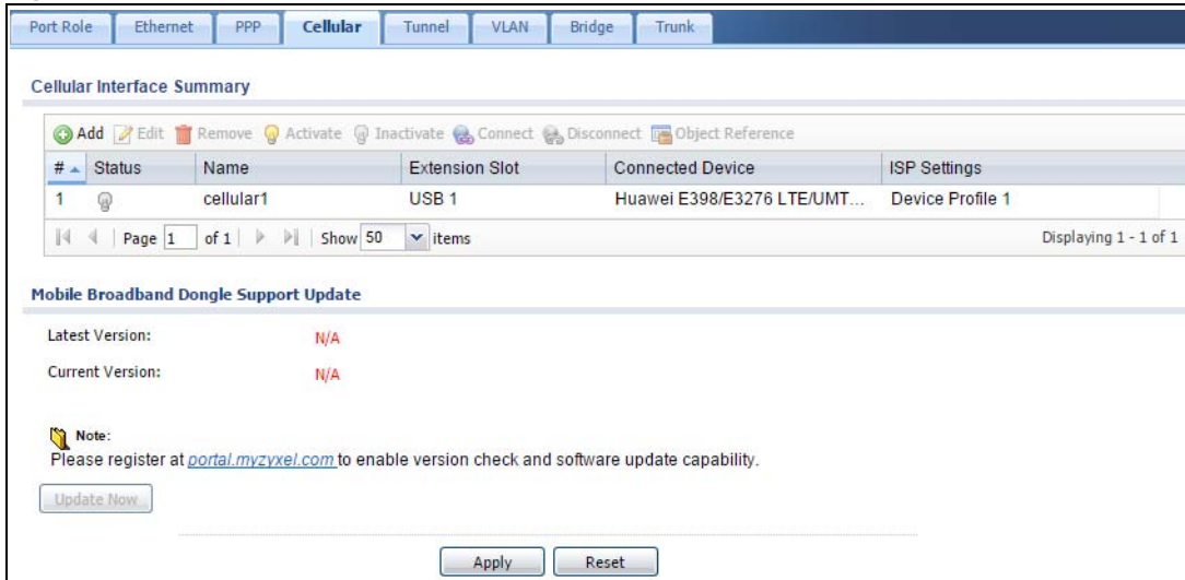
Figure 158 Configuration > Network > Interface > Cellular
