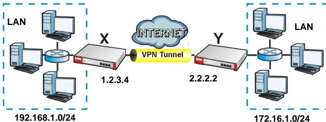
Figure 275 Site-to-site IPSec VPN Example
