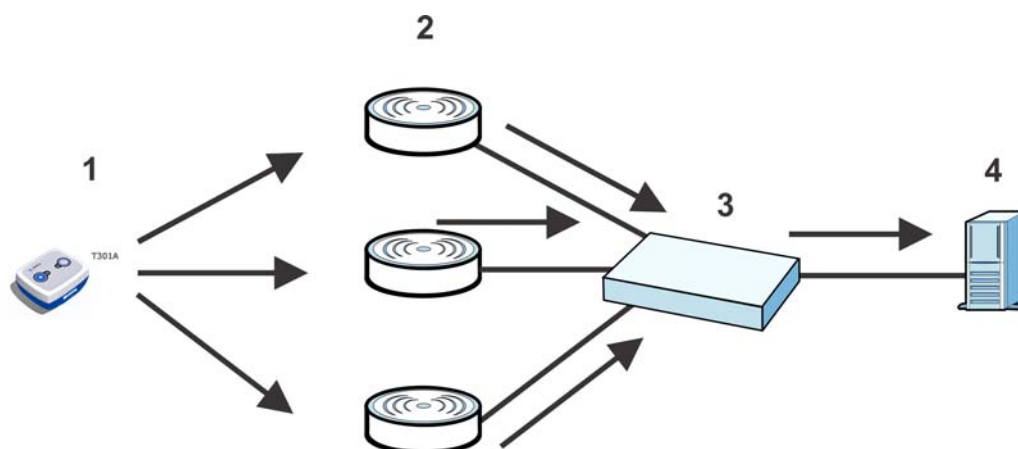
Figure 240 RTLS Example
