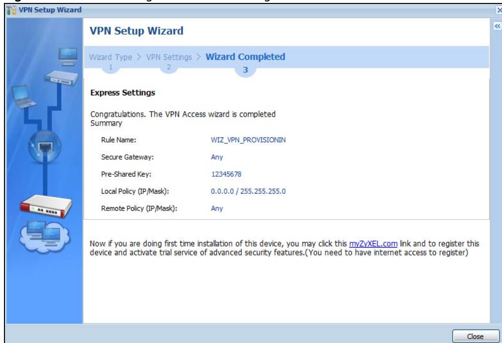
Figure 70 VPN for Configuration Provisioning Advanced Wizard: Finish
