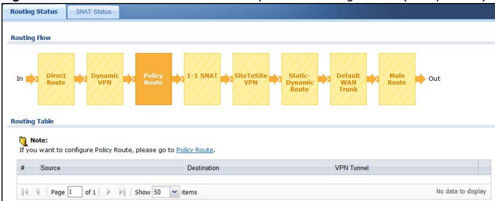
Figure 533 Maintenance > Packet Flow Explore > Routing Status (Policy Route)
