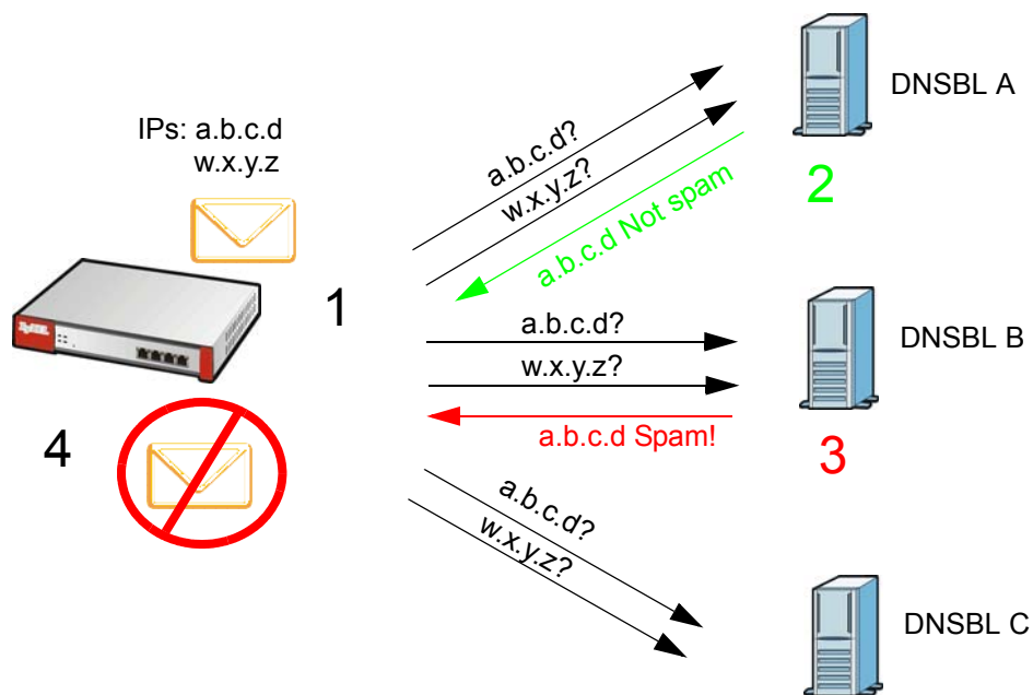
Figure 360 Conflicting DNSBL Replies Example
