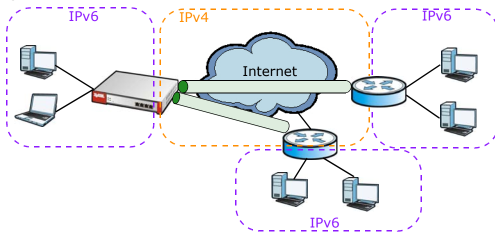
Figure 163 6to4 Tunnel
