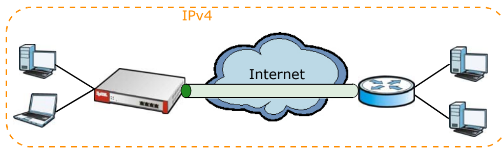
Figure 160 GRE Tunnel Example
