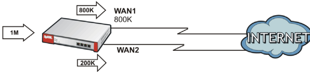
Figure 176 Spillover Algorithm Example
