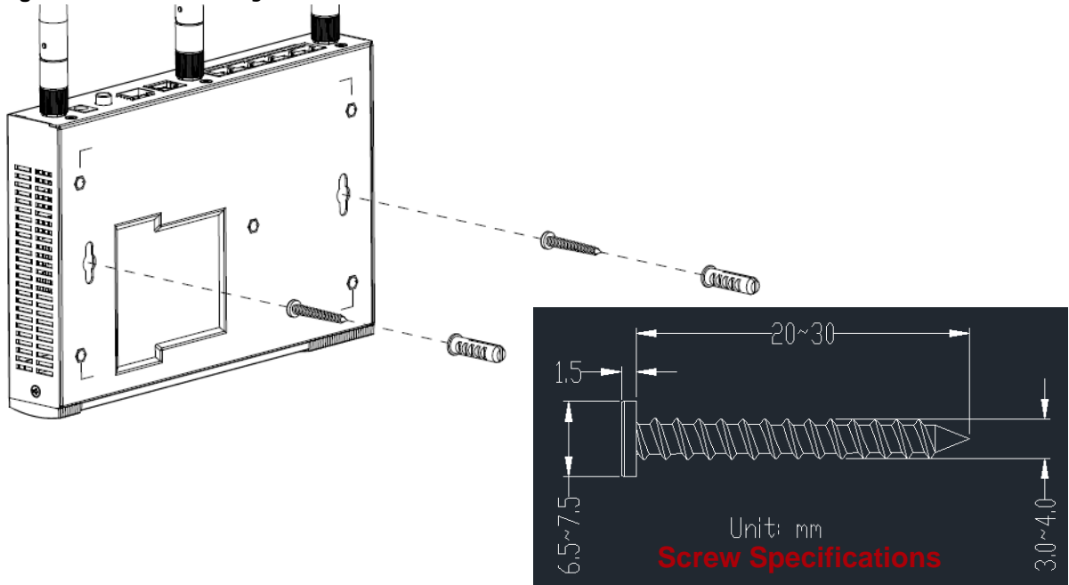
Figure 40 Wall Mounting
