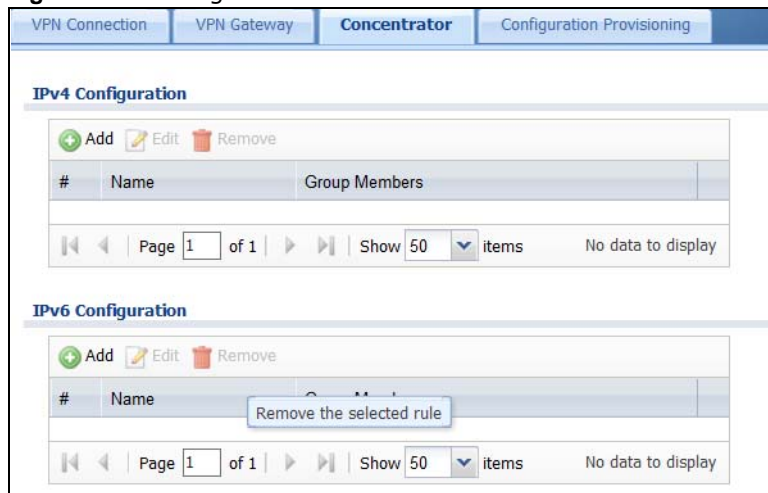
Figure 266 Configuration > VPN > IPsec VPN > Concentrator
