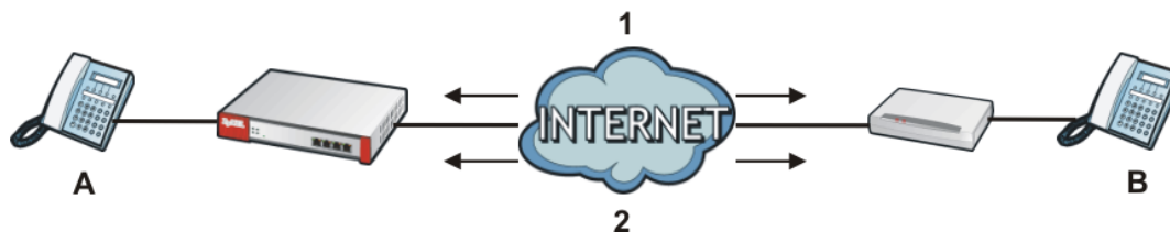
Figure 207 H.323 ALG Example
