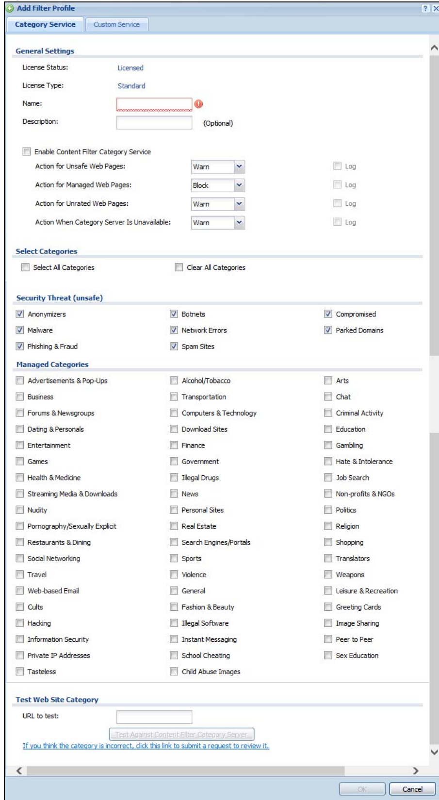
Figure 328 Content Filter > Profile > Add Filter Profile > Category Service
