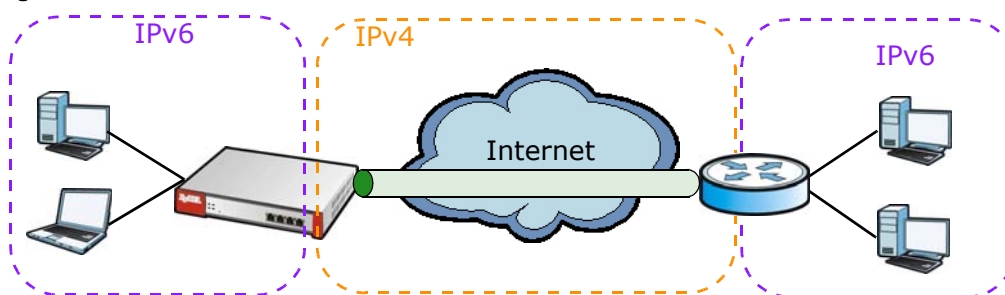
Figure 162 IPv6-in-IPv4 Tunnel
