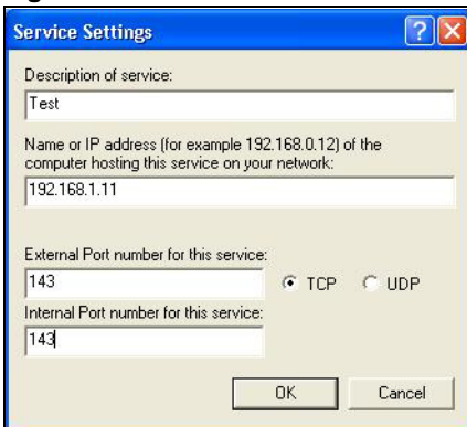
Figure 215 Internet Connection Properties: Advanced Settings: Add
