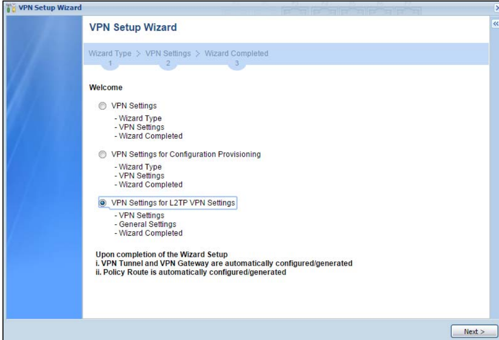
Figure 71 VPN Settings for L2TP VPN Settings Wizard: L2TP VPN Settings
