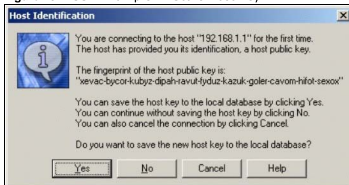
Figure 487 SSH Example 1: Store Host Key
