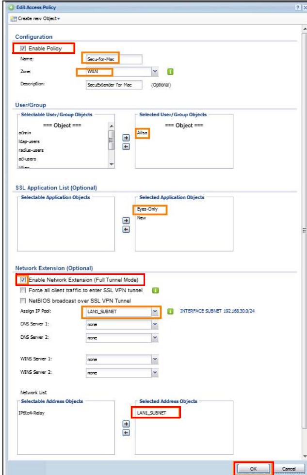
Figure 283 Create an SSL VPN Access Privilege Policy
