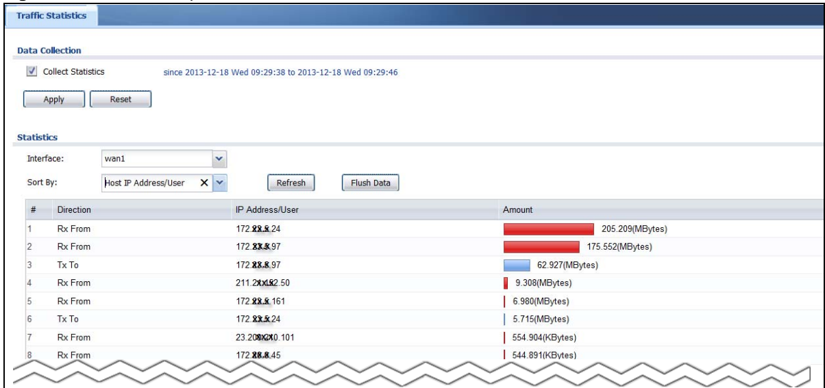
Figure 97 Monitor > System Status > Traffic Statistics
