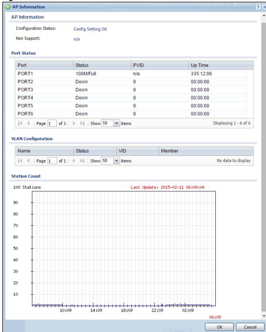
Figure 109 Monitor > Wireless > AP Information > AP List > More Information
