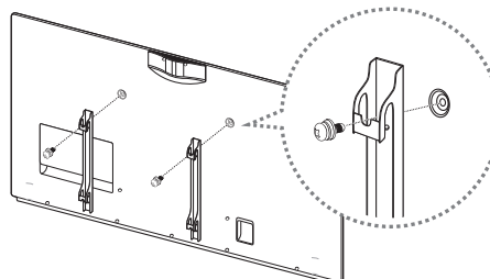
Case B. Installing another company's Wall-Mount
