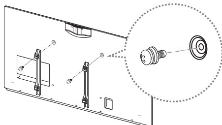
Case A. Installing the SAMSUNG Wall-Mount
