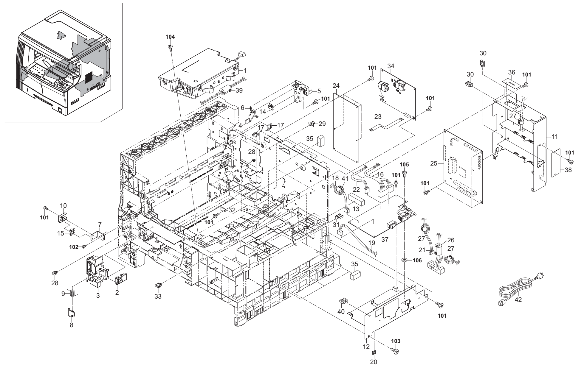
FIG. 12 Electrical Components
