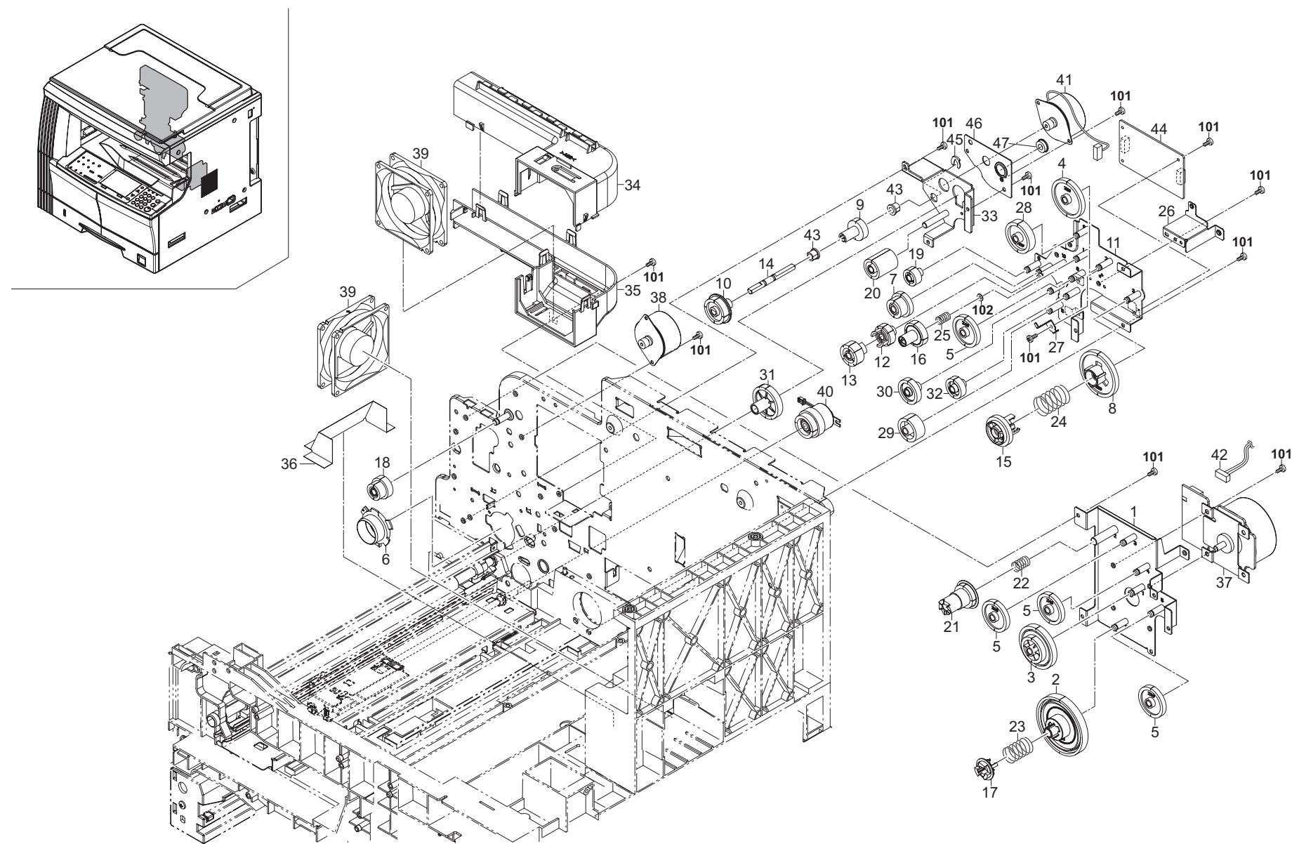
FIG. 11 Driving & Cooling
