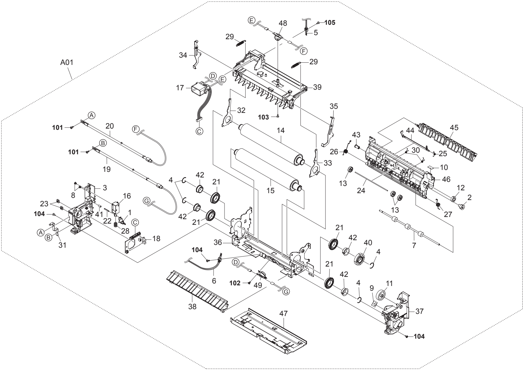
FIG. 6 Fuser Unit (16/17ppm EUR/USA)
