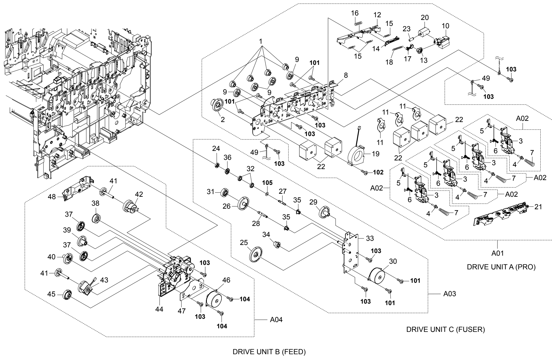
FIG. 3 Drive Units
