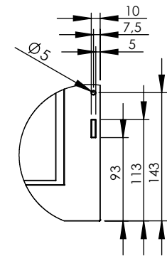
DETAIL A SCALE 1 : 6
