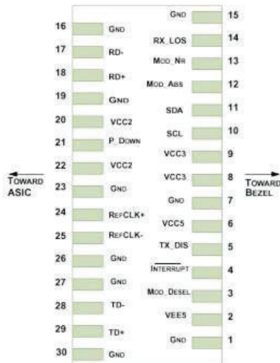
Pin-out of Connector Block on Host Board
