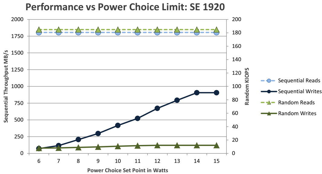
Figure 14. 1920GB Scalable Endurance: Performance vs Power Limit Settings IOPs chart
