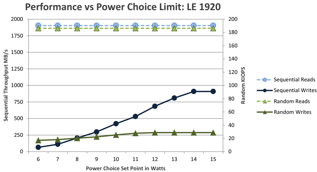
Figure 10. 1920GB Light Endurance: Performance vs Power Limit Settings IOPs chart
