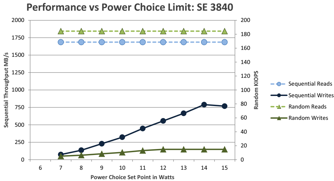
Figure 13. 3840GB Scalable Endurance: Performance vs Power Limit Settings IOPs chart
