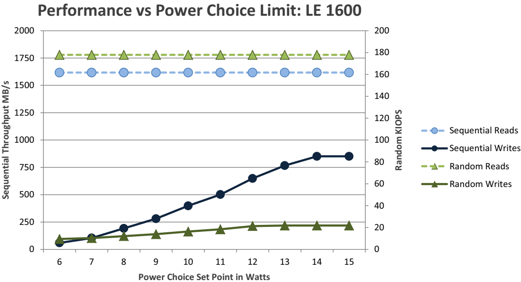
Figure 6. 1600GB Light Endurance: Performance vs Power Limit Settings IOPs chart
