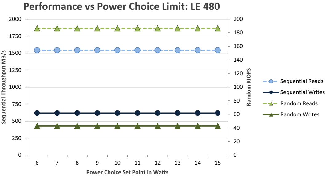
Figure 12. 480GB Light Endurance: Performance vs Power Limit Settings IOPs chart
