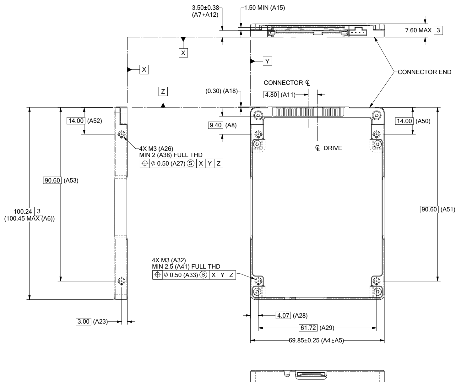
Figure 19. Mounting configuration dimensions (2.5" - 7mm models)
