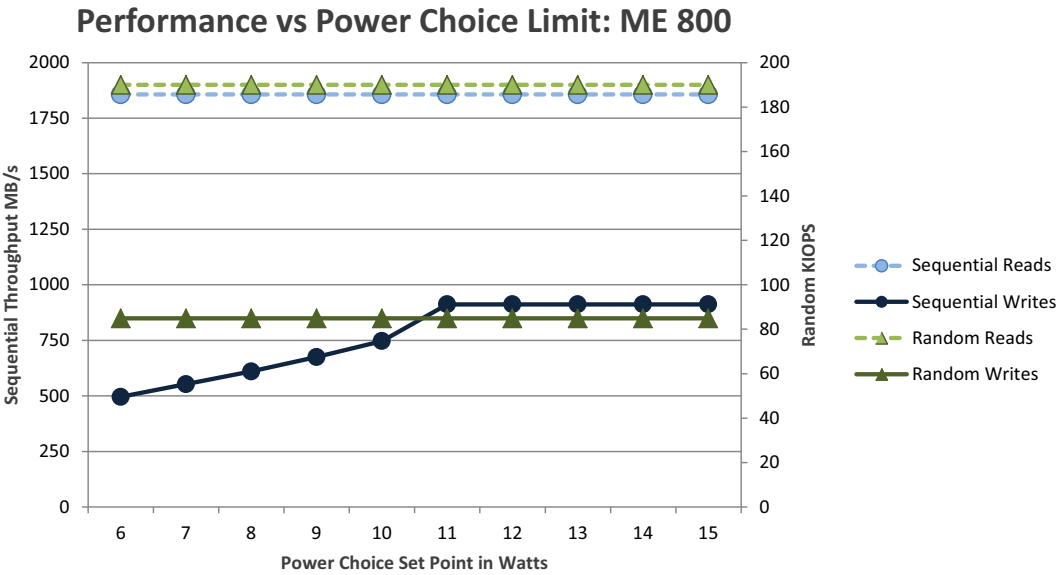
Figure 3. 800GB Mainstream Endurance: Performance vs Power Limit Settings IOPs chart
