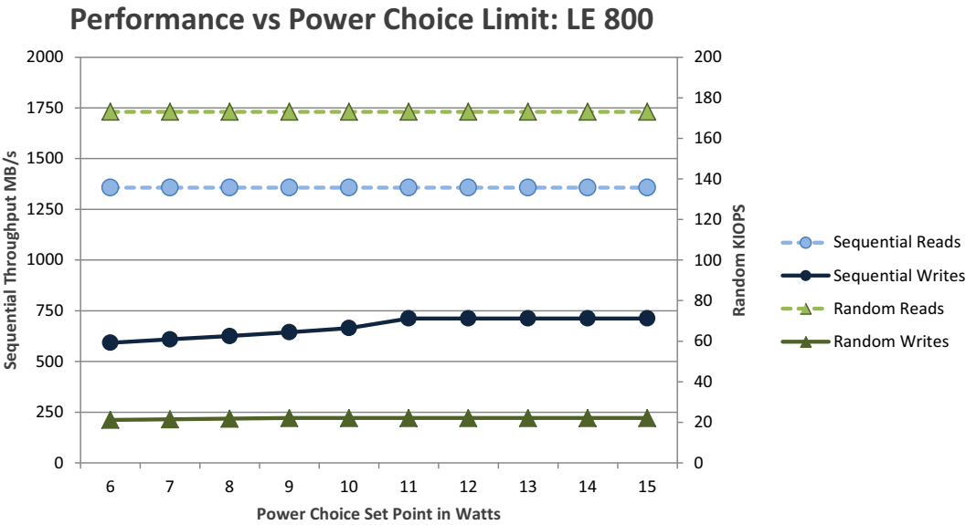
Figure 7. 800GB Light Endurance: Performance vs Power Limit Settings IOPs chart
