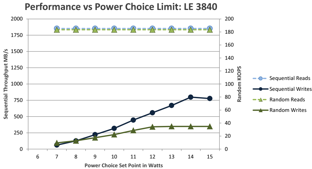
Figure 9. 3840GB Light Endurance: Performance vs Power Limit Settings IOPs chart
