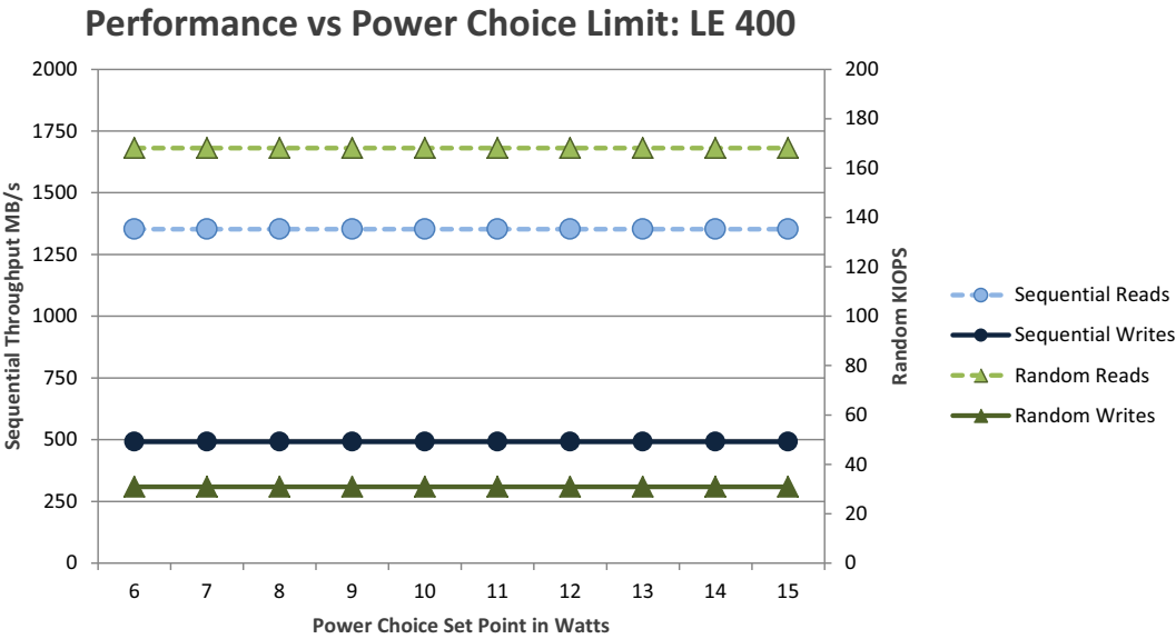
Figure 8. 400GB Light Endurance: Performance vs Power Limit Settings IOPs chart
