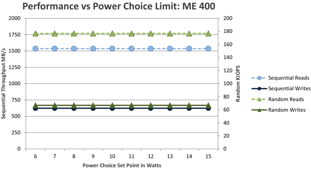
Figure 4. 400GB Mainstream Endurance: Performance vs Power Limit Settings IOPs chart
