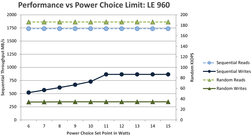
Figure 11. 960GB Light Endurance: Performance vs Power Limit Settings IOPs chart
