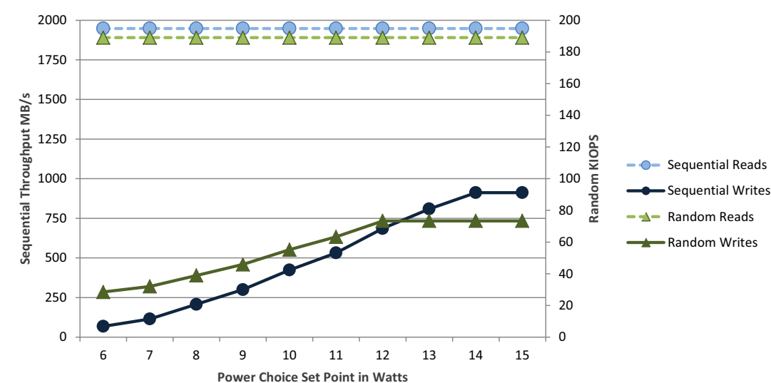
Performance vs Power Choice Limit: ME 1600
