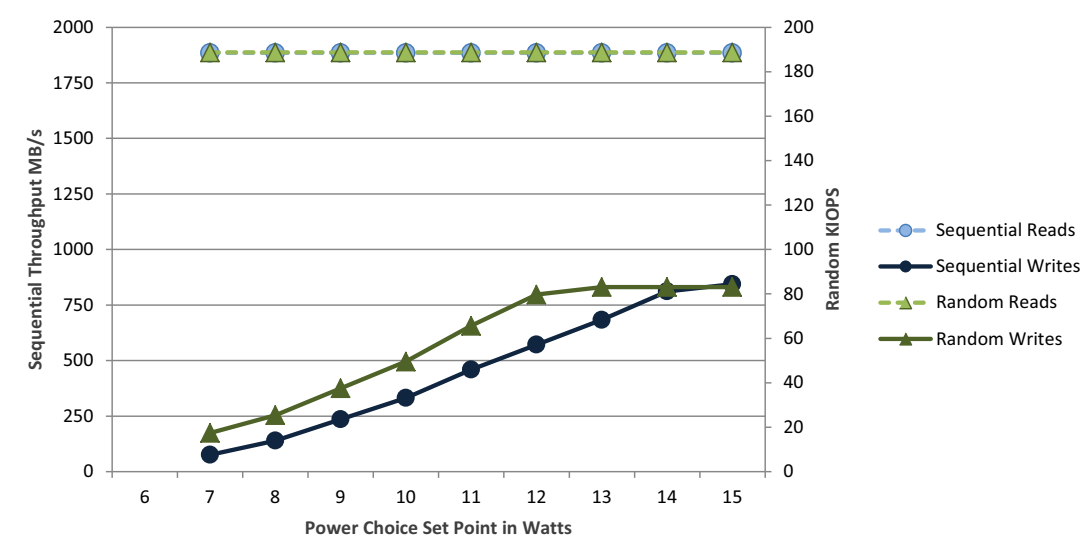
Performance vs Power Choice Limit: ME 3200
