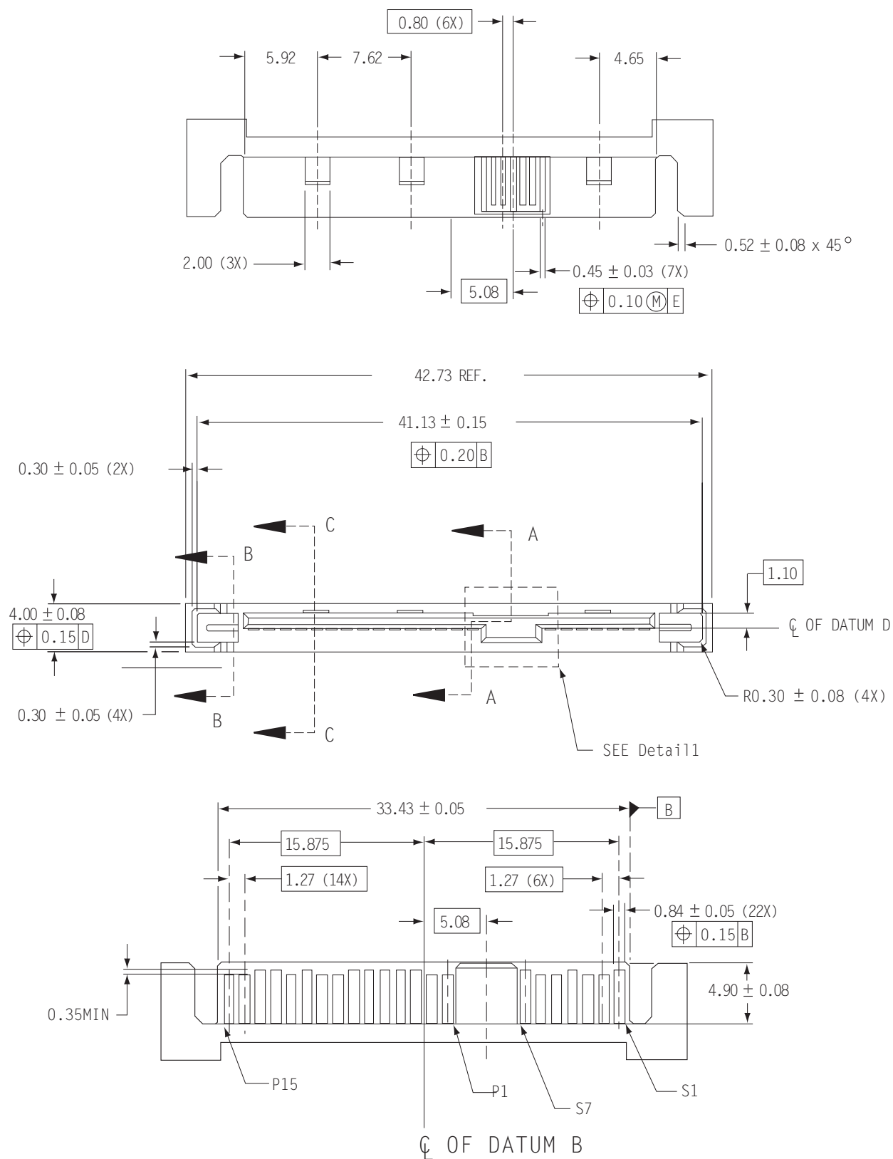
Figure 25. SAS device plug dimensions
