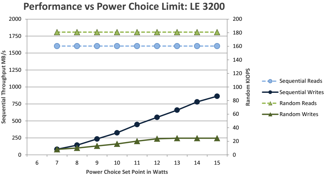
Figure 5. 3200GB Light Endurance: Performance vs Power Limit Settings IOPs chart
