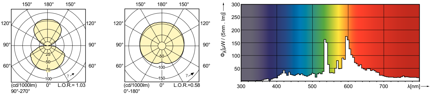
LDLD_CDM-TD_150W_830-Light distribution diagram
