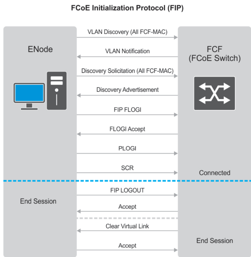
Figure 39. FIP Discovery and Login Between an ENode and an FCF
