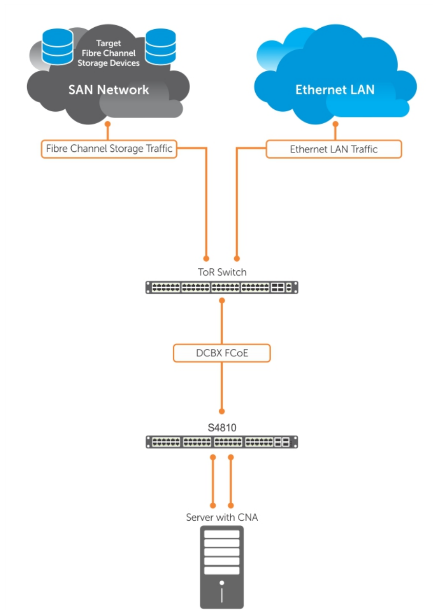
Figure 40. FIP Snooping on a Dell EMC Networking Switch
