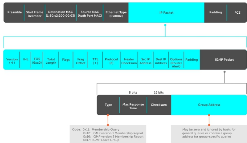
Figure 46. IGMP Messages in IP Packets
