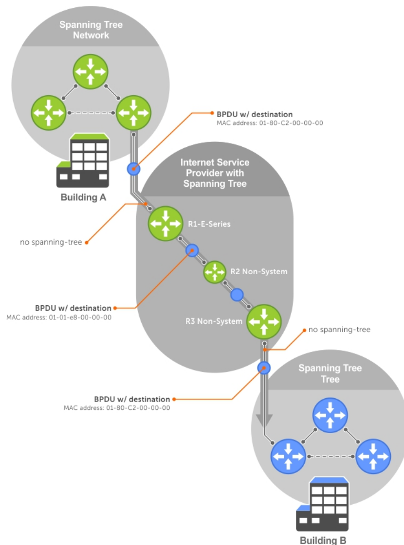
Figure 125. VLAN Stacking with L2PT
