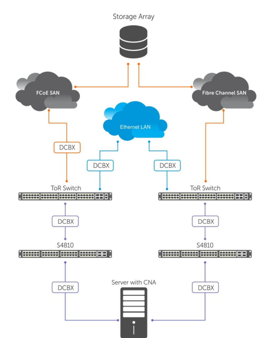
Figure 33. PFC and ETS Applied to LAN, IPC, and SAN Priority Traffic
