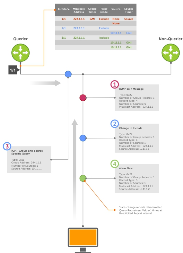
Figure 49. Membership Reports: Joining and Filtering
