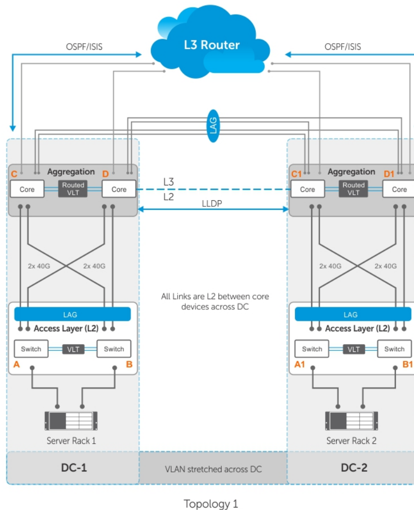
Figure 152. Sample Configuration for a VLT Proxy Gateway
