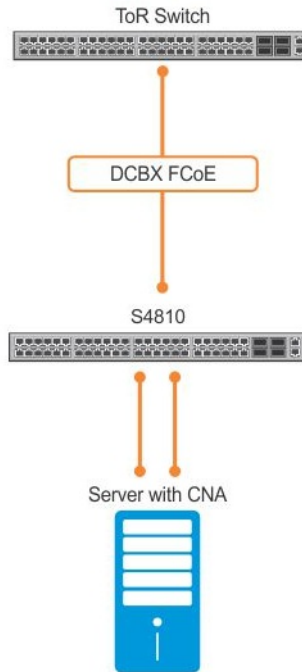
Figure 41. Configuration Example: FIP Snooping on a Switch
