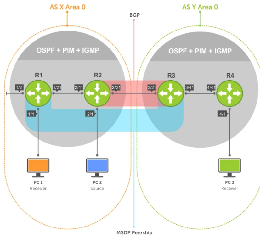
Figure 86. Multicast Source Discovery Protocol (MSDP)
