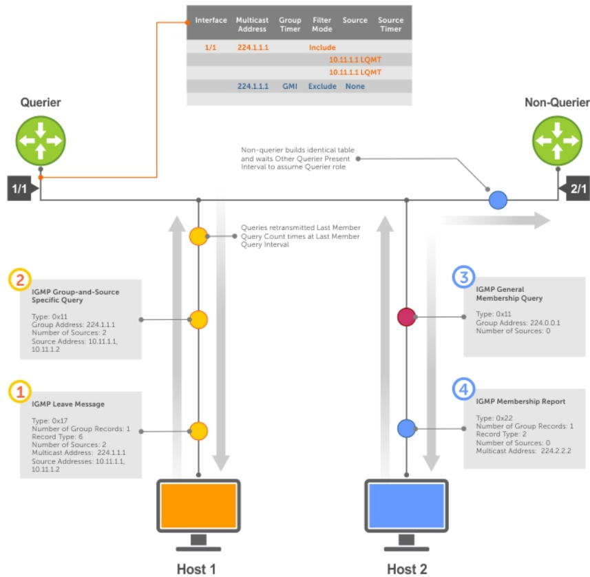
Figure 50. Membership Queries: Leaving and Staying
