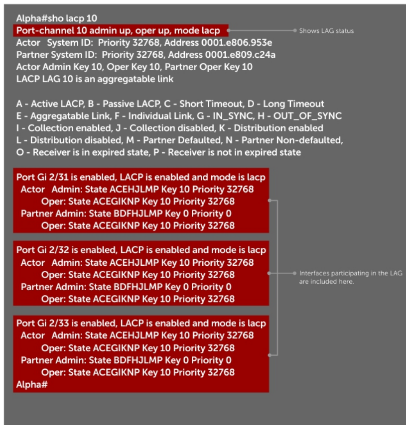
Figure 70. Verifying LAG 10 Status on ALPHA Using the show lacp Command
