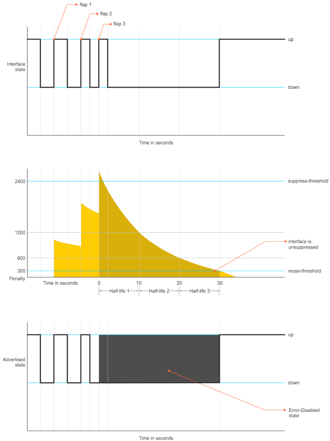
Figure 52. Interface State Change
