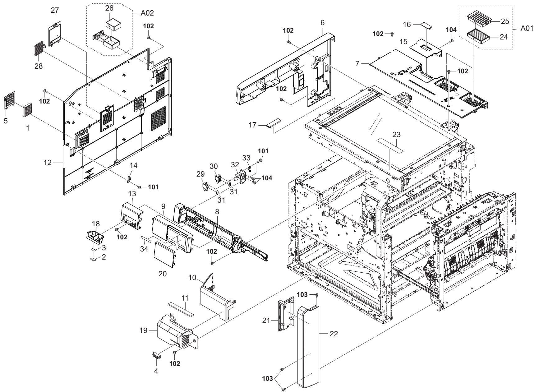
FIG. 2 Covers 2
