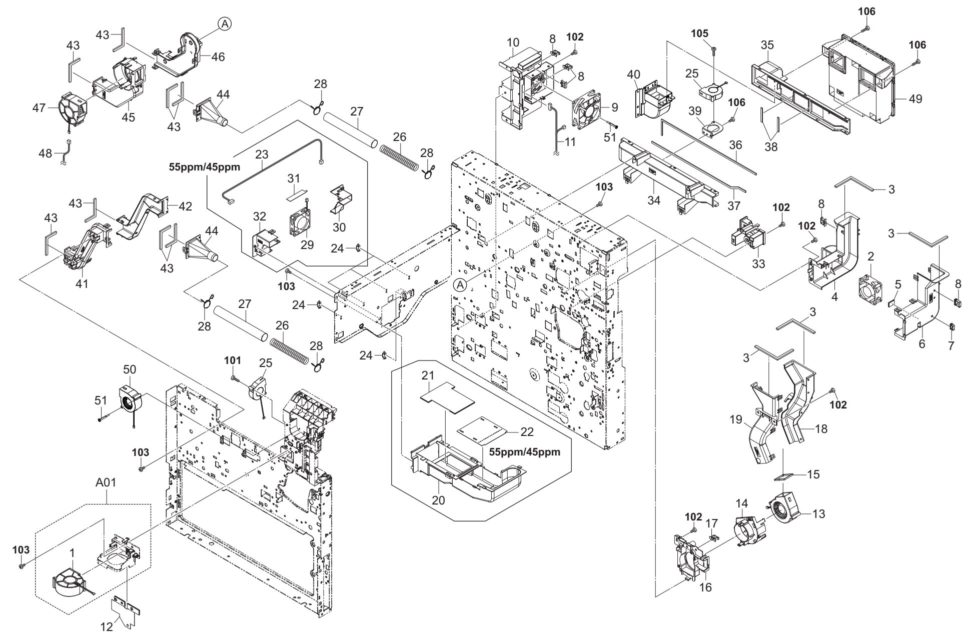
FIG. 18 Cooling Section
