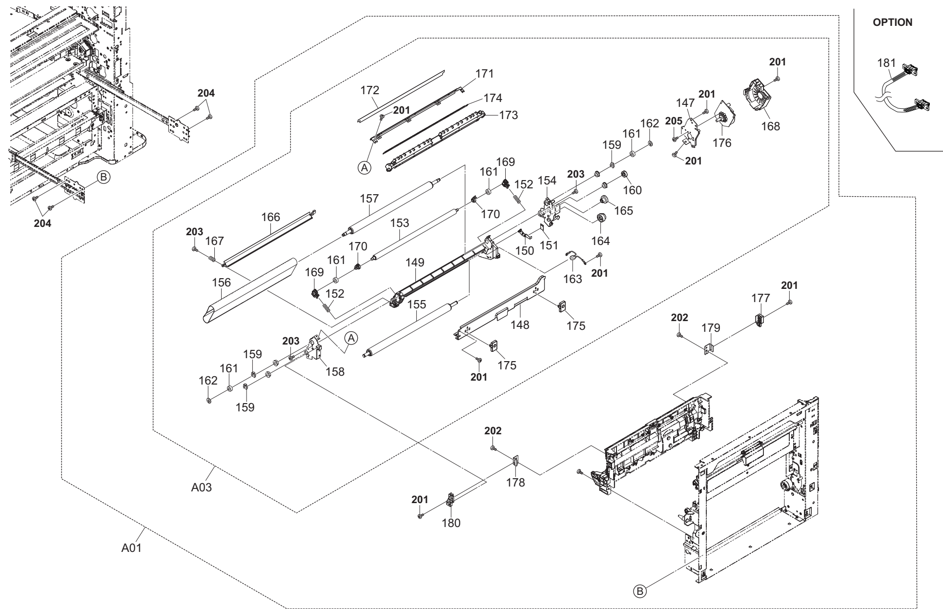
FIG. 8 Paper Conveying Section 1-3
