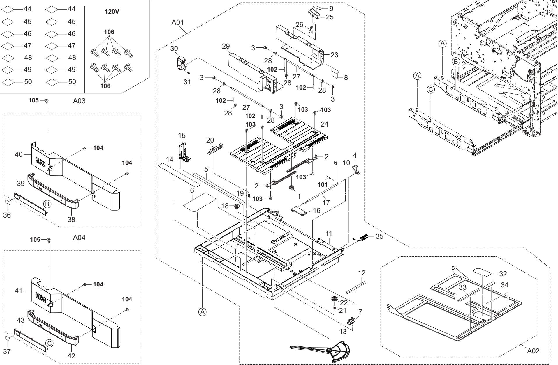
FIG. 5 Paper Cassettes
