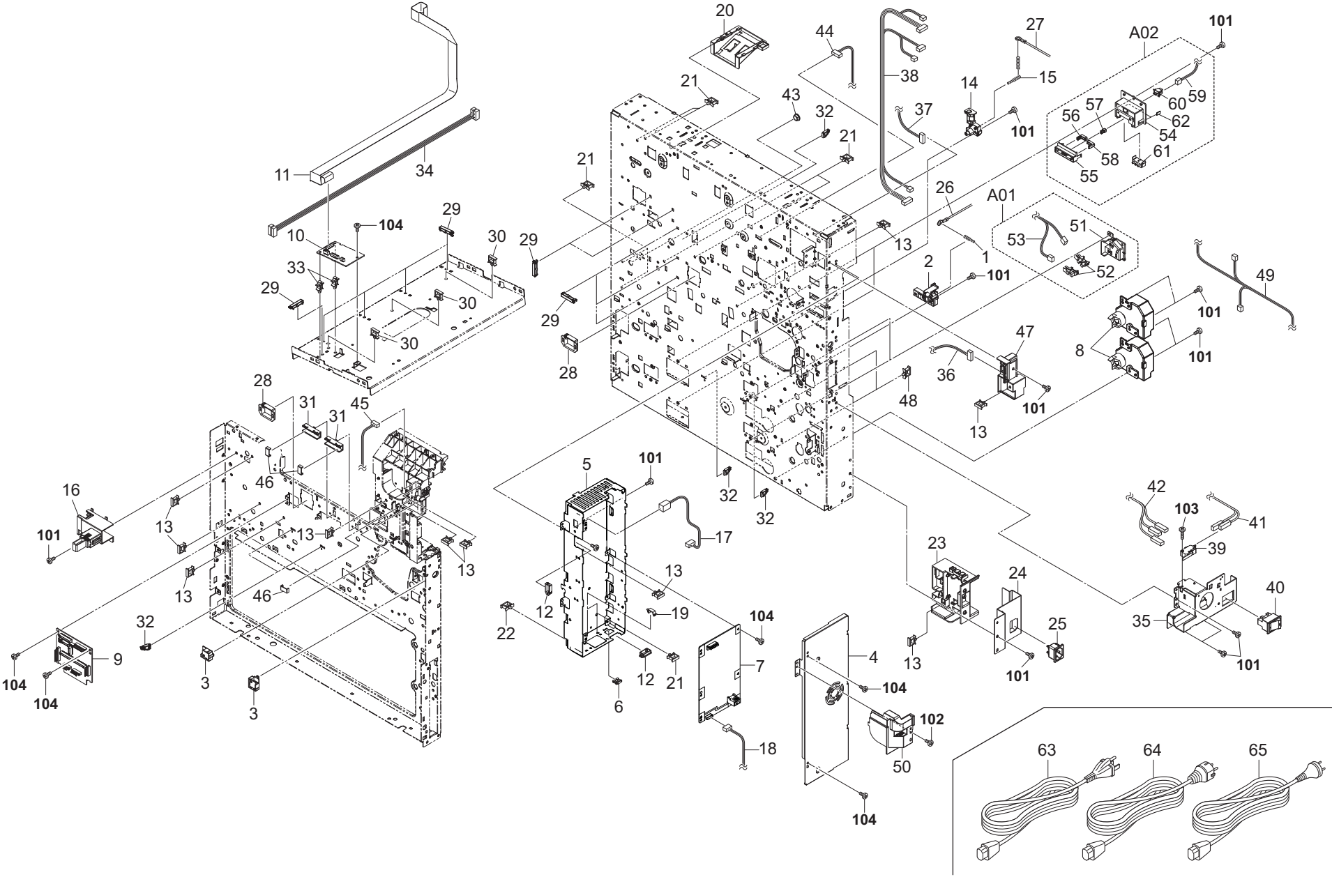
FIG. 20 Electrical Components 1
