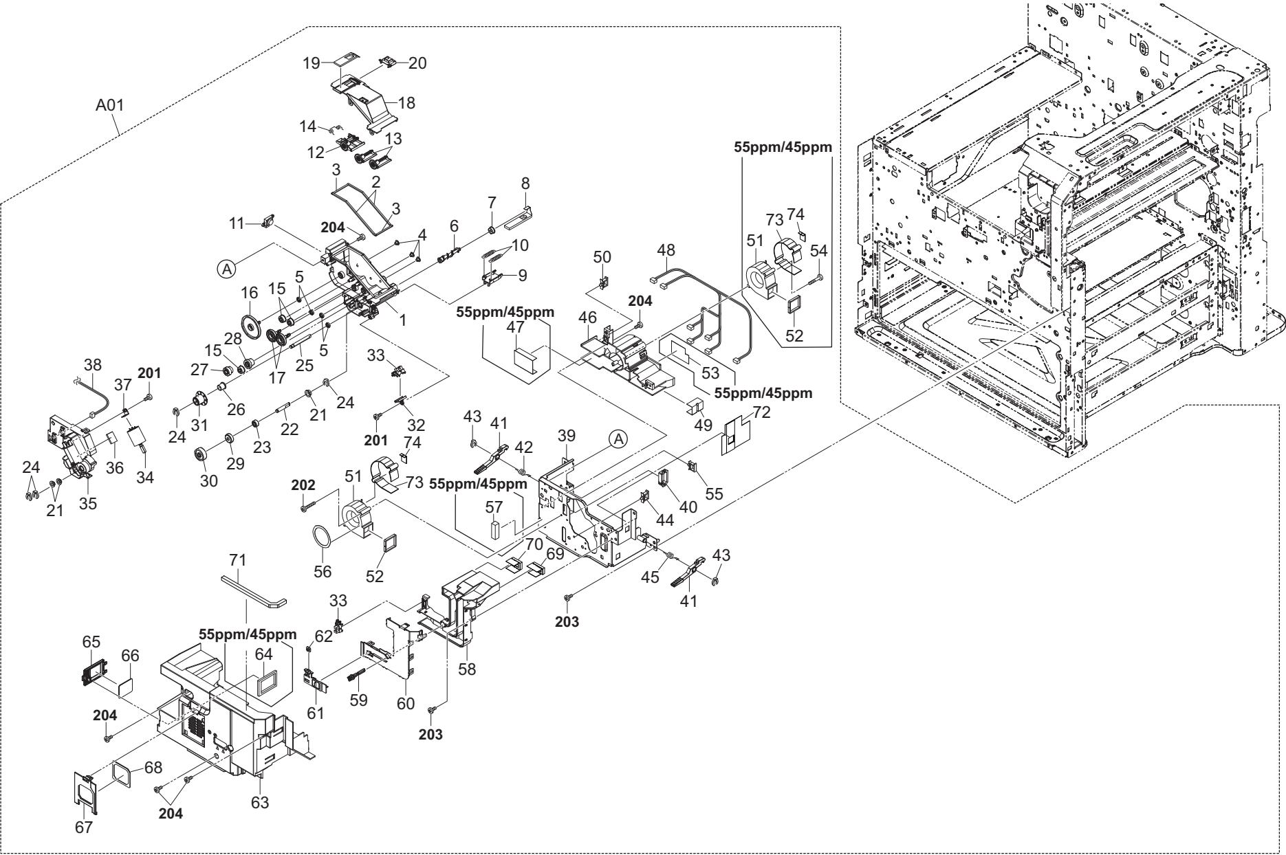
FIG. 13 Inner Section 1-1
