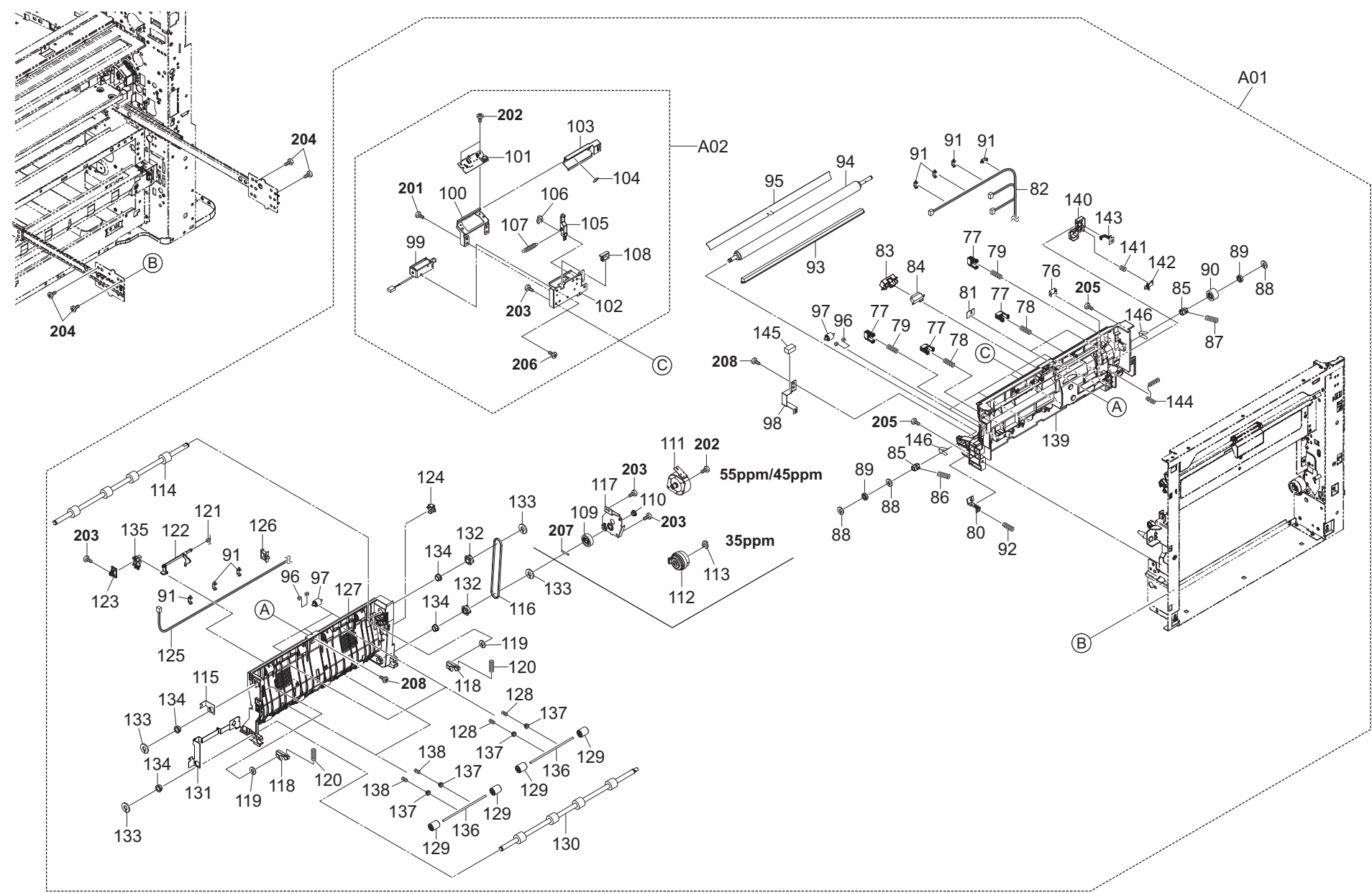
FIG. 8 Paper Conveying Section 1-2
