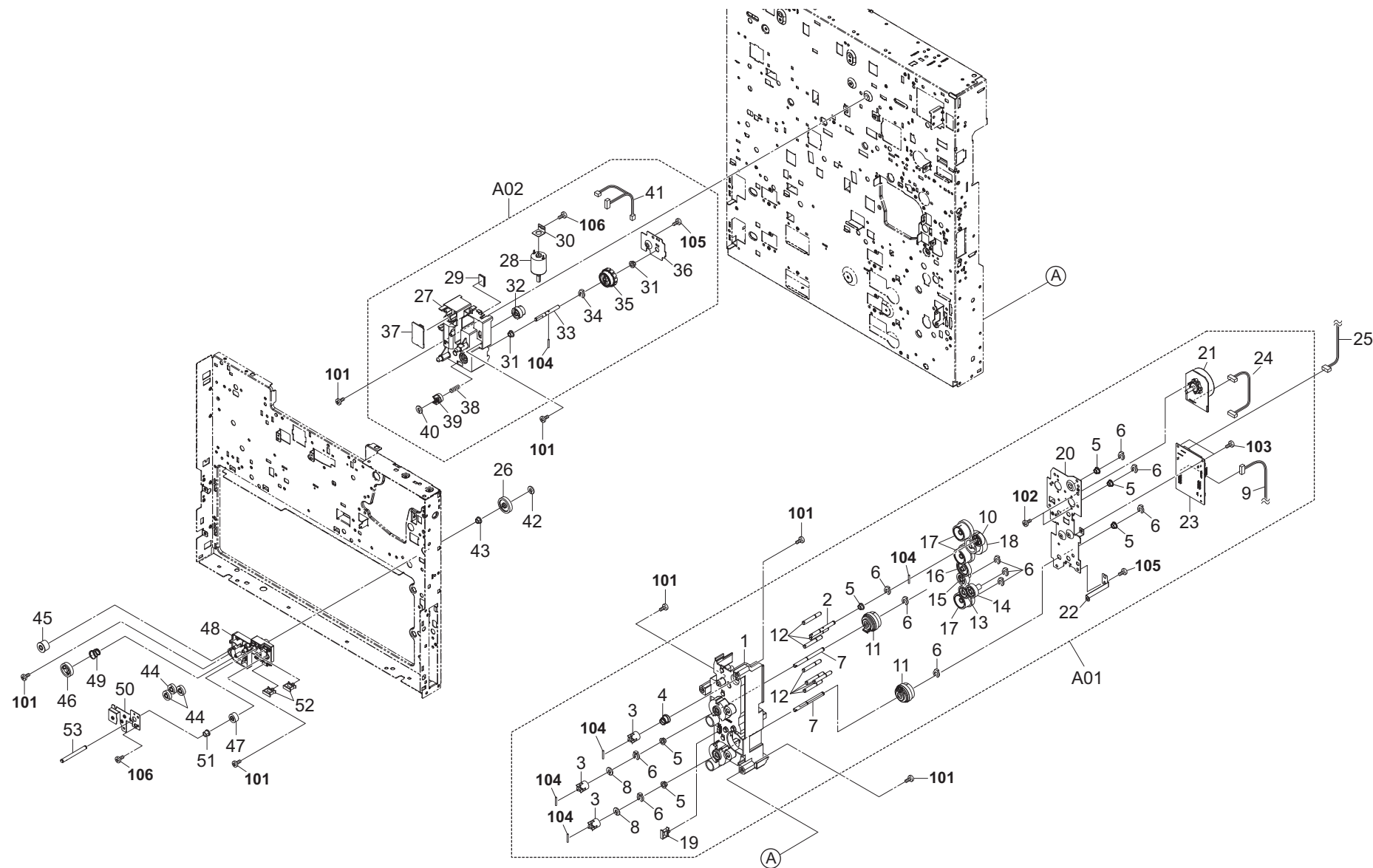
FIG. 17 Drive Section 2 (35ppm)
