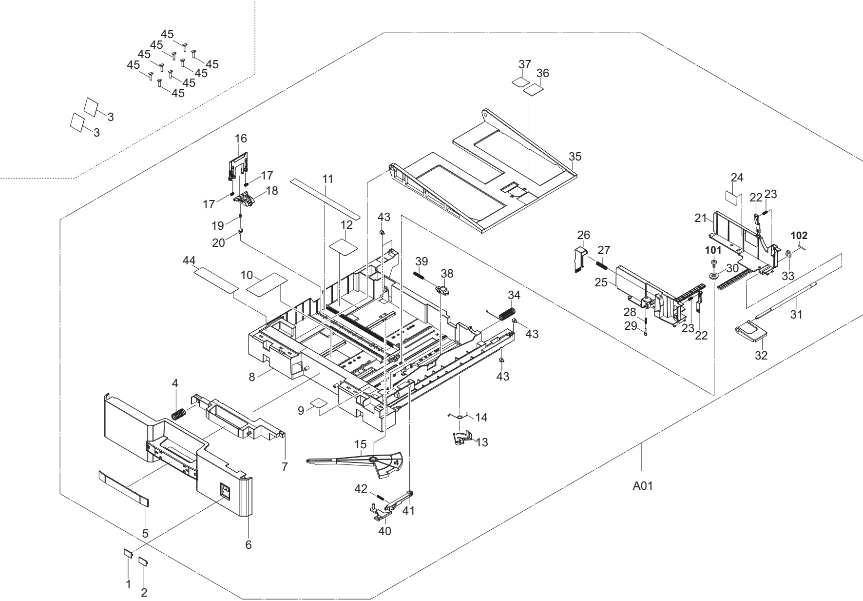
FIG. 8 Paper Cassette
