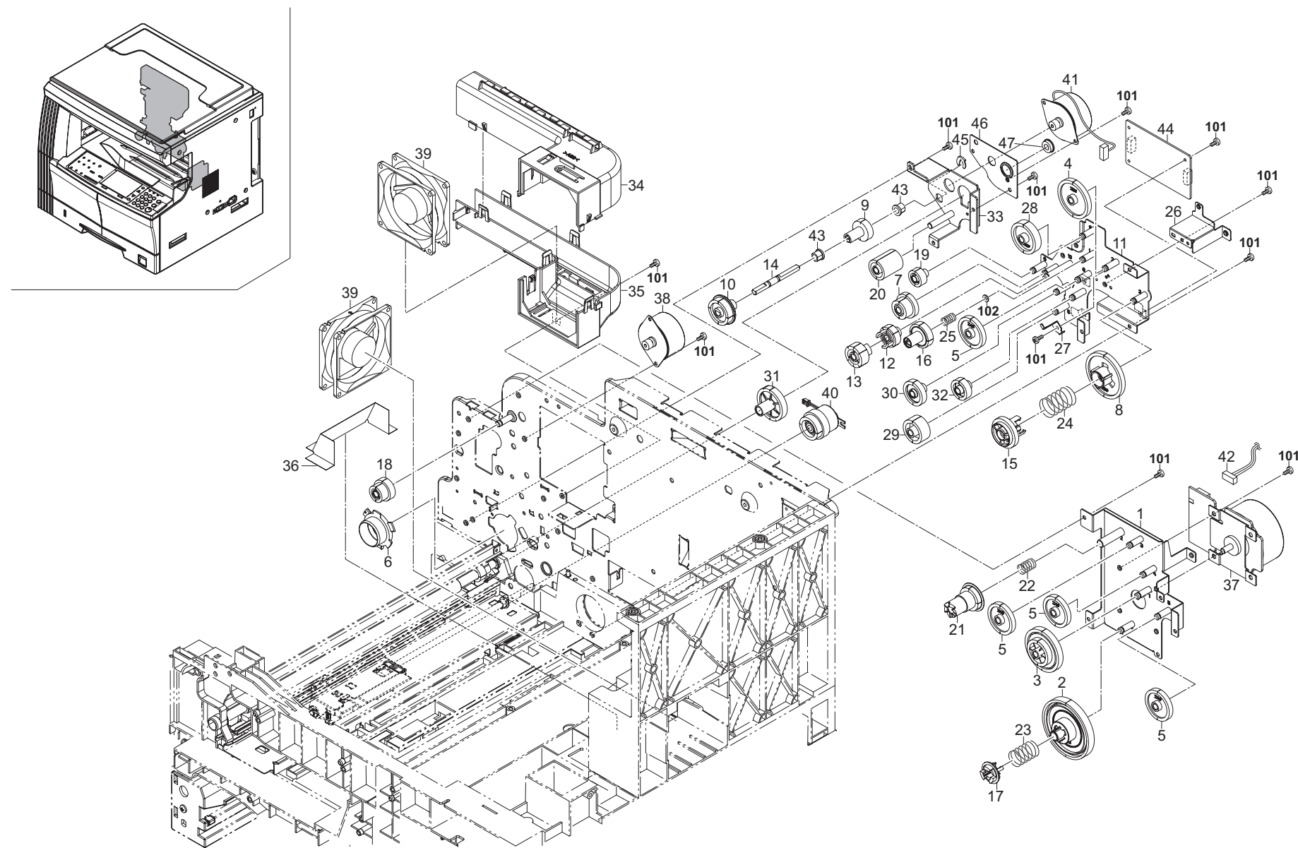
FIG. 11 Driving & Cooling
