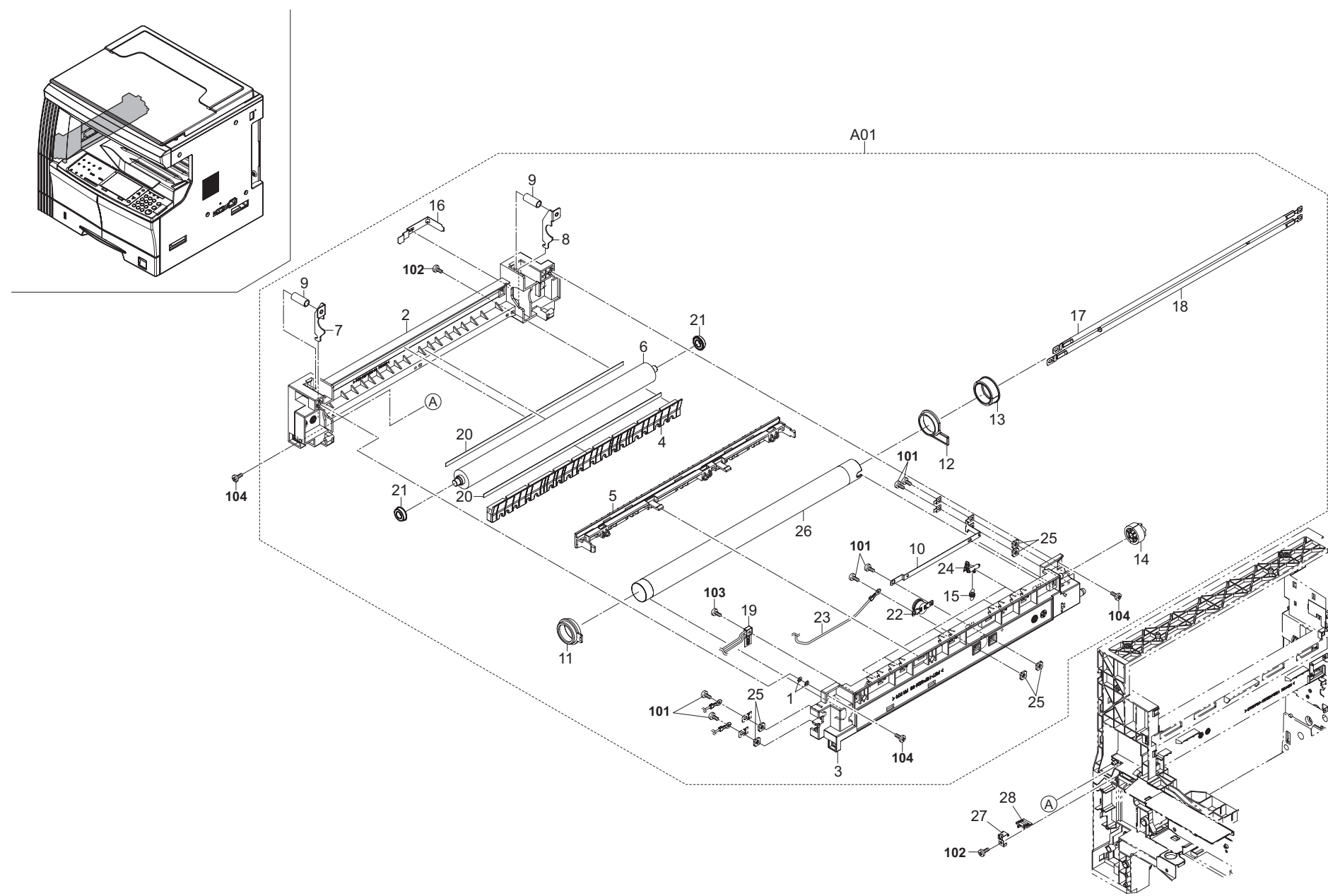
FIG. 10 Fuser Unit
