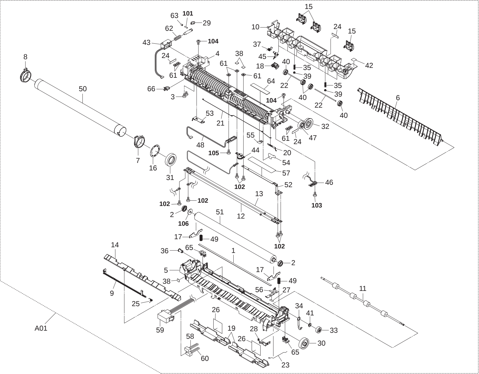
FIG. 11 Fuser Section 1
