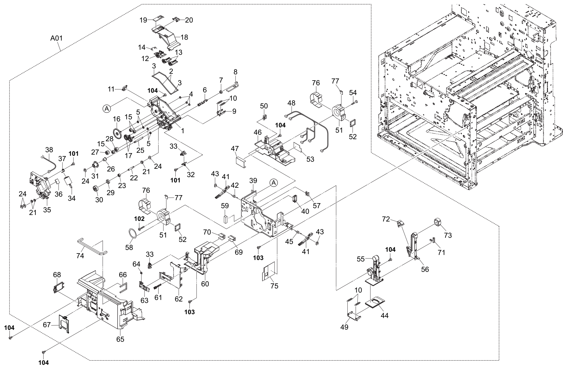
FIG. 21 Inner Section 1
