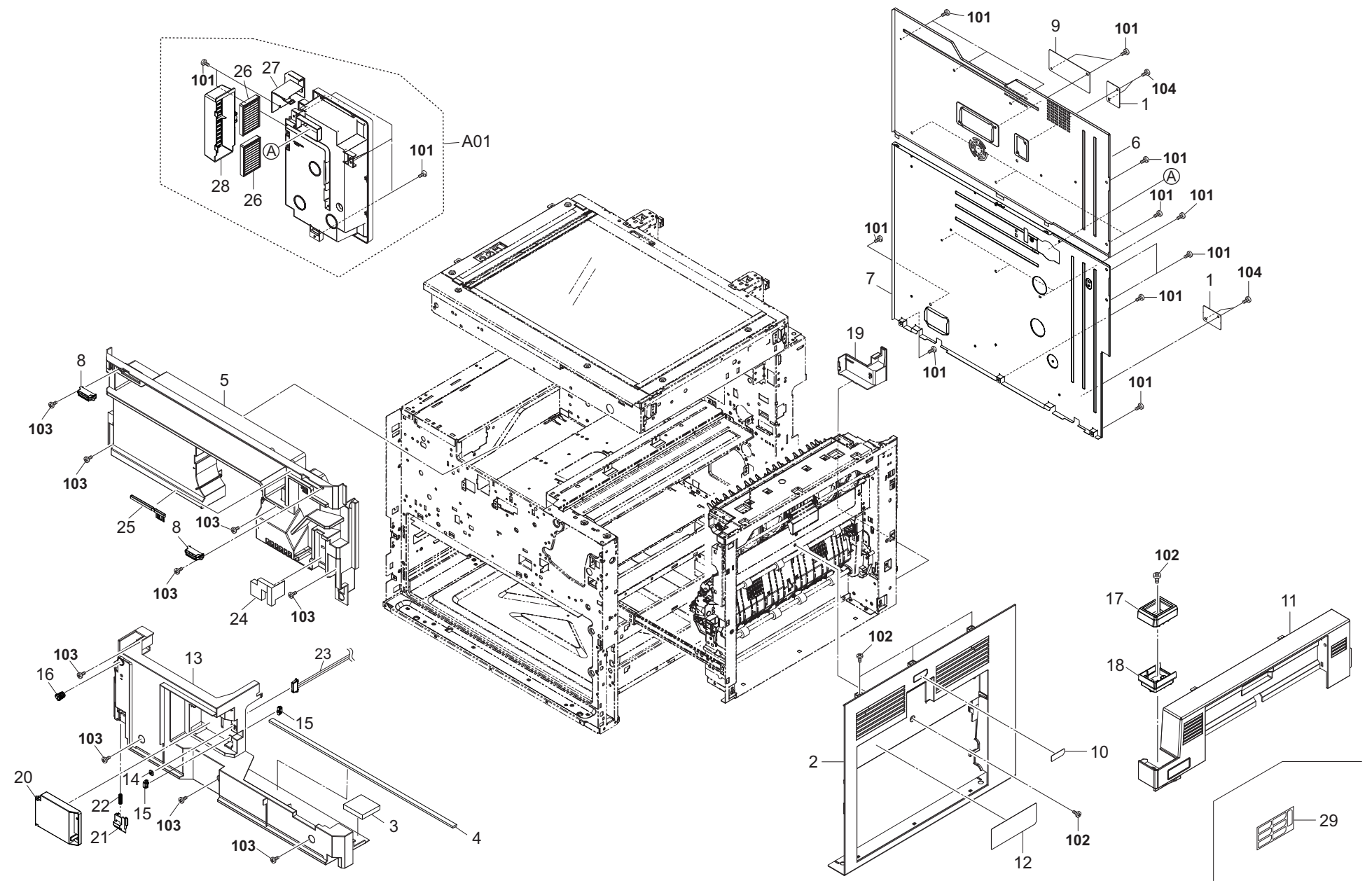
FIG. 3 Covers 3
