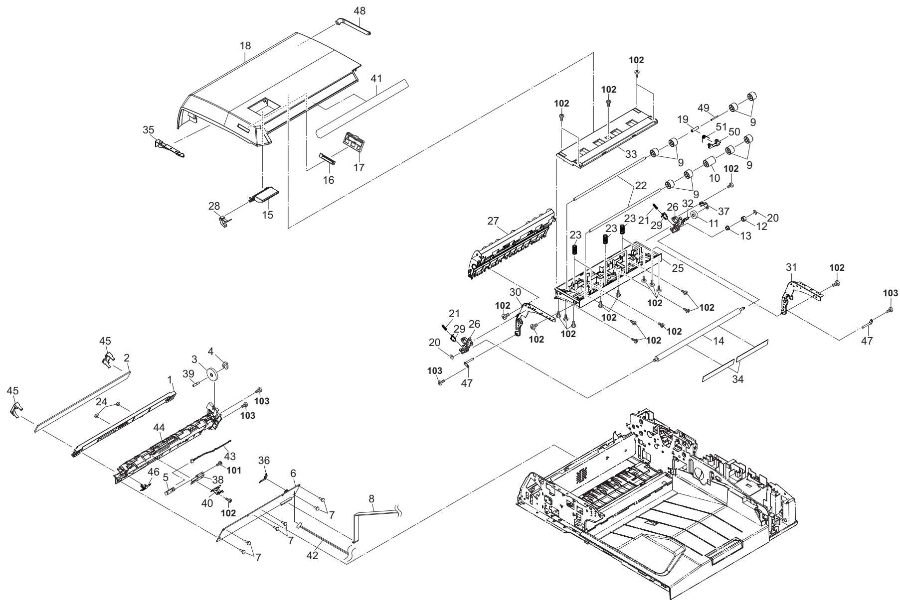
FIG. 40 Paper Feed Section 1(DP)
