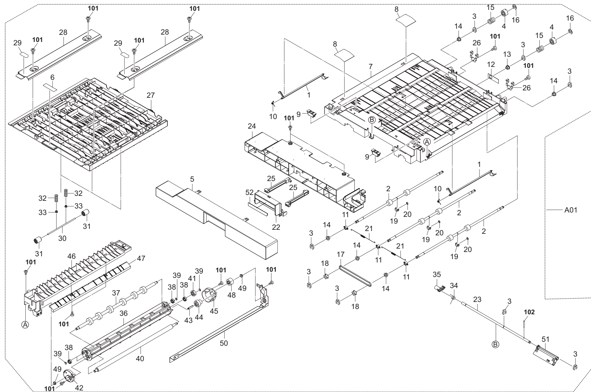
FIG. 29 Bridge Section 1
