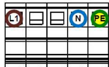
HARDWIRED TERMINAL DETAIL (32 A, 1/N/PE, 200-240 V)
