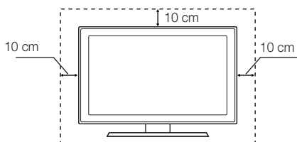
Paigaldamine alusega
