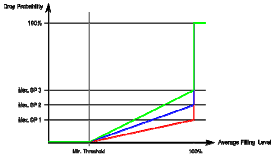
RED Drop Probability Function
