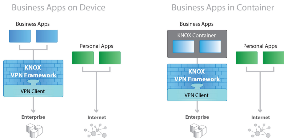
Figure 5 – Per Application VPN in KNOX
