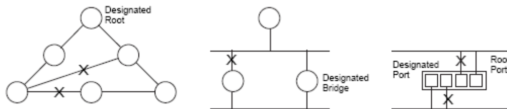
Figure 45: STP Root Ports and Designated Ports
