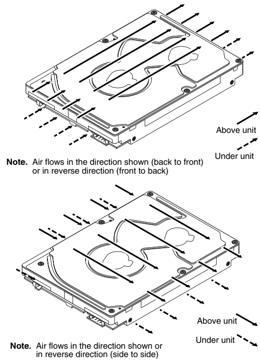
Figure 12. Air flow
