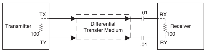
Figure 17. SAS transmitters and receivers
