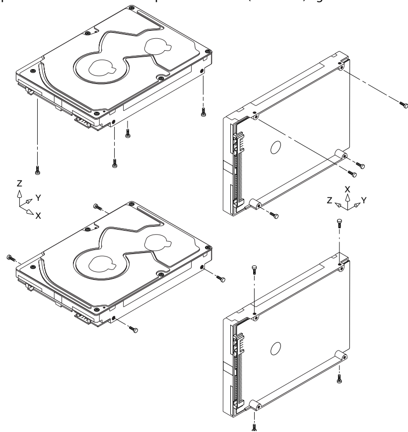
Figure 8. Recommended mounting
