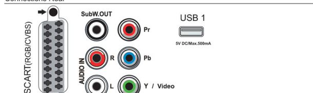
Connections Rear
