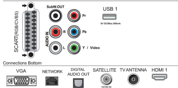
Connections Rear
