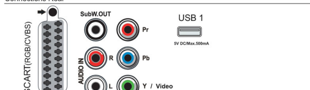
Connections Rear
