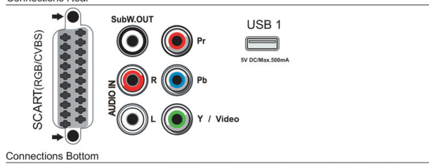
Connections Rear
